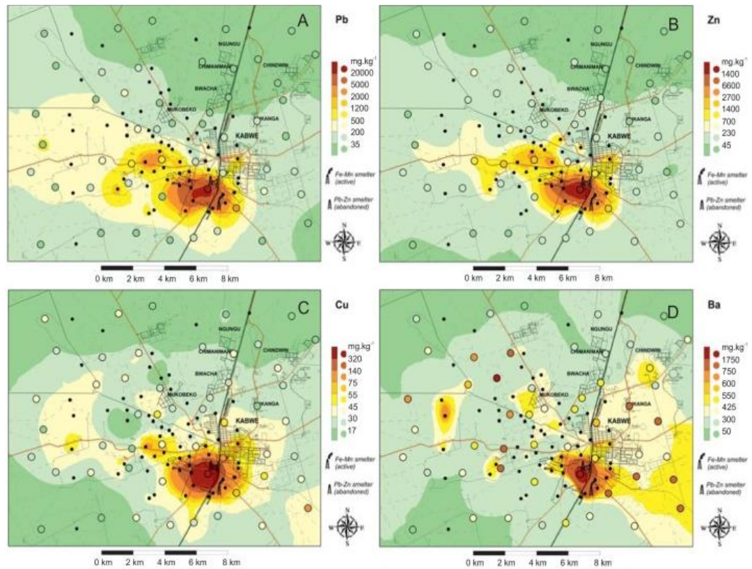
Figure 1. Contour maps of the Pb (A), Zn (B), Cu (C) and Ba (D), contents (in mg/kg) in topsoil (0-3 cm depth) and classed point maps of the same elements in subsurface soils (70-80 cm depth) in the Kabwe area, Zambia (Křibek et al., 2019).
