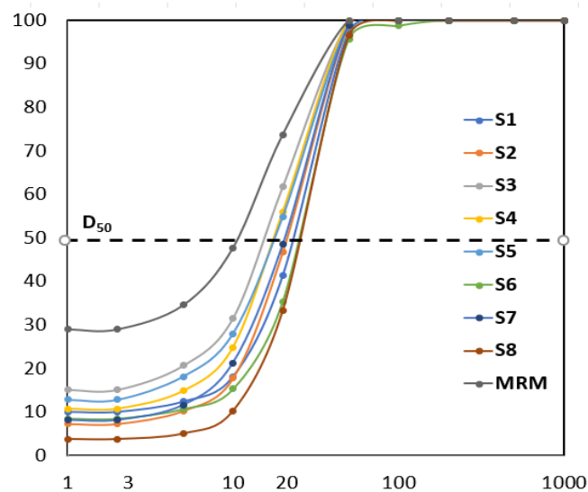
Figure 11. Particle size distribution in ( < 30\ \mu\text{m} ) with their 50% effective diameter
