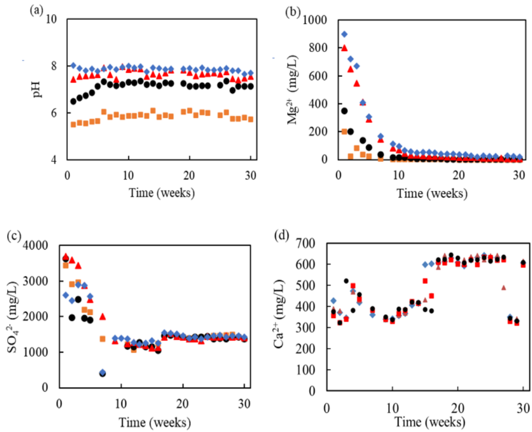
Figure 17. Changes in pH, \text{Mg}^{2+} , \text{SO}_4^{2-} , and \text{Ca}^{2+} concentrations over time: pH vs time (a), \text{Mg}^{2+} vs time (b), \text{SO}_4^{2-} concentration vs time (c), and \text{Ca}^{2+} concentration vs time (d) (case HBD 0 (■), case HBD 1 (●), case HBD 5 (▲), and case HBD 10 (◆))
