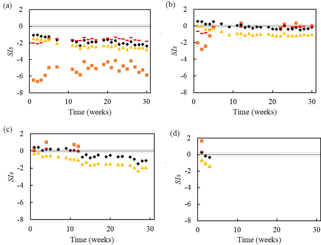
Figure 22. Saturation indices of cerussite (■), smithsonite (▲), hydrocerussite (■), and hydrozincite (◆) in the effluents of cases HBD 0 (a), HBD 1 (b), HBD 5 (c), and HBDD 10 (d)
