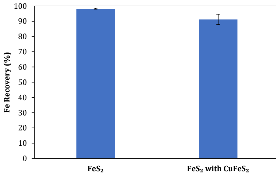
Fig. 4-4. Pyrite recovered (%) without (left) and with (right) chalcopyrite fine particles present, Test conditions: [KAX] = 500 g/t; [MIBC] = 25 \mu\text{L/L} ; [particle size] = -125+106 \mu\text{m} ; [ \text{FeS}_2 amount] = 10 g; [ \text{CuFeS}_2 amount] = 20 g.
