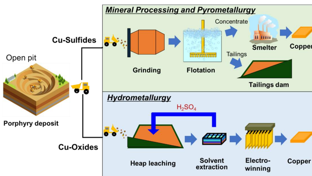
Fig. 1-1. Main processes for extracting copper from sulfide and oxide ores.
