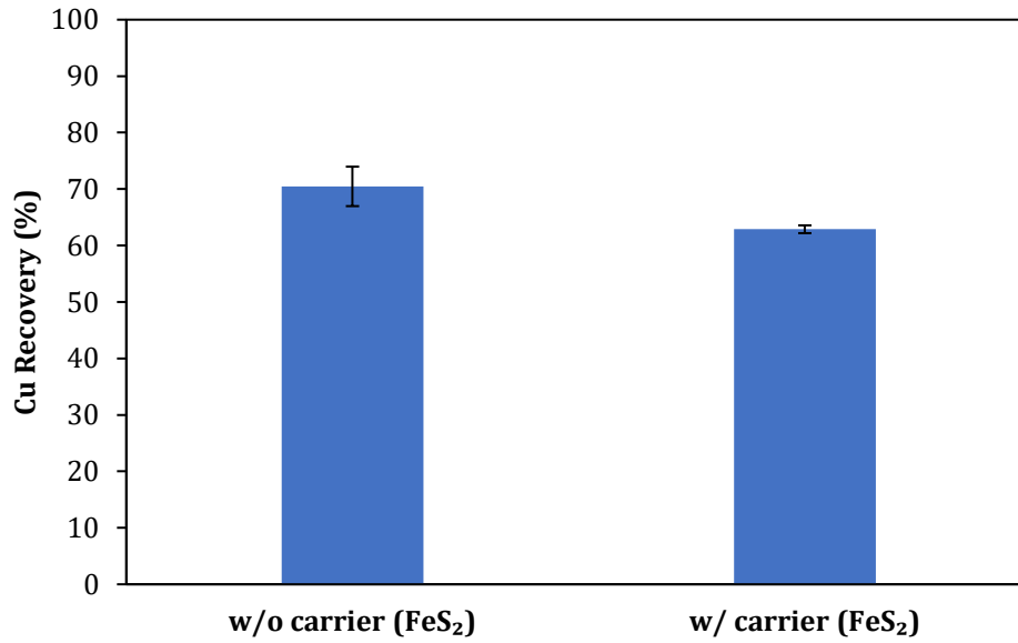
Fig. 4-3. Cu Recovery (%) from fines without (left) and with (right) pyrite as a carrier, Test conditions: [KAX] = 500 g/t; [MIBC] = 25 \mu\text{L/L} ; [Carrier size] = -125+106 \mu\text{m} ; [Carrier amount] = 10 g. KAX = potassium amyl xanthate; MIBC = methyl isobutyl carbinol.
