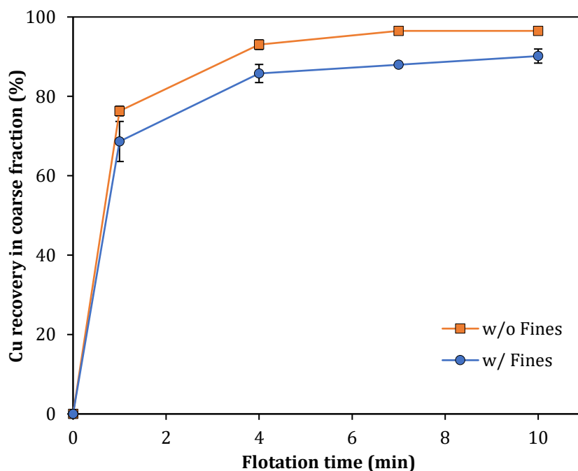
Fig. 3-10. Effect of fines on recovery of coarse particles, Test conditions: [KAX] = 200 g/t of fines; [MIBC] = 25 \mu\text{L/L} ; [Carrier Size] = -106+75 \mu\text{m} .
