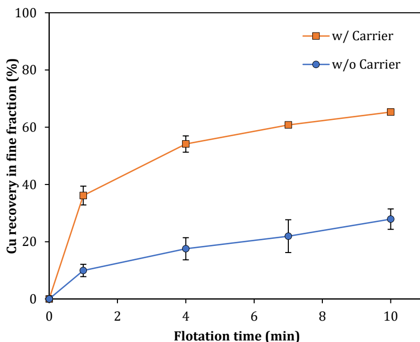
Fig. 3-9. Cu Recovery% of fines, Test conditions: [KAX] = 200 g/t of fines; [MIBC] = 25 \mu\text{L/L} ; [Carrier size] = -106+75 \mu\text{m} ; [Carrier amount] = 10 g.
