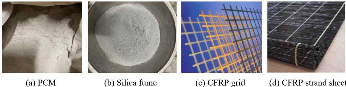
Figure 5-1 Overlaying material used in this experimental work
