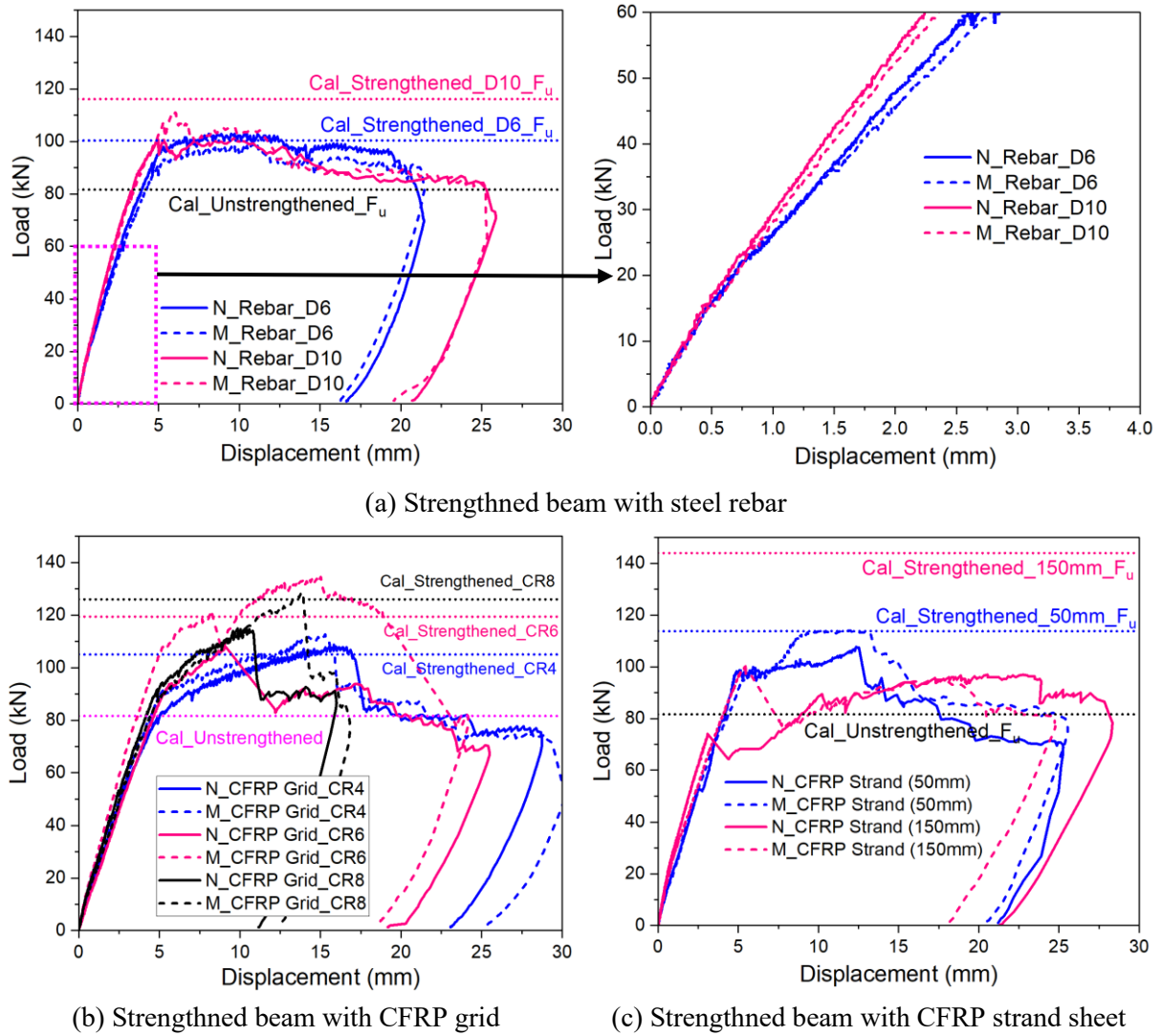
Figure 5-6 Comparison of load-displacement diagram and ultimate displacement of all the strengthened RC beam
