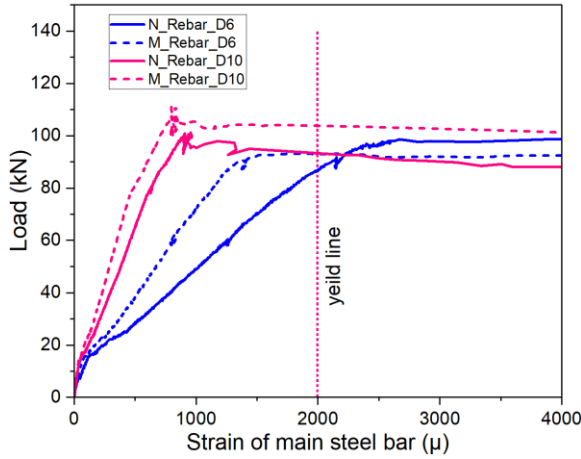
(a) Steel rebar as strengthening reinforcement
