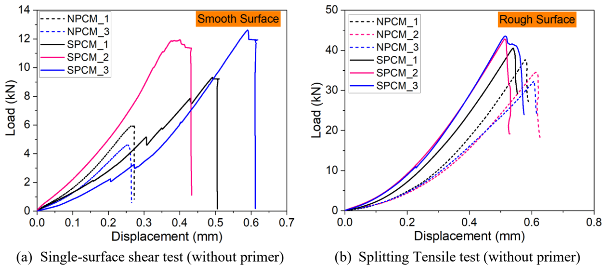
Figure 2-10 Load-displacement relationship of the normal and modified 5% silica PCM specimens
