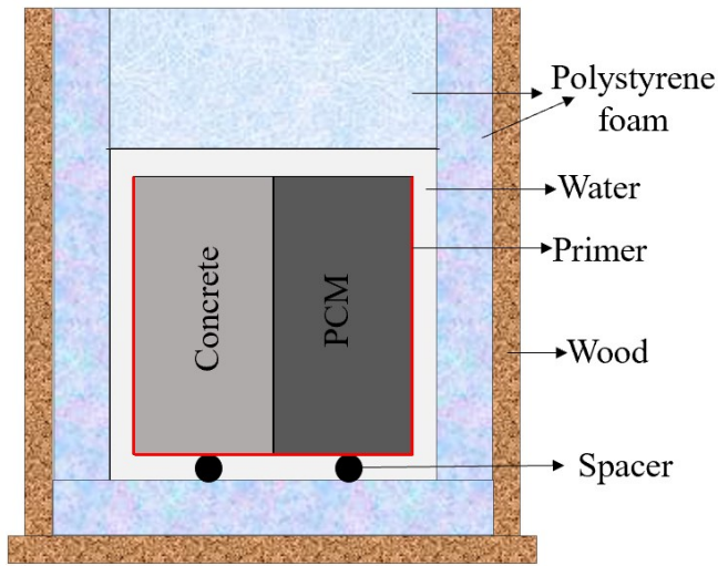
(a) Self-designed freeze thaw environment
