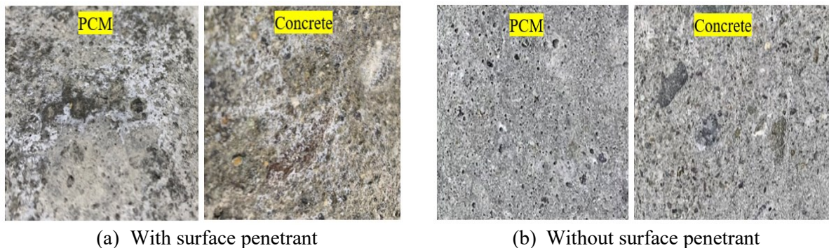
Figure 3-7 White compound in the interface
