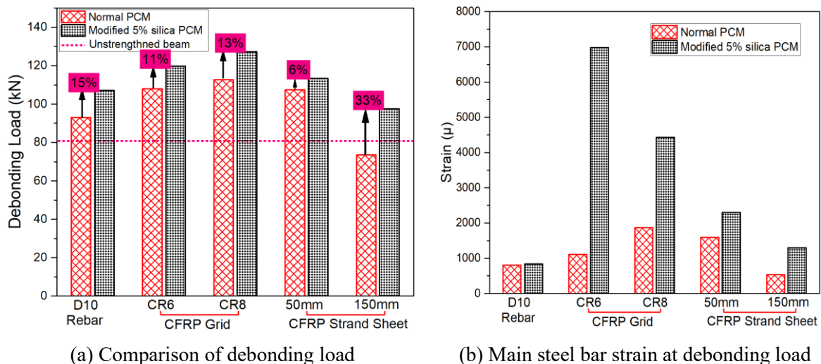
Figure 5-9 Influence of silica fume to delay the occurrence of debonding
