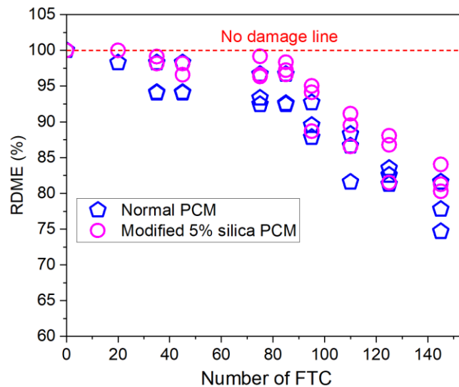
Figure 4-8 RDME of composite specimens under FTC (Type A specimens)
