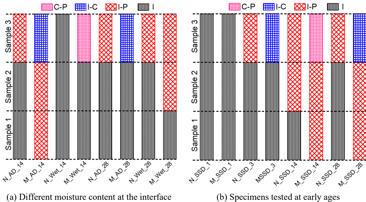
Figure 3-14 Fracture mode of all the composite specimens of Series -II and Series-III
