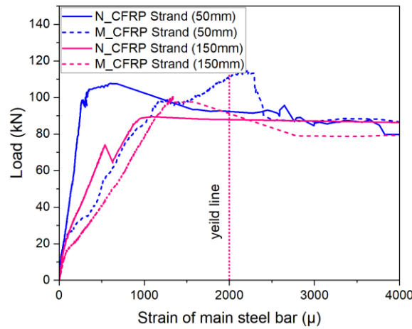
(c) CFRP strand sheet as strengthening reinforcement
