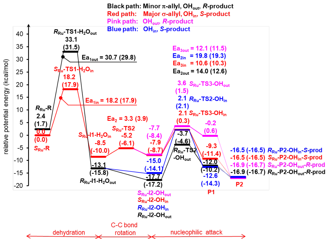
Figure 4. Potential energy profiles for ( R )-Cl-Naph-PyCOOH-CpRu catalyzed intramolecular O-allylation via major \sigma -allyl mechanism (red), minor \pi -allyl mechanism (black) and possible routes OH out , R -product (pink) with OH in , S -product (blue). Gibbs free energies (298.15 K) are shown in parenthesis.
