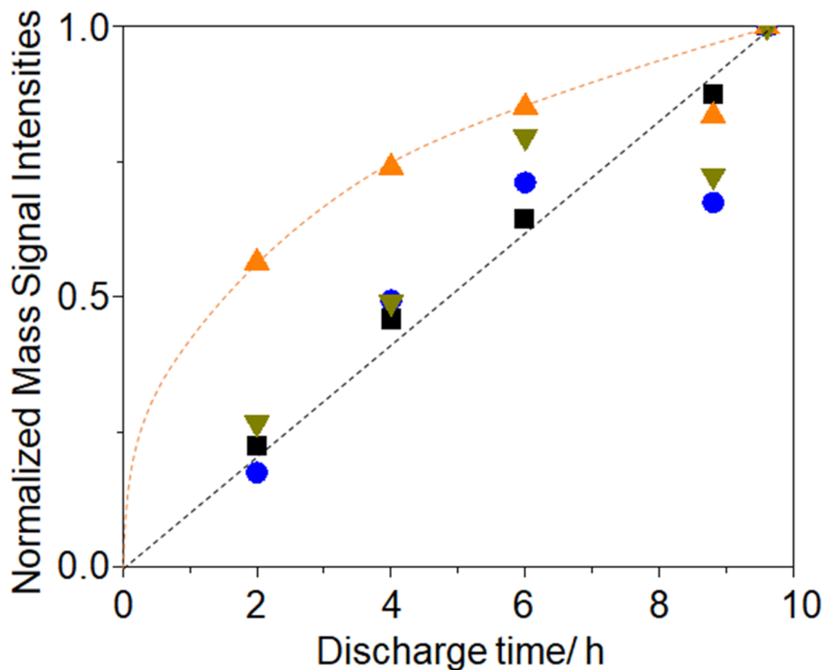
Figure 3-7. Discharge time dependencies of integrated signal intensities, i.e., current (▼), and ion current of 18 (▲), 32 (●), and 44 (■), normalized by those of 9.6 hr discharge.
