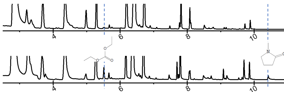
Figure 5-16. Gas chromatograms of head space gas sampled by CTPC-GC/MS of the cells prepared using 1 M LiTFSI (top panel) and 0.5 M LiTFSI and 0.5 M LiNO 3 dissolved in TEGDME (HG) (bottom panel).
