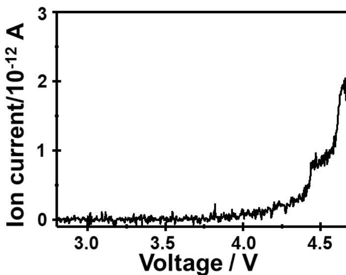
Figure 4-47. Ion current of molecules Methane ( \text{CH}_4 ) as a function of voltage.
