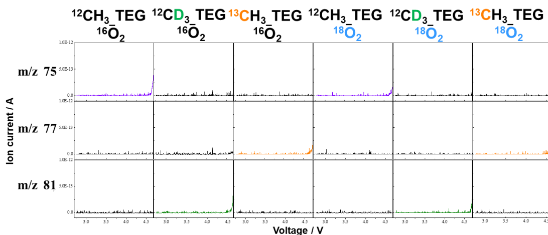
Figure 4-16. On-line QMS of m/z = 75/77/81 in isotope experiments.
