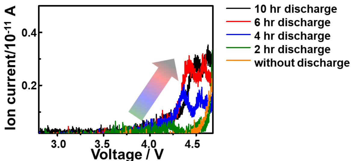
Figure 4-37. Mass signals of m/z = 31 with different discharge time, as a function of voltage.
