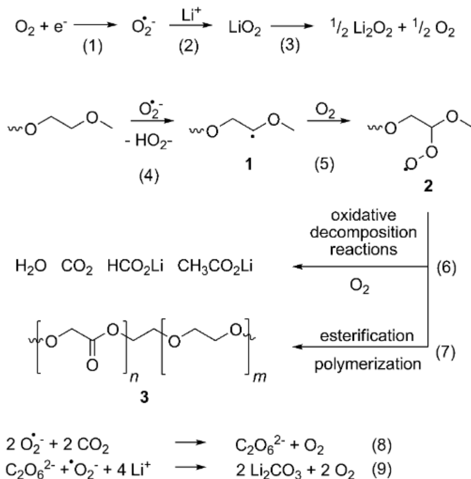
Scheme 1-2. Proposed mechanism for reactions that occur during dis-charge. 68
