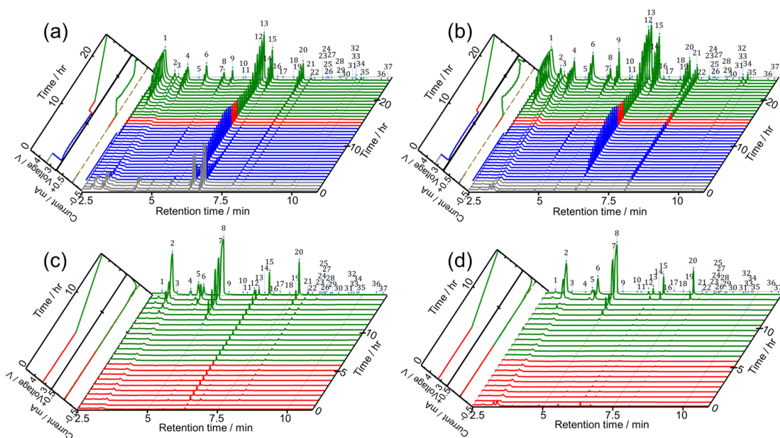
Figure 5-1. Gas chromatograms of head space gas sampled by CTPC-GC/MS every 40 min ( a, b ) during OCP (2 hr: gray), constant-current discharge (0.4 mA, 10 hr: blue), OCP (ca. 2.82 V, 2 hr: red), and charge by voltage sweep ( 0.05 \text{ mV s}^{-1} from OCP ( \sim 2.82 \text{ V} ) to 4.7 V: green) of the cells prepared using ( a ) BG- and ( b ) HP-TEGDME and ( c, d ) OCP (3.27 V to 3.25 V, 6 hr: red lines) and voltage sweep ( 0.05 \text{ mV s}^{-1} from 3.2 V to 4.7 V: green lines) without discharge of the cells prepared using HP-TEGDME filled with ( c ) Ar and ( d ) O 2 . Left panel: voltage and current as a function of time. Color coding is as of gas chromatograms.
