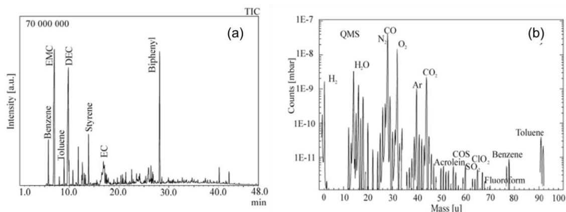
Figure 1-17. (a) Results of the gas chromatography-mass spectrometry (GC-MS) analysis. (b) the quadrupole mass spectrometry (QMS) analysis. 110
