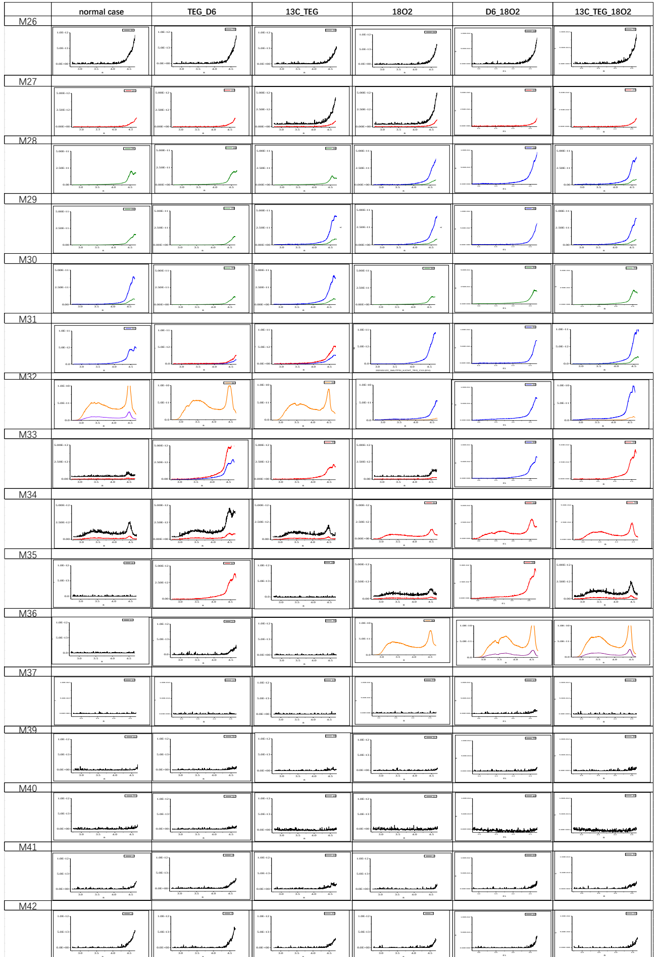
Isotope experiments mass behavior of m/z = 26\sim 42 . Table 2
