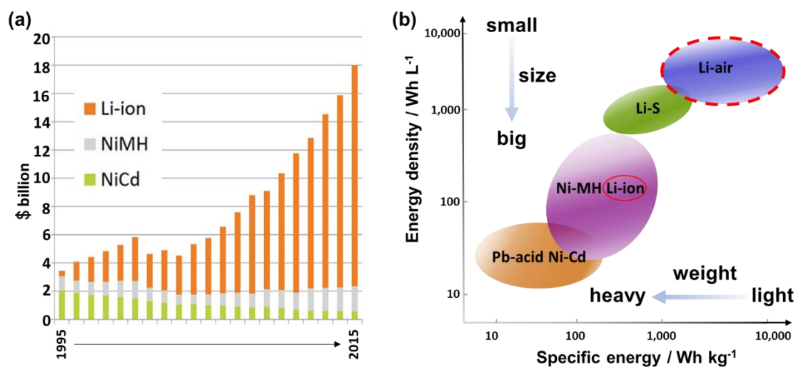
Figure 1-1. (a) Bar graph demonstrating the increase in financial support for LIB relative to NiCd and NiMH batteries from 1995 to 2015. (b) Comparison of specific energy and energy density of various batteries.
