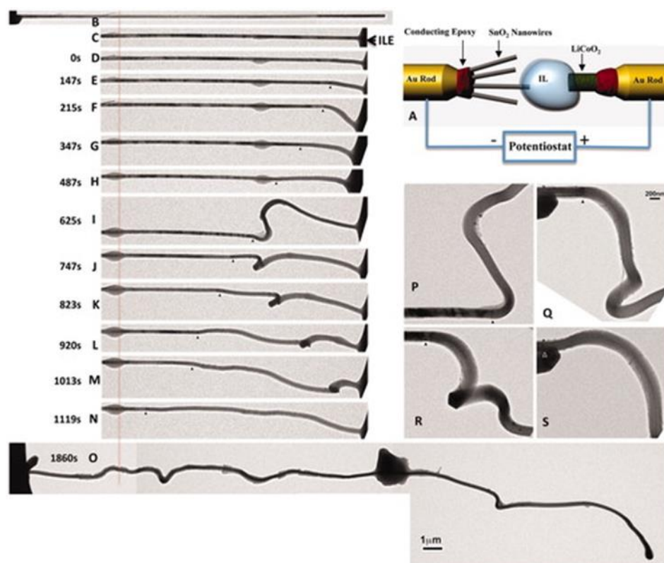
Figure 1-14. Time-lapse structure evolution of a \text{SnO}_2 nanowire anode during charging at -3.5 V against a \text{LiCoO}_2 cathode. 92
