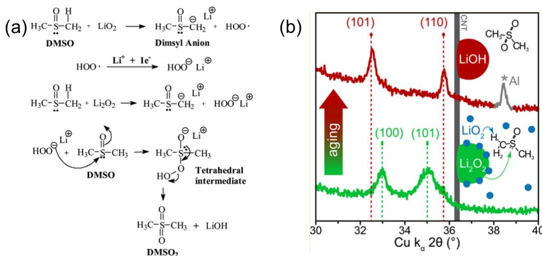
Figure 1- 8. (a) Proposed mechanism of degradation of DMSO. 71 [b] XRD patterns showing evolution of LiOH. 72
