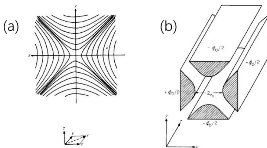
Figure 2-7. (a) Equipotential lines for a quadrupole field where \Phi = -1/2 E_0 \lambda (x^2 - y^2) ; (b) The electrode structure required to generate the potential shown in (a). These are the ideal quadrupole mass filter electrodes having hyperbolic cross-sections.
