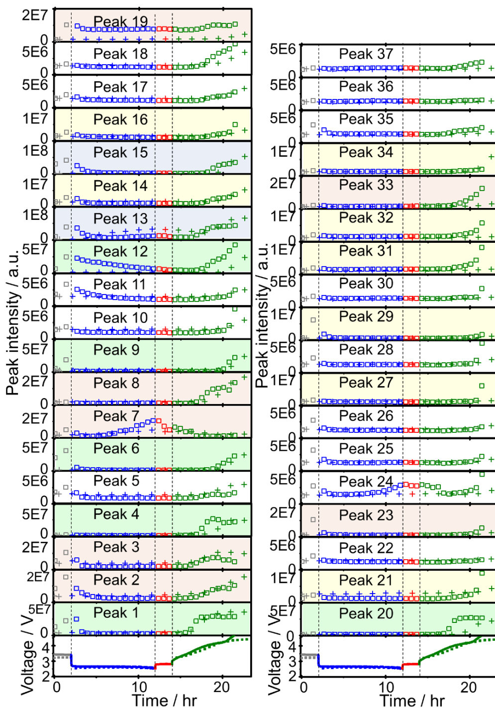
Figure 5-8. Voltage (bottom panels) and intensities of peaks 1 – 37 as a function of time for LOBs using TEGDME (BG) ( \square ) and TEGDME (HP) (+). Color coding is as of fig. 5-7 (a) and (b).
