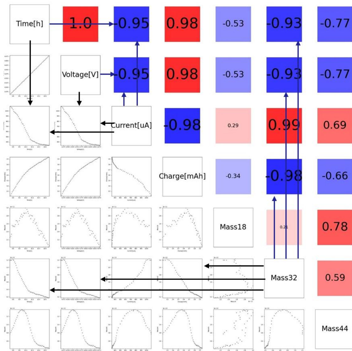
Figure 4-7. Python calculated correlation of mass numbers at voltage sweep from 4.45 to 4.68 V which is the second current minimum in Fig. 4-1(b) .
