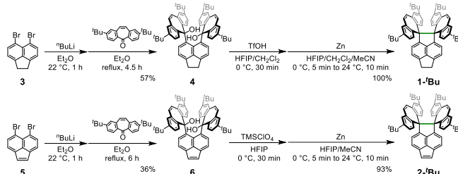
Scheme 1 Preparation of hydrocarbons 1-Bu and 2-Bu .
