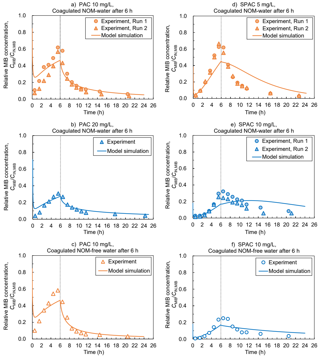
Fig. 11S. Comparison of experimental and simulated time courses of effluent/influent MIB concentration ratios ( C_{\text{MIB}}/C_{\text{IN,MIB}} ) in the SMHS with PAC (left panels) and SPAC (right panels). Simulations were conducted using setting B. The MIB-containing influent was replaced by MIB-free influent at 6 h (vertical dotted lines).
