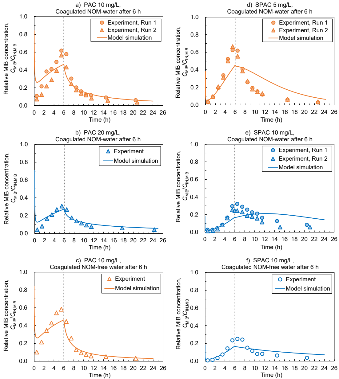
Fig. 10S. Comparison of experimental and simulated time courses of effluent/influent MIB concentration ratios ( C_{\text{MIB}}/C_{\text{IN,MIB}} ) in the SMHS with PAC (left panels) and SPAC (right panels). Simulations were conducted using setting A. The MIB-containing influent was replaced by MIB-free influent at 6 h (vertical dotted lines).
