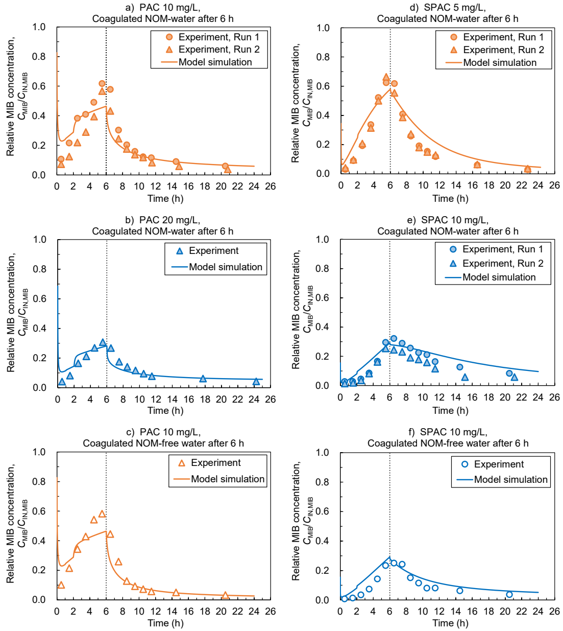
Fig. 15S. Comparison of experimental and simulated time courses of effluent/influent MIB concentration ratios ( C_{\text{MIB}}/C_{\text{IN,MIB}} ) in the SMHS with PAC (left panels) and SPAC (right panels). Simulations were conducted using setting G. The MIB-containing influent was replaced by MIB-free influent at 6 h (vertical dotted lines).
