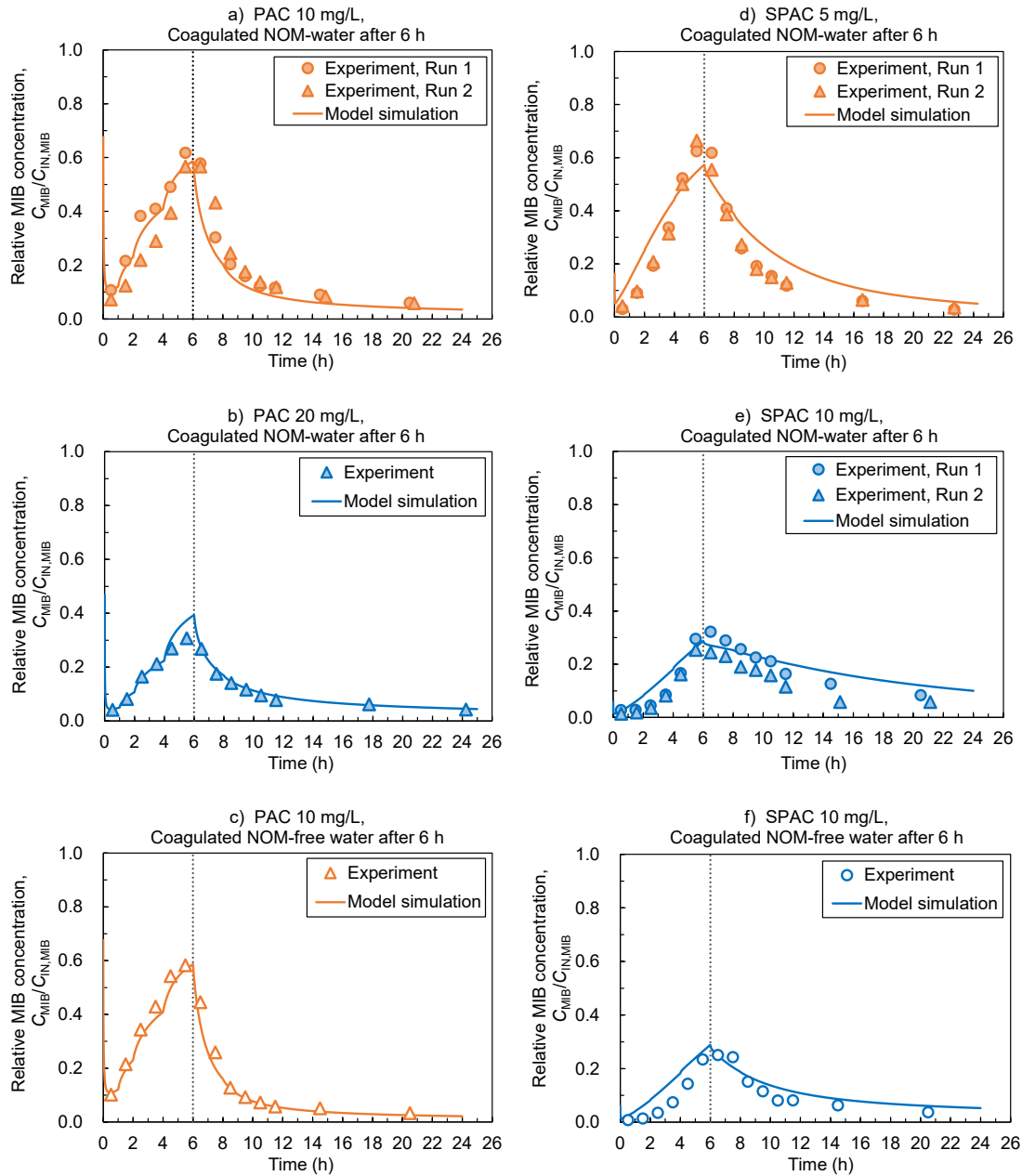
Fig. 6. Comparison of experimental and simulated time courses of effluent/influent MIB concentration ratios ( C_{\text{MIB}}/C_{\text{IN,MIB}} ) in the SMHS with PAC (left panels) and SPAC (right panels). Simulations were conducted using setting F. The MIB-containing influent (Coagulated MIB-spiked NOM-water, C_{\text{IN,MIB}} \approx 1 \mu\text{g/L} ) was replaced by MIB-free influent (either Coagulated NOM-water or Coagulated NOM-free water) at 6 h (vertical dotted lines).
