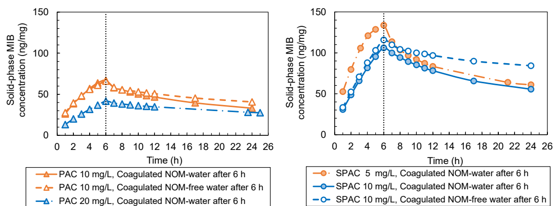
Fig. 4. Time course of solid-phase MIB concentrations (i.e., MIB adsorbed on AC) in the SMHS with PAC (left) and SPAC (right). The MIB-containing influent (Coagulated MIB-spiked NOM-water, C_{IN,MIB} \approx 1 \mu\text{g/L} ) was replaced by MIB-free influent (either Coagulated NOM-water or Coagulated NOM-free water) at 6 h (vertical dotted lines).
