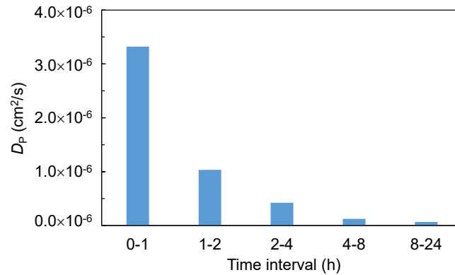
Fig. 7. Estimation of intraparticle diffusivity ( D_p ) in AC pores by means of best-fitting model simulation for setting F.
