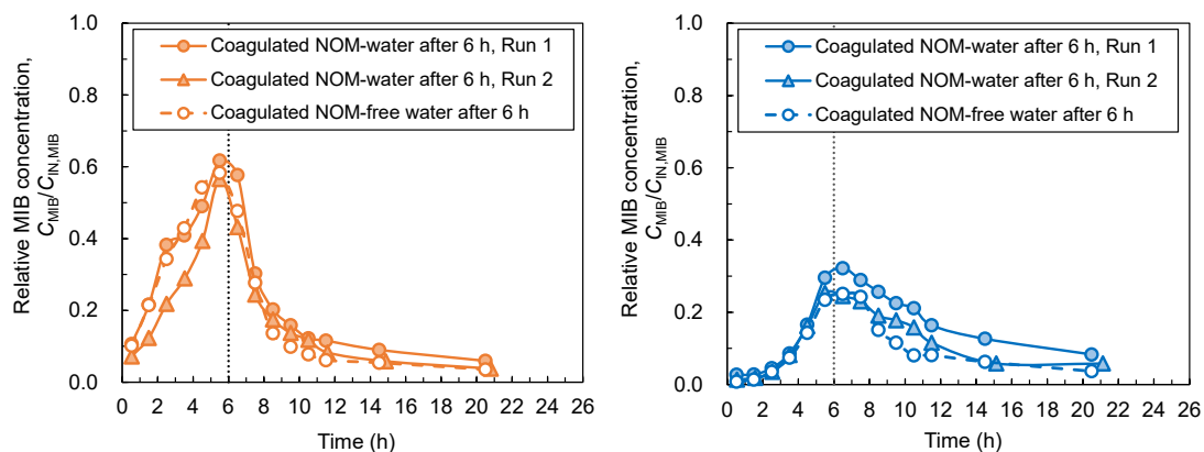
Fig. 3. Time course of effluent/influent MIB concentration ratios ( C_{MIB}/C_{IN,MIB} ) in the SMHS with 10 mg/L PAC (left panel) and 10 mg/L SPAC (right panel). The solid and dashed lines indicate data for tests in which MIB-containing influent (Coagulated MIB-spiked NOM-water, C_{IN,MIB} \approx 1 \mu\text{g/L} ) was replaced by MIB-free water, either Coagulated NOM-water or Coagulated NOM-free water, respectively, at 6 h (vertical dotted lines). The x-axis values of the plots are times in the middle of each sampling period.
