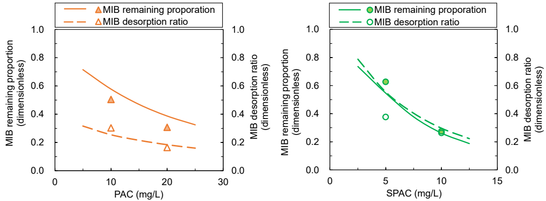
Fig. 8. Effects of PAC (left) and SPAC (right) dosage on MIB remaining proportion and MIB desorption ratio. The symbols indicate experimental data; the lines represent the data of model simulation by using optimized parameters of setting F. The MIB remaining proportions were determined at 6 h, just before the MIB-containing influent ( C_{IN,MIB} = 1 \mu\text{g/L} ) was replaced by the MIB-free influent. The MIB desorption ratio is the ratio of the amount of MIB desorbed during the first 6 h of the no-contamination period divided by the amount of MIB adsorbed during the 6 h of the contamination period.
