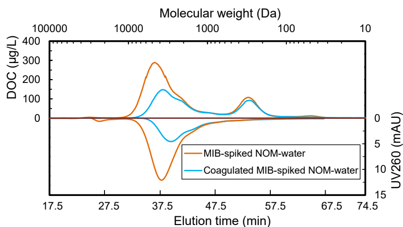
Fig. 4S. Molecular weight distributions of NOM in MIB-spiked NOM-water and Coagulated MIB-spiked NOM-water.
