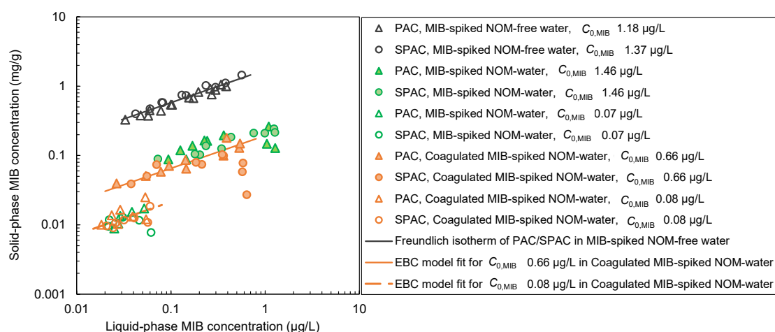
Fig. 5. Isotherms for adsorption of MIB on PAC and SPAC from MIB-spiked NOM-free water, MIB-spiked NOM-water, and Coagulated MIB-spiked NOM-water.
