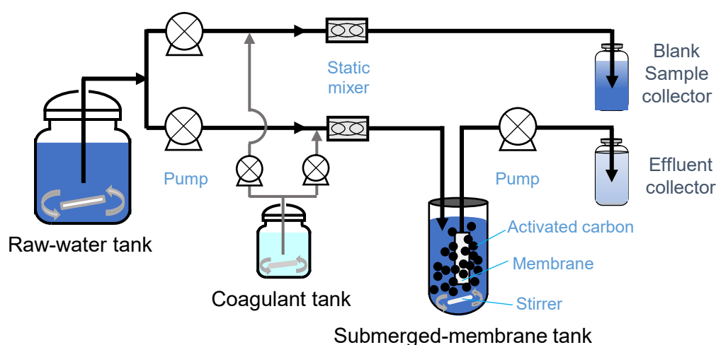
Fig. 1. Schematic diagram of the SMHS(submerged-membrane hybrid system)-PAC(powdered activated carbon)/SPAC(superfine powdered activated carbon) used in this study.
