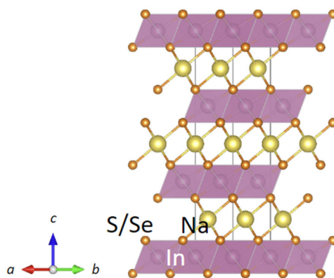
Fig. 1. Crystal Structure of \text{NaInS}_{2-x}\text{Se}_x .
