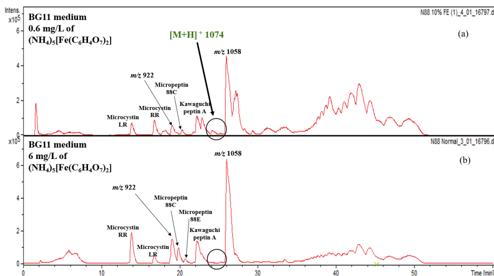
Figure 2: Chromatogram of crude extracts of M. aeruginosa grown in (a) BG-11 medium with 0.6 mg/L of (\text{NH}_4)_5[\text{Fe}(\text{C}_6\text{H}_4\text{O}_7)_2] (b) BG-11 medium with 6 mg/L of (\text{NH}_4)_5[\text{Fe}(\text{C}_6\text{H}_4\text{O}_7)_2] .
