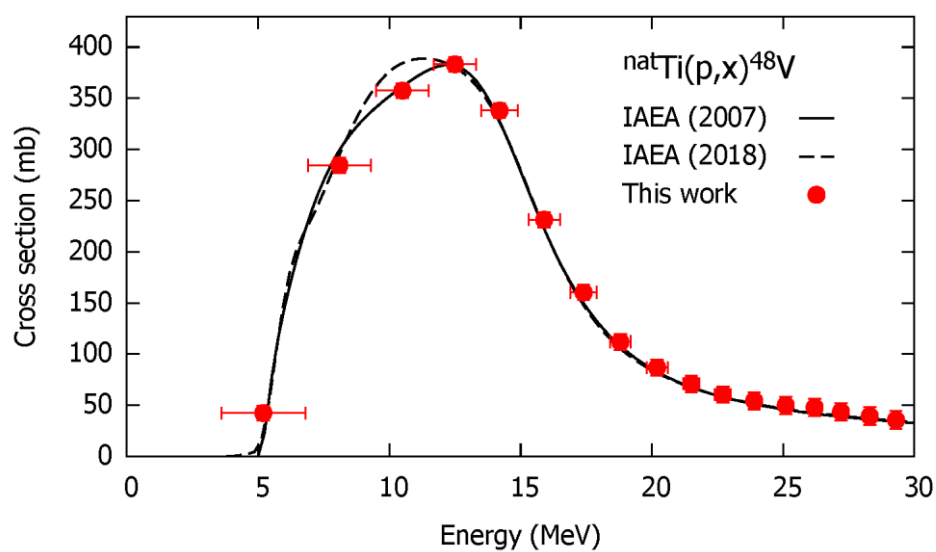
Fig. 1. Excitation function of the ^{\text{nat}}\text{Ti}(p,x)^{48}\text{V} monitor reaction with the recommended values [17,18].
