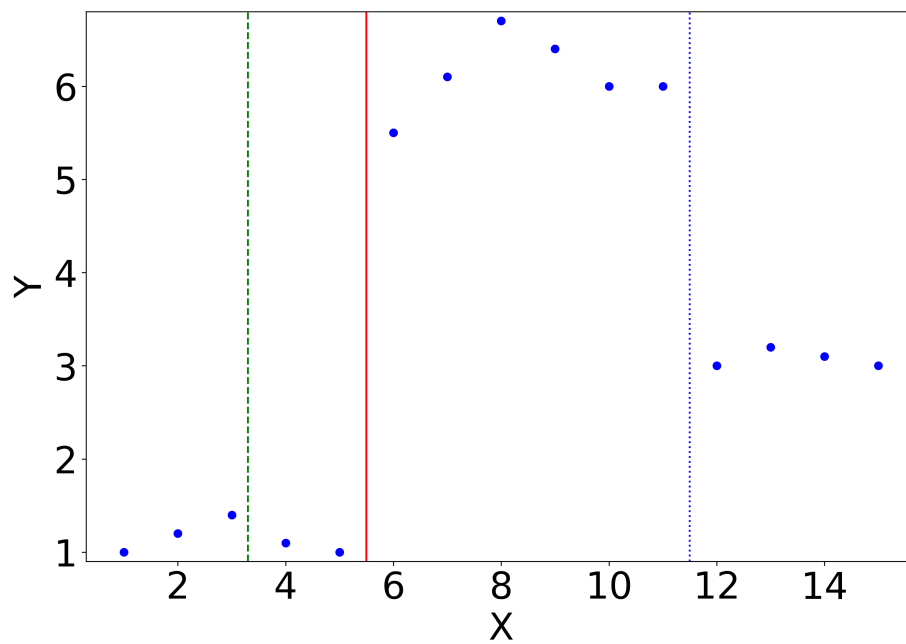
Fig. 2.7. Scatter plots with splitting lines.
