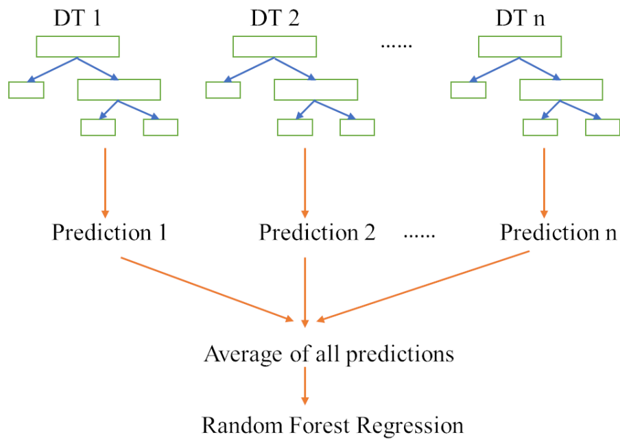
Fig. 2.6. Schematic diagram of Random Forest Regression.
