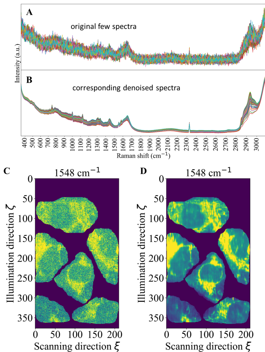
Fig. A.4. For the Raman image of FTC-133(#2) (A) few individual pixel level raw Raman spectra (B) corresponding denoised spectra, (C-D) intensity distribution at 1548 \text{ cm}^{-1} : (C) raw Raman image, (D) denoised Raman image.
