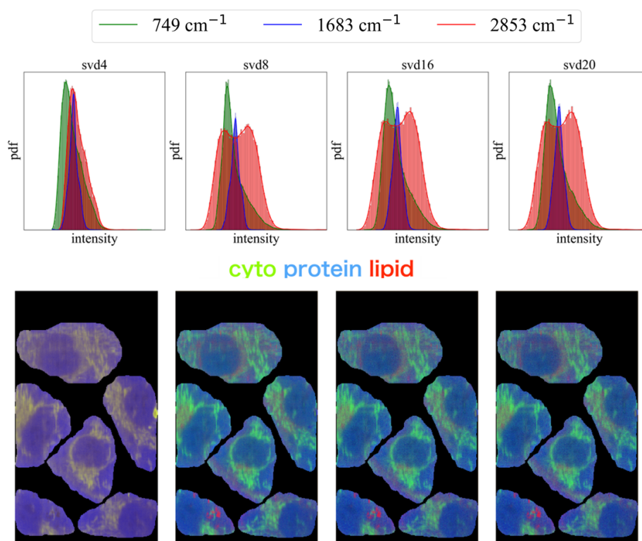
Fig. A.2. The Raman intensity distribution at known cytochrome peak 749 \text{cm}^{-1} , protein peak 1683 \text{cm}^{-1} and lipid peak 2853 \text{cm}^{-1} for the Raman image of FTC-133(#2) for different singular value decomposition components.
