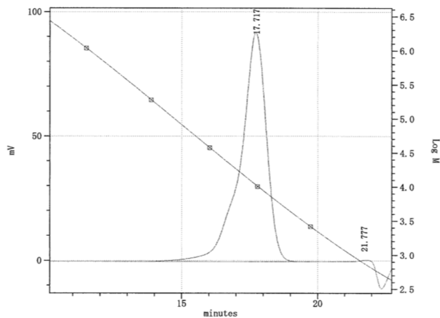
Figure S-2. n -BuLi Initiated Polymerization of Styrene in The Flow System (flow rate of n -BuLi (0.05 M) = 5.0 mL/min, flow rate of Styrene (2.0 M) = 15.0 mL/min, T-250-250 mixer, 30 degree-C)
