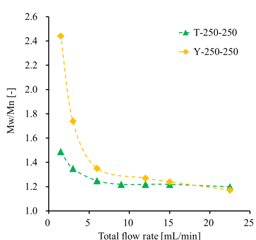
Figure 7. Comparing V-shape and T- shape mixers
