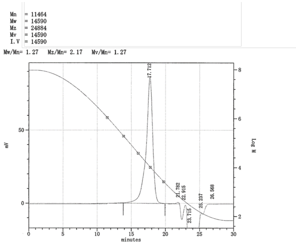
Figure S-19. n -BuLi Initiated Polymerization of Styrene in The Flow System (flow rate of n -BuLi (0.05 M) = 2.0 mL/min, flow rate of Styrene (2.0 M) = 4.0 mL/min, T-250-250 mixer, -20 degree-C)
