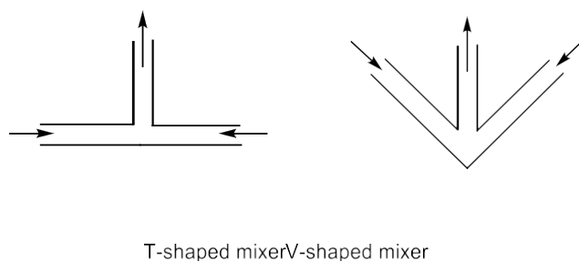
Figure 6. Schematic diagrams of the T-shaped micromixer and the V-shaped micromixer.
