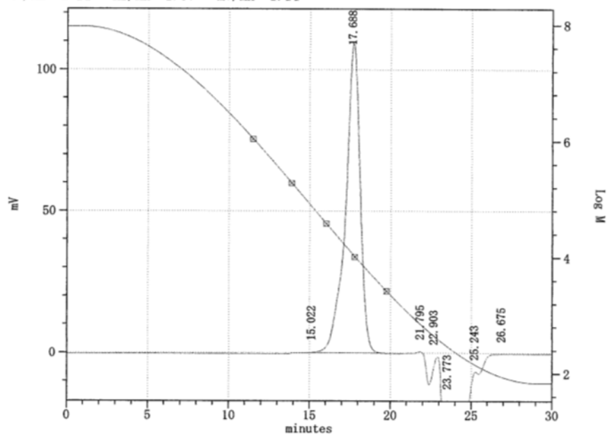
Figure S-8. n -BuLi Initiated Polymerization of Styrene in The Flow System (flow rate of n -BuLi (0.05 M) = 7.5 mL/min, flow rate of Styrene (2.0 M) = 15.0 mL/min, T-250-250 mixer, 0 degree-C)
