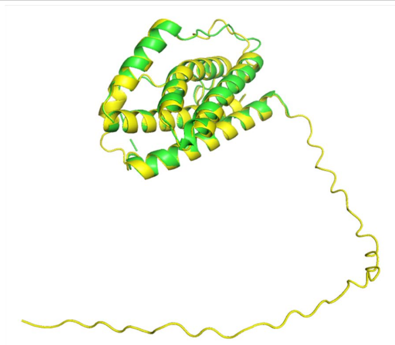
Figure S1. Structural analysis of IL-6 (a) dimer structure reported in PDB (PBD: 1ALU), (b) Structural comparison of PDB (green) and AlphaFold-2 (yellow), root mean square deviation = 0.359Å
