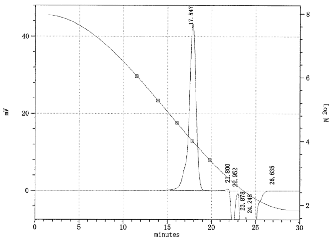
Figure S-53. n -BuLi Initiated Polymerization of Styrene in The Flow System (flow rate of n -BuLi (0.05 M) = 7.5 mL/min, flow rate of Styrene (2.0 M) = 15.0 mL/min, T-250-250 mixer, 30 degree-C, 2 nd trial)
