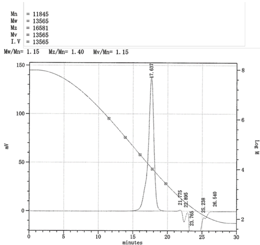
Figure S-15. n -BuLi Initiated Polymerization of Styrene in The Flow System (flow rate of n -BuLi (0.05 M) = 7.5 mL/min, flow rate of Styrene (2.0 M) = 15.0 mL/min, T-250-250 mixer, -20 degree-C)
