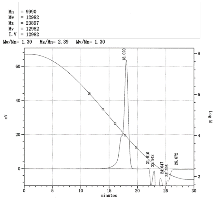
Figure S-37. n -BuLi Initiated Polymerization of Styrene in The Flow System (flow rate of n -BuLi (0.05 M) = 2.0 mL/min, flow rate of Styrene (2.0 M) = 4.0 mL/min, T-250-500 mixer, 30 degree-C)
