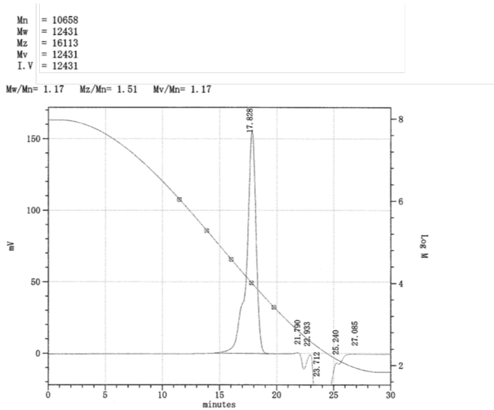
Figure S-22. n -BuLi Initiated Polymerization of Styrene in The Flow System (flow rate of n -BuLi (0.05 M) = 5.0 mL/min, flow rate of Styrene (2.0 M) = 10.0 mL/min, T-500-500 mixer, 30 degree-C)
