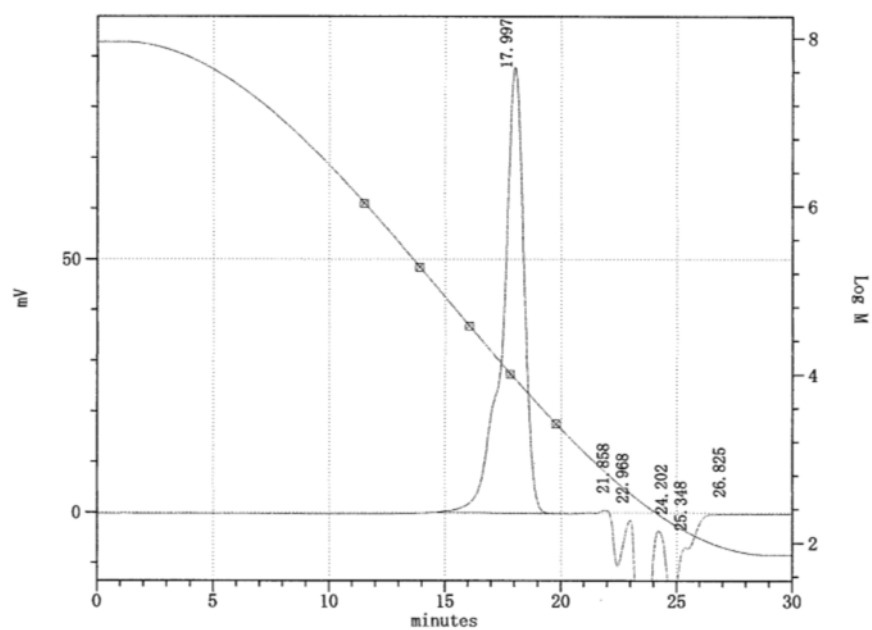
Figure S-34. n -BuLi Initiated Polymerization of Styrene in The Flow System (flow rate of n -BuLi (0.05 M) = 5.0 mL/min, flow rate of Styrene (2.0 M) = 10.0 mL/min, T-250-500 mixer, 30 degree-C)
