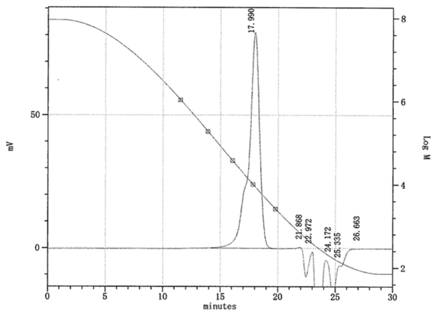
Figure S-35. n -BuLi Initiated Polymerization of Styrene in The Flow System (flow rate of n -BuLi (0.05 M) = 4.0 mL/min, flow rate of Styrene (2.0 M) = 8.0 mL/min, T-250-500 mixer, 30 degree-C)
