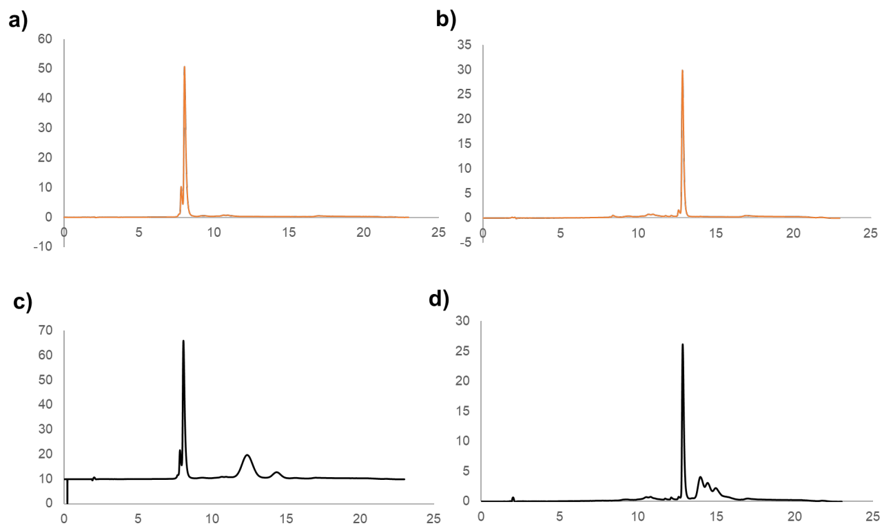
Figure S4. RP-HPLC analysis (a) naked lysozyme (b) naked IL-6 (c) PEGylated lysozyme produced by continuous flow mode (d) PEGylated IL-6 produced by continuous flow mode
