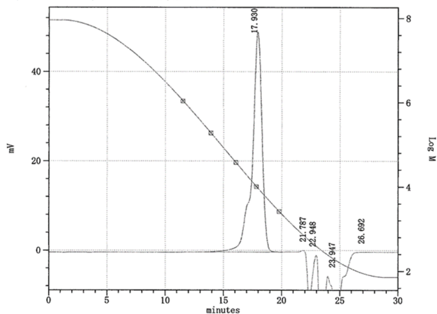
Figure S-40. n -BuLi Initiated Polymerization of Styrene in The Flow System (flow rate of n -BuLi (0.05 M) = 7.5 mL/min, flow rate of Styrene (2.0 M) = 15.0 mL/min, T-500-250 mixer, 30 degree-C)
