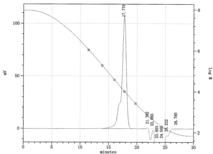
Figure S-3. n -BuLi Initiated Polymerization of Styrene in The Flow System (flow rate of n -BuLi (0.05 M) = 4.0 mL/min, flow rate of Styrene (2.0 M) = 8.0 mL/min, T-250-250 mixer, 30 degree-C)
