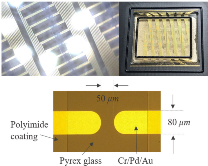
Figure 3.A.3: Actual electrode array graph and the magnified parts of one of its pairs. The test end of electrode array for polymer wire growth consists of 90 pairs of rounded tip Au electrodes with a gap of \mu\text{m} . The wiring area is covered by polyimide film.
