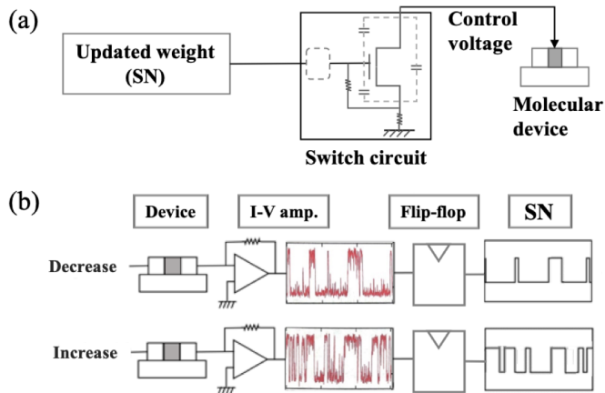
Figure 4.A.4: Realization method of weight update SN circuit using molecular element.
