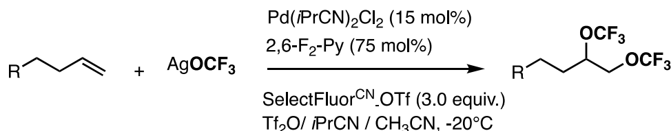
Scheme 7 : Palladium-catalyzed intermolecular ditrifluoromethoxylation of unactivated alkenes: CF 3 O-palladation initiated by Pd(IV). (2018)
