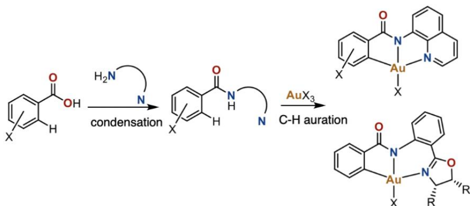
Figure 2.2: Direct C-H auration using N-(8-quinoliny)benzamide derivatives as ligands for Au(III) pincer complexes .
