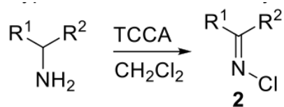
Scheme 3.7: Typical N -chloroketimines synthesis.
