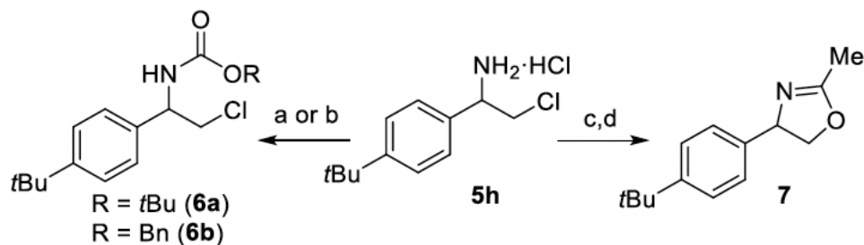
Scheme 3.10: Transformations of chloroamine 5h . [a] Boc 2 O (2 equiv), NEt 3 (2.2 equiv), CH 2 Cl 2 , rt, 17 h, 72% yield. [b] CbzCl (2 equiv), NaHCO 3 (2 equiv), THF, 0°C, 15 min, 55% yield. [c] Ac 2 O (3 equiv), NEt 3 (3.5 equiv), THF, rt, 1.5 h, 74% yield. [d] NEt 3 (2 equiv), TBAI (0.5 equiv), THF, 80°C, 7 h, 80% yield.
