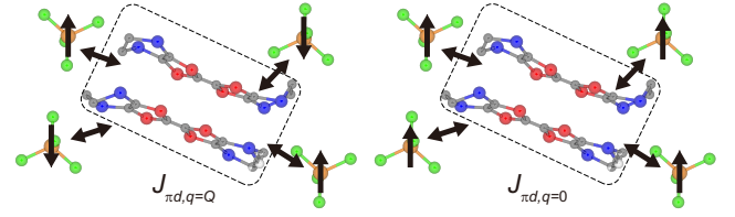
FIG. 6. Antiferromagnetic structure with q = Q ( J_{\pi d, q=Q} ) and the ferromagnetic structure with q = 0 ( J_{\pi d, q=0} ). The two-headed arrows between a dimer and anions represent the \pi - d interaction.
