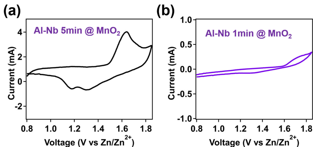
Figure S23. CV curves obtained from (a) the Al-Nb samples prepared by sputtering for 5 min and (b) the Al-Nb samples prepared by sputtering for 1 min. The sweep rate is 0.5 mV s -1 .
