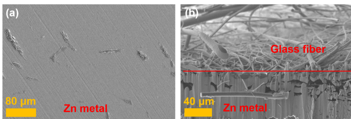
Figure S10. SEM images of Zn deposited on Al-Nb foil under high current density (25 mA cm -2 ). (a) Top view of the Zn coating and (b) cross sectional observation of the Zn coating.
