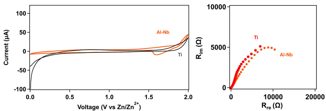
Figure S21. CV test of Zn||Ti foil half cells at the scanning rate of 0.5 \text{ mV s}^{-1} (left), and the Nyquist plot of Zn||Ti foil half cells (right).
