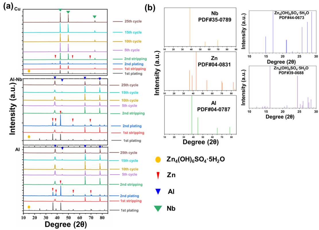
Figure S15. (a) Ex-situ XRD patterns of different substrates after Zn plating/stripping, from top to bottom are Cu, Al-Nb, and Al, respectively. (b) Standard XRD patterns of the related materials.
