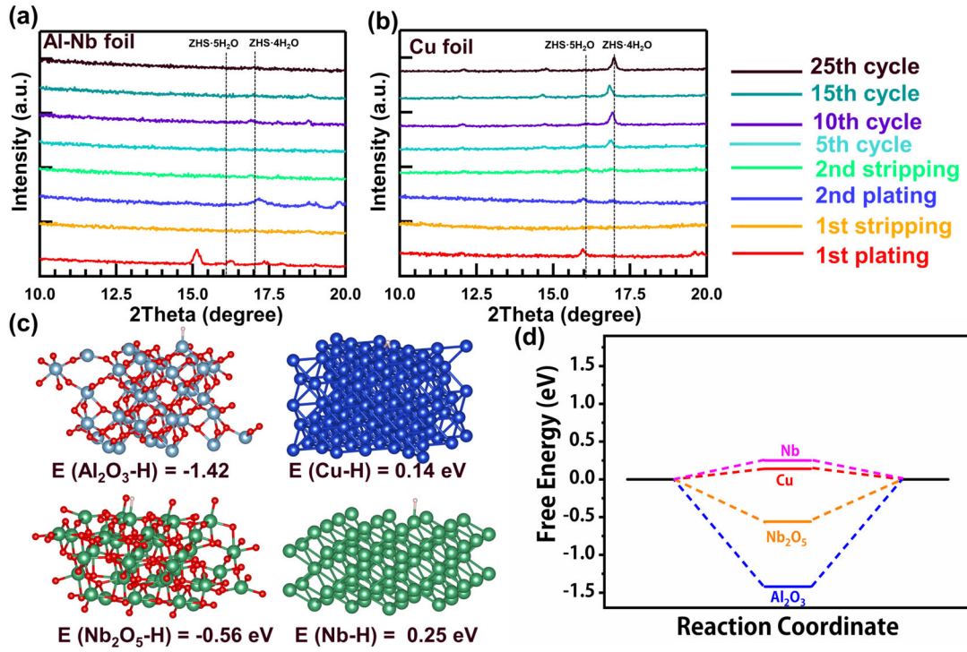
Figure 4. Ex-situ XRD patterns of different substrates after Zn plating/stripping. XRD patterns at different stage for (a) Al-Nb foil and (b) Cu foil. The plating/stripping current density is 10 mA cm -2 and the capacity is 5 mAh cm -2 . (c) The used models for DFT simulation. (d) Free-energy barriers for HER on different substrates.
