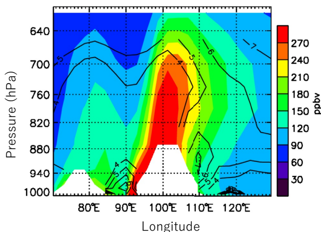
Figure 14. As in Figure 13, but for the CO mixing ratio in the control experiment.
