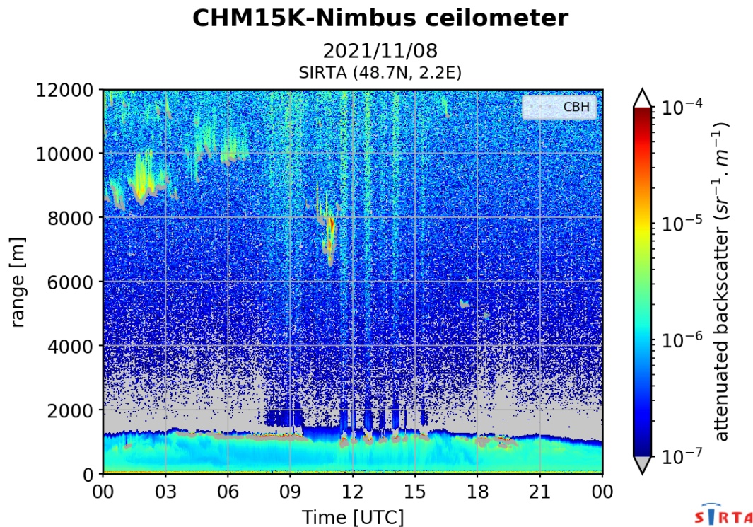
Figure 2: Measurements from a ceilometer at the same site on the same day as for Figure 1. Taken from https://sirta.ipsl.fr/bdd/pub/basesirta/1a/chm15k/2021/11/08/chm15k.1a_z1Ppr2R15mF15s_v01_20211108_000000_1440.png (accessed June 21, 2022).
