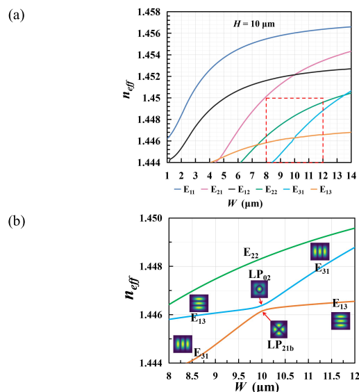
Fig. 2 (a) Waveguide width dependency of the effective refractive index when H = 10\mu\text{m} . (b) The detail image of the region of W = 8 \sim 12\mu\text{m} , as shown in the region enclosed by the red dashed line in Fig. 2(a).
