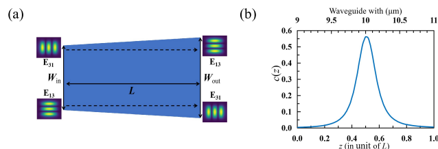
Fig. 3 (a) Linear taper structure with input waveguide width W_{\text{in}} = 9\mu\text{m} and output waveguide width W_{\text{out}} = 11\mu\text{m} . (b) The adiabaticity parameter c(z) for the E_{31} and E_{13} or these hybrid modes in the linear taper waveguide from W_{\text{in}} = 9\mu\text{m} to W_{\text{out}} = 11\mu\text{m} .
