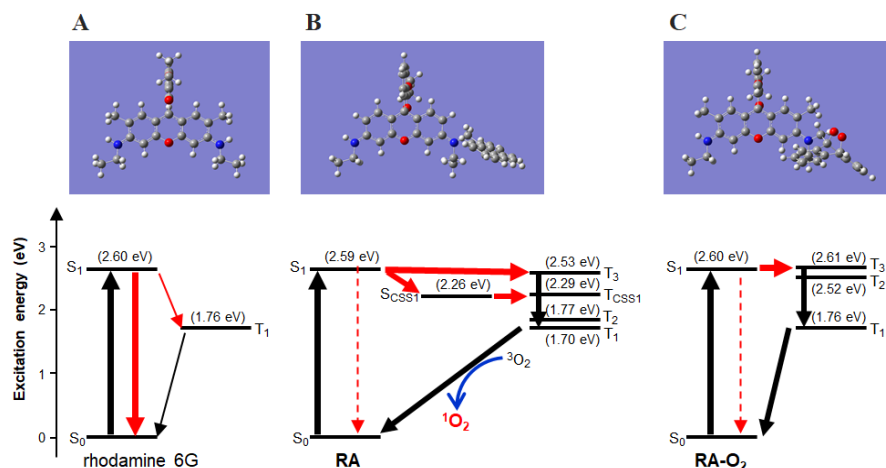
Figure 5. Optimized structures and energy levels predicted for (A) rhodamine 6G, (B) RA , and (C) RA-O 2 , by the DFT calculations at the UB3LYP/6-311+G** level with SCRF where DMF is the solvent. CSS denotes a charge-separated state.
