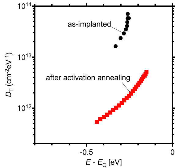
FIG. 7. D_{it} distributions at the ALD \text{Al}_2\text{O}_3/\text{GaN} interface formed with as-implanted GaN and that formed after activation annealing at 1250 °C. Data for the as-implanted sample are taken from our previous report. Taken with permission from Akazawa et al. , Jpn. J. Appl. Phys. 60 , 016502 (2021). Copyright 2020 The Japan Society of Applied Physics.
