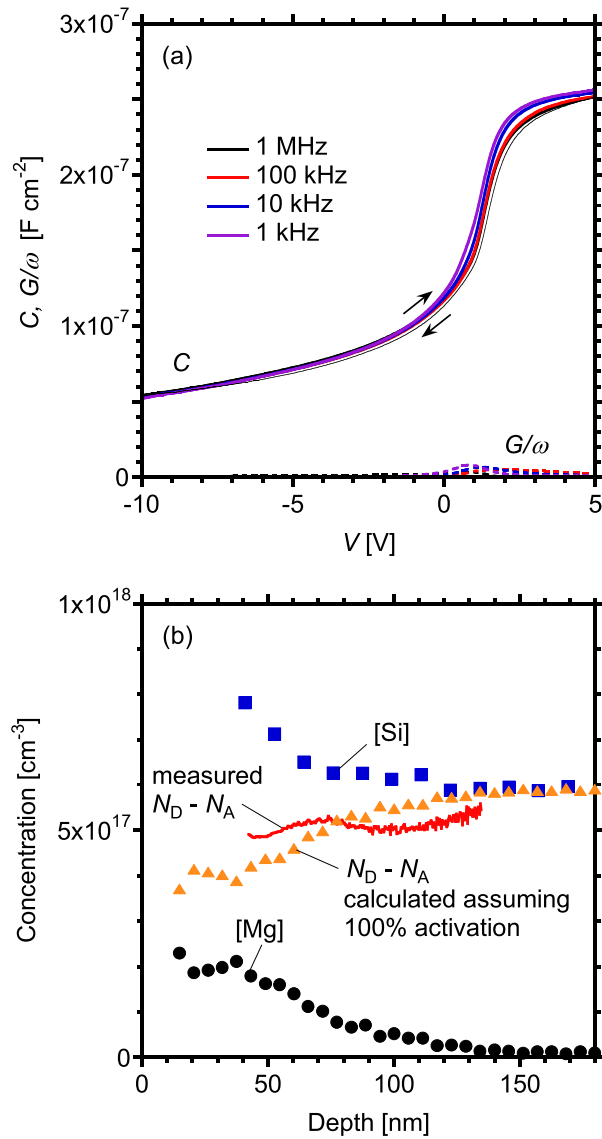
FIG. 5. (a) C-V characteristics of completed MOS diode. The thin black line indicates the C-V curve measured from the positive bias side to the negative bias side only for the 1 MHz curve to show the hysteresis, while the thick lines indicate the curve measured in the opposite direction. (b) N_D - N_A profiles derived from 1 MHz C-V curve (solid line). The SIMS [Mg] (solid circles) and [Si] (solid rectangles) profiles in Fig. 3 appear again. The N_D - N_A profile calculated for the 100% activation of Mg acceptors is also plotted (solid triangles).
