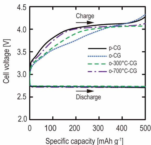
Figure 6 Discharge-charge curves of surface-modified CGs. (Current density: 50 \text{mA g}^{-1} , discharge-charge capacity limitation: 500 \text{mAh g}^{-1} ) The measurements were conducted using coin-type cells.
