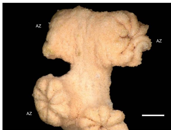
Fig. 6. Detail of twig of Hemicorallium meraboshi sp. nov., NSMT-Co 1801. Abbreviation: AZ, autozooid. Scale bar: 1.0 mm.
