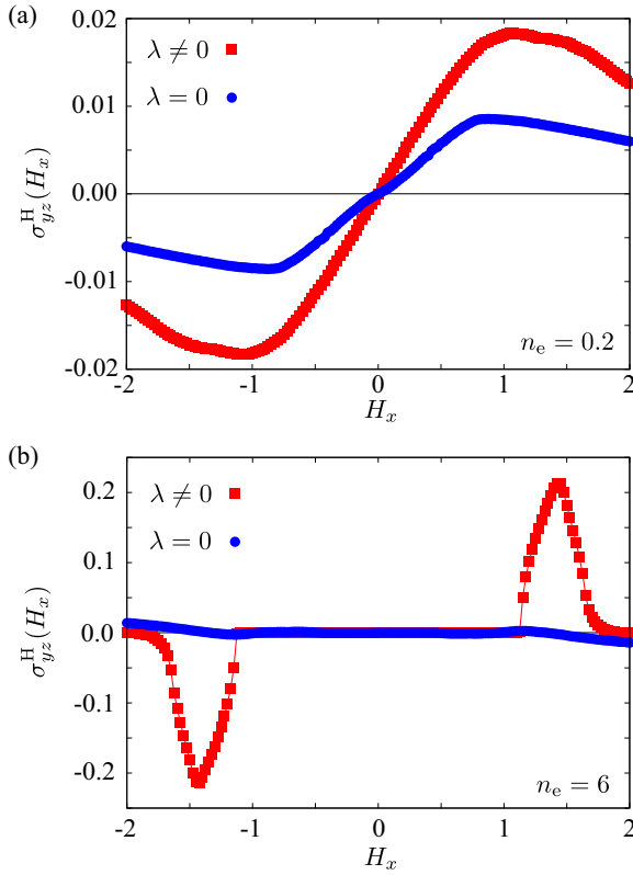
FIG. 4. H_x dependence of the conventional Hall conductivity \sigma^H_{yz}(H_x) at \lambda = 0 and 2 for (a) n_e = 0.2 and (b) n_e = 6 .
