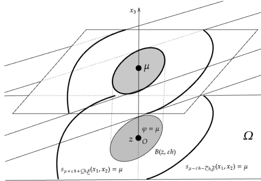
Figure 4: Level sets of s_{\mu-\varepsilon h-\overline{C}h, \overline{\beta}} , s_{\mu+\varepsilon h+\underline{C}h, \underline{\beta}} and \varphi .
