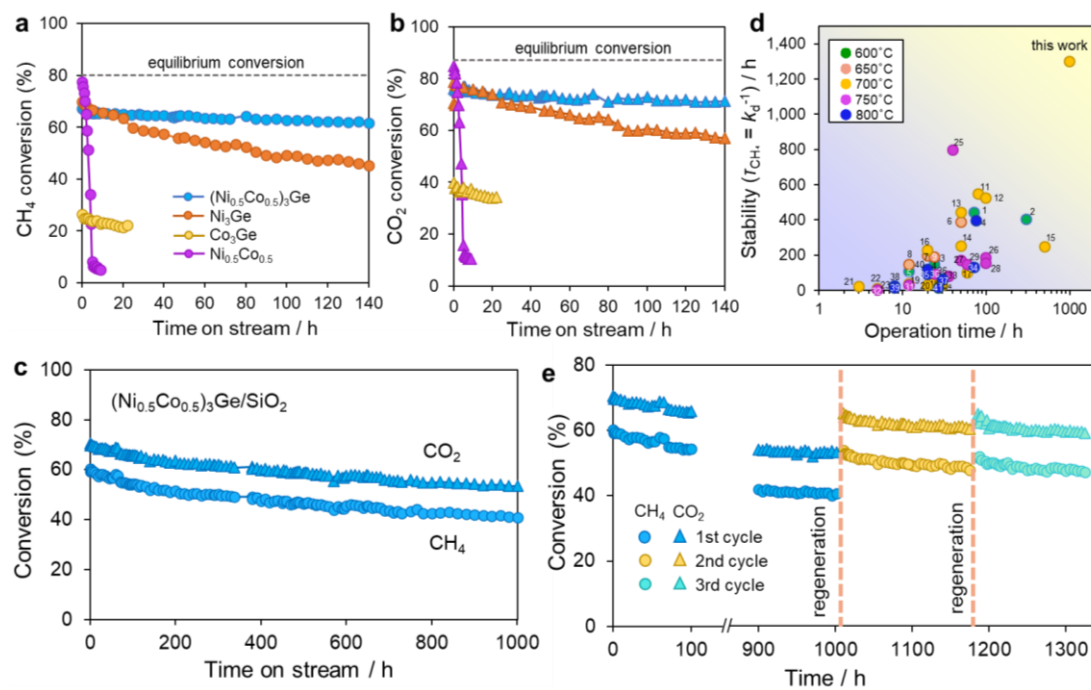
Figure 2.10. Catalytic performance of Ni-based catalysts in DRM. Reaction conditions: catalyst amount of 100 mg, \text{CH}_4\text{:CO}_2\text{:Ar} = 10\text{:}10\text{:}20 \text{ mL}\cdot\text{min}^{-1} , 700^\circ\text{C} , 1 bar. a, b Time course of (a) \text{CH}_4 Conversions and (b) \text{CO}_2 Conversions. c Long-term stability of \text{CH}_4 conversion and \text{CO}_2 conversion over (\text{Ni}_{0.5}\text{Co}_{0.5})_3\text{Ge/SiO}_2 . d Comparison of the stability with reported Ni-based DRM catalysts under equilibrium conversion. Numbers correspond to the entries in Table 2.3. e Regeneration test using (\text{Ni}_{0.5}\text{Co}_{0.5})_3\text{Ge/SiO}_2 during three catalytic cycles. Regeneration conditions: \text{CO}_2\text{:Ar} = 10\text{:}10 \text{ mL}\cdot\text{min}^{-1} for 7 h, followed by \text{H}_2 of 10 \text{ mL}\cdot\text{min}^{-1} for 1 h at 700^\circ\text{C} .
