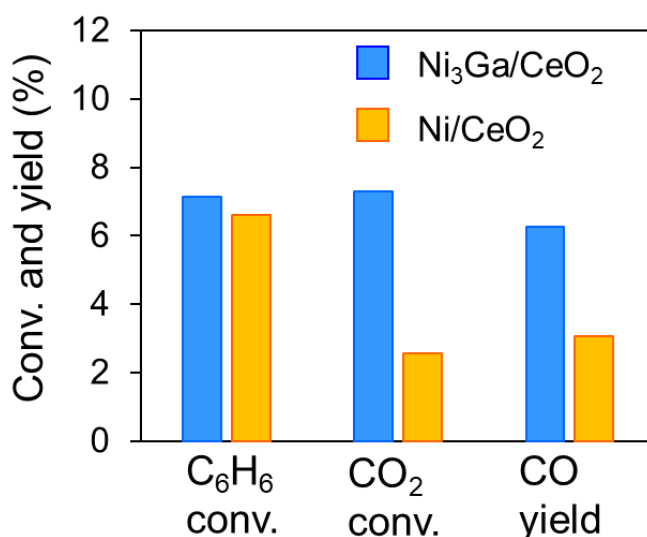
Figure 3.8. Catalytic performance of \text{Ni}_3\text{Ga}/\text{CeO}_2 and \text{Ni}/\text{CeO}_2 in the DRB. Reaction conditions: catalyst amount, 100 mg; flow rate, \text{C}_6\text{H}_6:\text{CO}_2:\text{He} = 2.4:14.4:20 \text{ mLmin}^{-1} ; temperature, 500^\circ\text{C} . Values at a time-on-stream of 125 min are shown.
