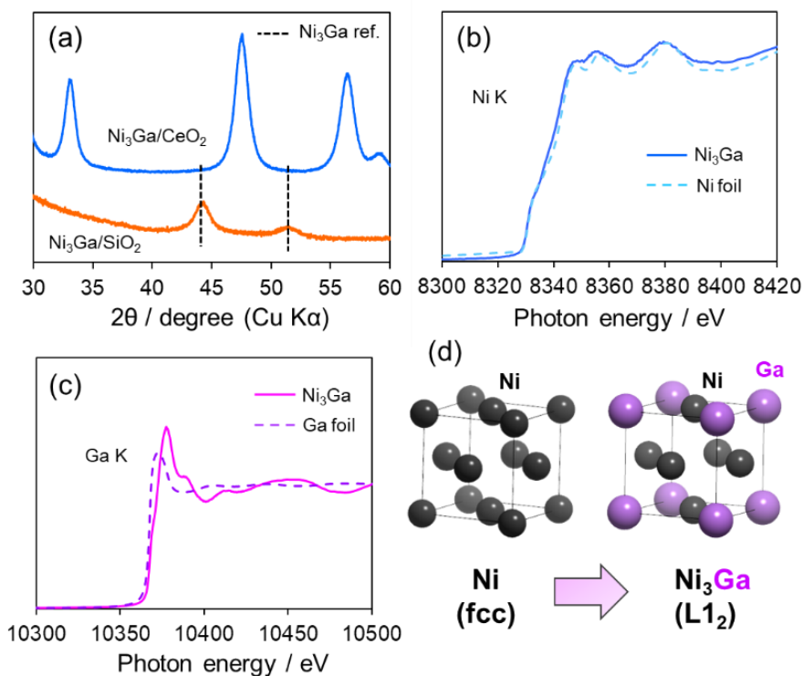
Figure 3.2. (a) XRD patterns of \text{Ni}_3\text{Ga} supported by \text{SiO}_2 and \text{CeO}_2 . (b), (c) Ni K- and Ga K-edge XANES spectra of the in situ reduced catalysts (solid lines) and reference foils (dashed lines). (d) Model of the \text{Ni}_3\text{Ga} intermetallic structure with the crystal structure unit.
