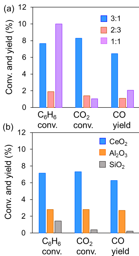
Figure 3.11. Catalytic performance of (a) \text{Ni}_{1-x}\text{Ga}_x/\text{CeO}_2 with different Ni:Ga ratios and (b) \text{Ni}_3\text{Ga} on different supports ( \text{CeO}_2 , \text{Al}_2\text{O}_3 , and \text{SiO}_2 ) in the DRB (values at a time-on-stream of 95 min and 125 min are shown, respectively).
