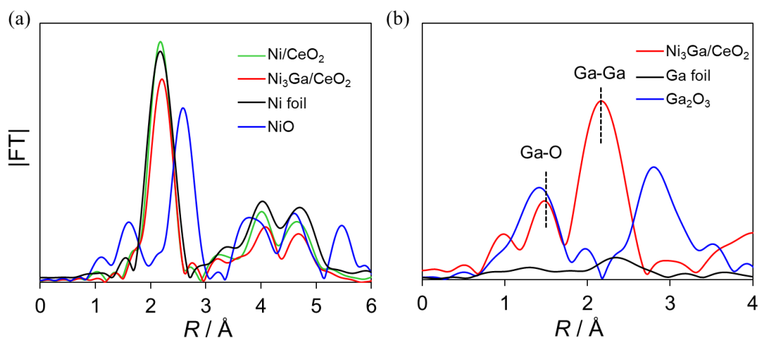
Figure 3.4. Fourier-transforms of EXAFS in (a) Ni, (b) Ga K-edge of the Ni 3 Ga/CeO 2 and Ni/CeO 2 catalysts and reference compounds.
