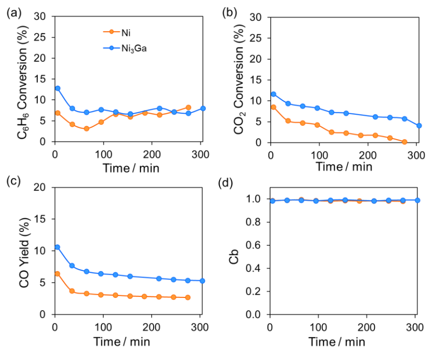
Figure 3.9. (a) \text{C}_6\text{H}_6 conversion, (b) \text{CO}_2 conversion (c) Product CO yield, (d) Carbon balance of \text{Ni}_3\text{Ga}/\text{CeO}_2 and \text{Ni}/\text{CeO}_2 .
