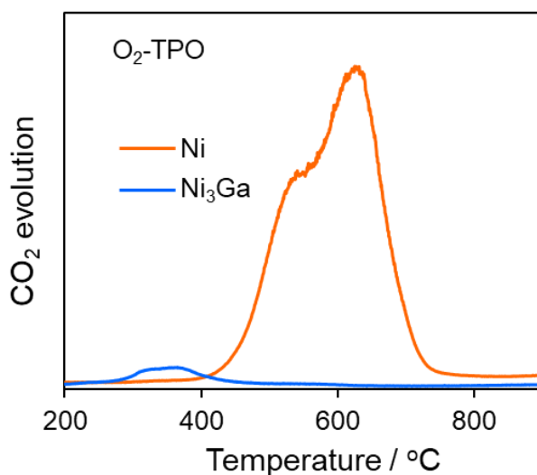
Figure 3.15. \text{O}_2 -TPO profiles of spent \text{Ni}_3\text{Ga}/\text{CeO}_2 and \text{Ni}/\text{CeO}_2 in the DRB.
