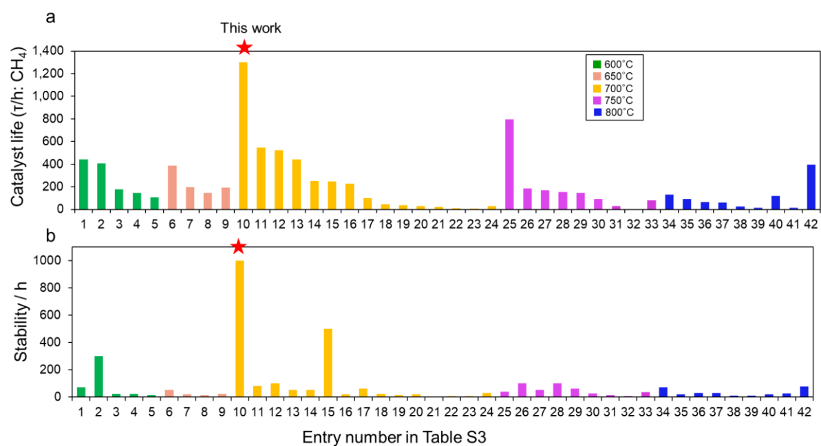
Figure 2.19. Catalytic performance of (Ni 0.5 Co 0.5 ) 3 Ge/SiO 2 and reported Ni-based systems for DRM under equilibrium conversion. (a) Mean catalyst life ( \tau = k_d^{-1} ), (b) Stability time.
