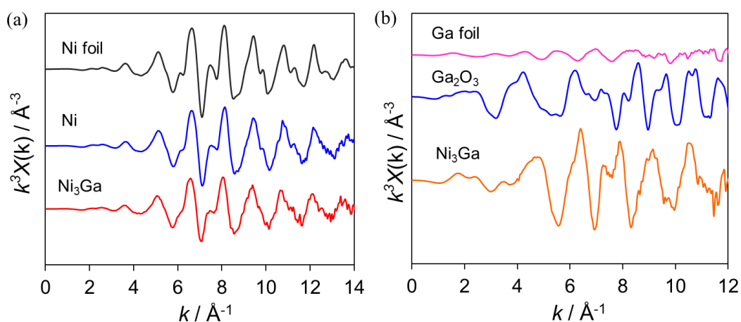
Figure 3.3. (a) Ni and (b) Ga K-edge extended X-ray absorption fine structure (EXAFS) spectra of the Ni 3 Ga/CeO 2 and Ni / CeO 2 catalysts and reference compound.
