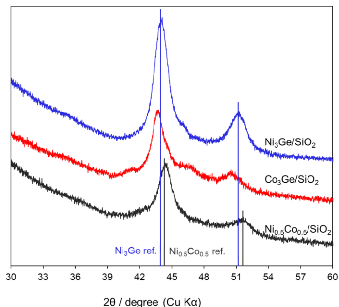
Figure 2.9. XRD patterns of \text{Ni}_3\text{Ge}/\text{SiO}_2 , \text{Co}_3\text{Ge}/\text{SiO}_2 , and \text{Ni}_{0.5}\text{Co}_{0.5}/\text{SiO}_2 catalysts.
