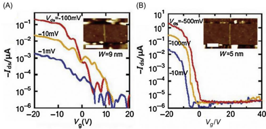
Figure 1.10 Graphene nanoribbon was applied in FETs and the switching ratio test. [adapted from 100 ]
