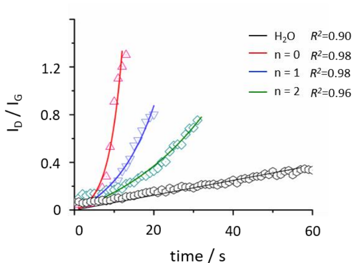
Figure 2A4 Fitting of I_D/I_G at the initial stage with formula 1 (formic is similar with water), R^2 : residual square
