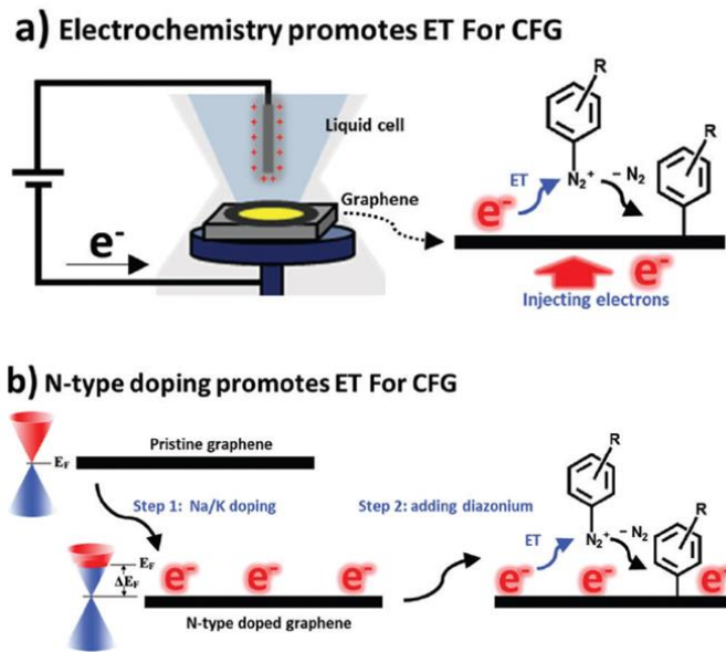
Figure 1.21 Electrochemical covalent modification on graphene [adapted from 178 ]
