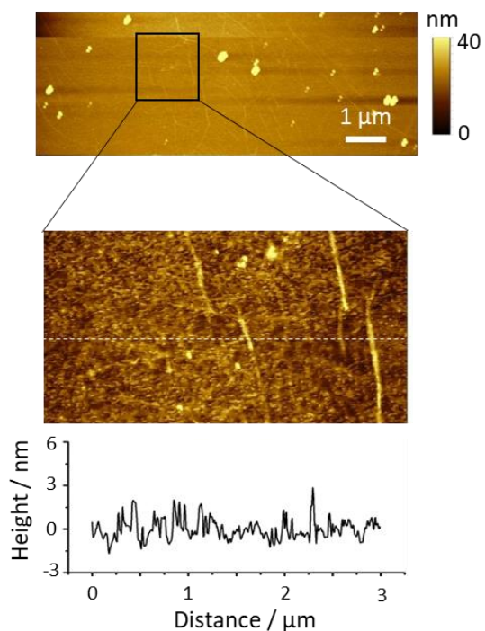
Figure 3A5 AFM measurement on single LB layer at the molar ratio of [SA] / [DiO] ~10: 1 (a) and ~10: 3 (b), respectively. The corresponding height profiles are presented at the bottom.
