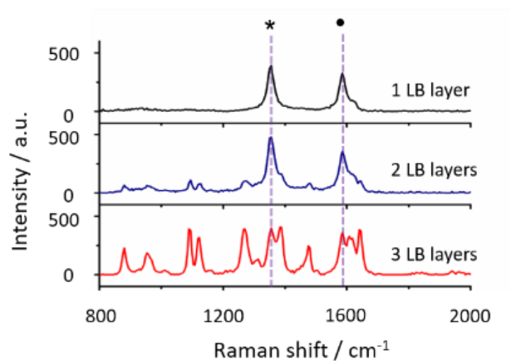
Figure 3A4 Raman spectra of DiO molecule with different layer numbers of the LB film on the PICM graphene substrate. Raman signals of DiO molecules are detected over double LB layers. The peaks marked with '*' and '•' correspond to the D and G bands of the graphene, respectively.
