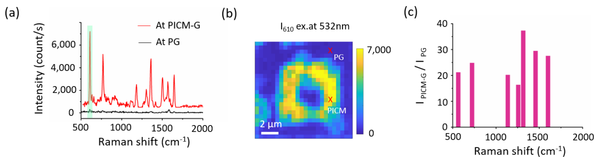
Figure 3.3 (a) GERS of Rh6G on PG and PICM-G excited at 488 nm. The green highlight represents the peak of Rh6G at 610 cm -1 used for mapping. (b) GERS mapping of Rh6G ( I_{610} , peak intensity at 610 cm -1 ) from the PG and PICM domain under 532 nm laser excitation (0.98 MW/cm 2 ). The red crosses on the Raman maps represent the PICM and PG regions, respectively. (c) Peak intensity ratio between the I_{PICM-G}/I_{PG} across the spectral region.
