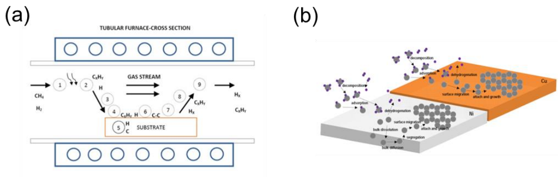
Figure 1.6 (a) schematic diagram of thermal CVD, (b) growth kinetics in CVD-produced graphene from CH 4 on Ni and Cu catalysts. [adapted from 62 ]
