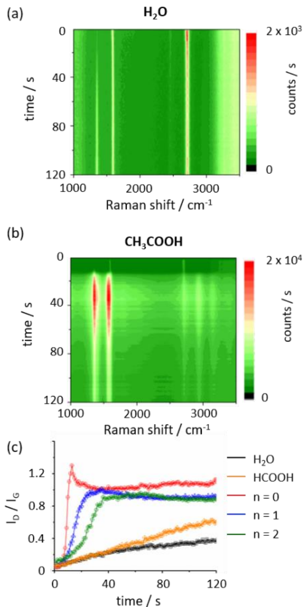
Figure 2.3 Time-course of Raman spectroscopy during the PICM. Waterfall plot of Raman spectra of graphene modified in \text{H}_2\text{O} (a) and acetic acid (b), respectively. (c) The intensity ratio between D and G bands ( I_D/I_G ) as a function of time for the PICM in \text{H}_2\text{O} (black), formic acid (orange), acetic acid ( n=0 ) (red), propionic acid ( n=1 ) (blue), and butyric acid ( n=2 ) (green), respectively.
