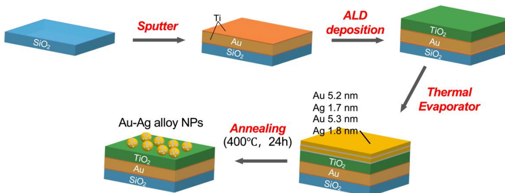
Figure 3.1 Schematic preparation of Au-Ag alloy NPs/ \text{TiO}_2 /Au-film (AATA) structure.
