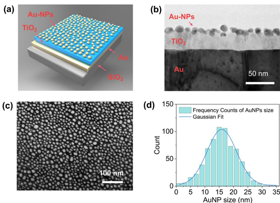
Figure 2.2 (a) Schematic of the ATA structure. (b) cross-section view STEM image of ATA structure, which consist of Au NPs, TiO 2 film (~30 nm) and Au-film. (c) SEM image of Au NPs on the ATA substrate. (d) Particle size distribution histogram and Gaussian fitting of Au NPs from the SEM image.
