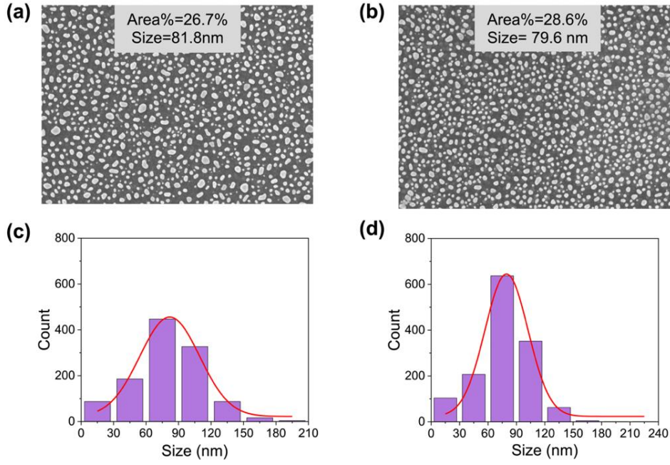
Figure 3.9 (a, b) SEM images of the Au-Ag alloy NPs on AATA (a) and AAT (b) structures in the top-view. (c, d) Size distributions (histogram and Gaussian fitting) from the SEM images of the Au-Ag alloy NPs on the AATA (c) and AAT (d) structures.
