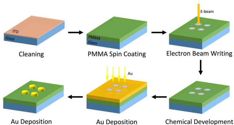
Figure 1.6 EB lithography technique used to fabricate Au nanostructures on an ITO glass substrate.
