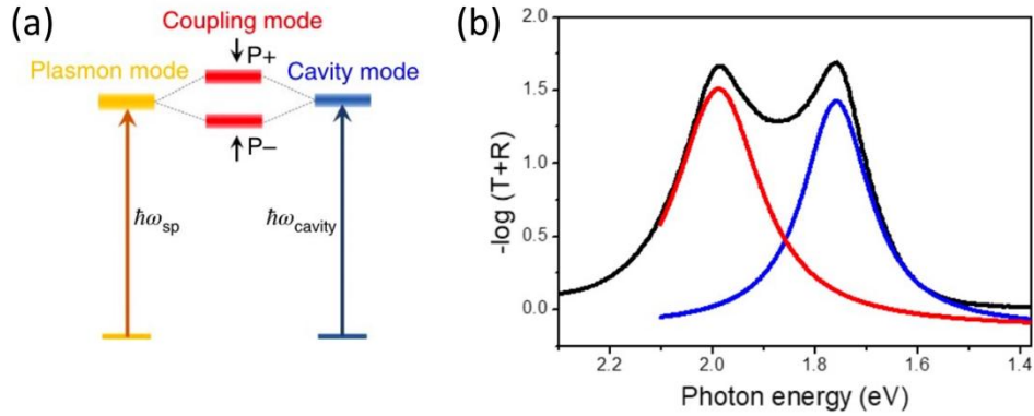
Figure 1.16 (a) Energy-level diagram of the strong coupling between the cavity mode in the \text{TiO}_2 film and the plasmon resonance of the Au NPs. The \omega_{sp} and \omega_{cavity} are the resonant frequencies of plasmon and FP nanocavity modes, respectively. (b) A representative absorption spectrum of the Au -NP/ \text{TiO}_2 /Au-film structure with an inlaid depth of 7 nm and its spectral separation by a Lorentz fitting.
