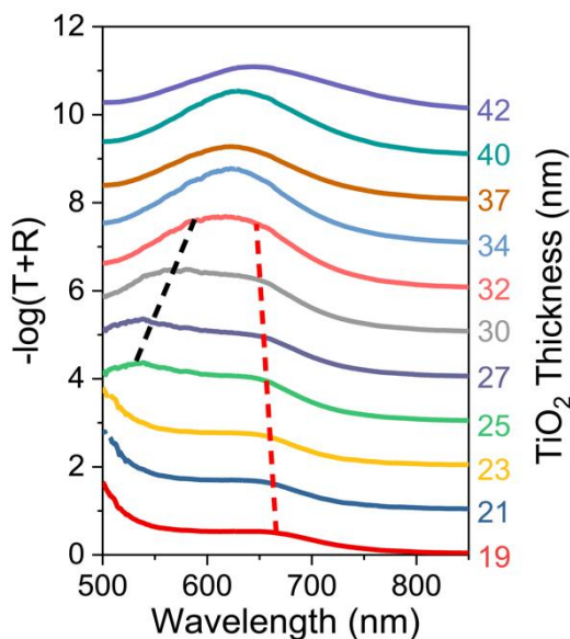
Figure 2.7 Absorption spectra calculated by -\log(T+R) of the ATA structure decorated by CV ( 10^{-6} mol/L) with various TiO 2 film thicknesses.
