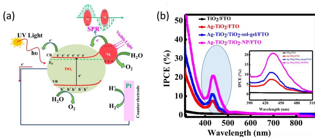
Figure 1.15 (a) Schematic diagram of the PEC water splitting mechanism by the Ag-TiO 2 -based
