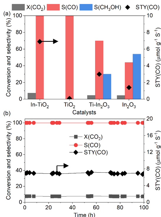
Figure 2. (a) Comparison of CO 2 hydrogenation activity of different catalysts. (b) Long term stability of In–TiO 2 during CO 2 hydrogenation. Reaction condition: 300 °C, 3 MPa, 30000 ml h -1 g -1 , H 2 :CO 2 = 3:1.
