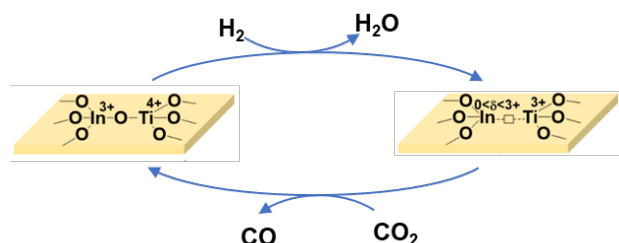
Scheme 1. Catalytic CO 2 hydrogenation to CO over In–TiO 2 catalyst through reverse Mars-van Krevelen pathway.
