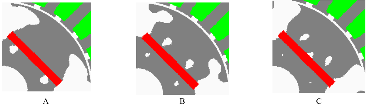
Fig. 6. Motor shapes corresponding to Pareto solutions A, B and C
