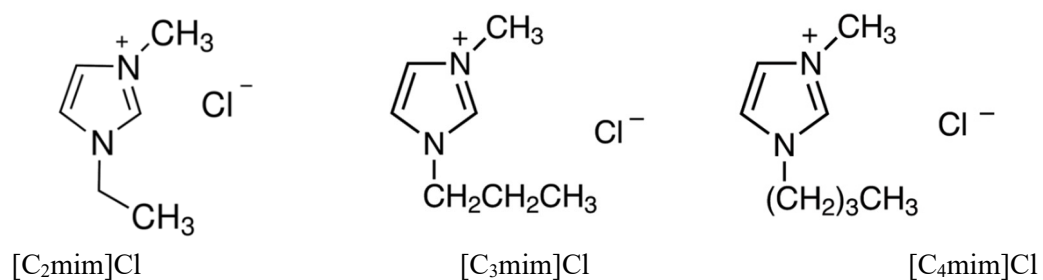
Fig. 1. Three ionic liquids used in the present work. [\text{C}_2\text{mim}]\text{Cl} (1-ethyl-3-methylimidazolium chloride), [\text{C}_3\text{mim}]\text{Cl} (1-methyl-3-propylimidazolium chloride), and [\text{C}_4\text{mim}]\text{Cl} (1-butyl-3-methylimidazolium chloride).
