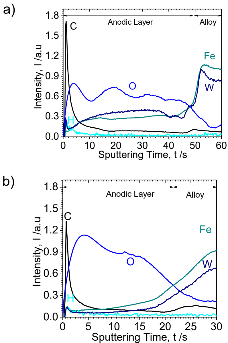
Figure 5.7 GDOES depth profiles of the anodic film grown on sputter-deposited Fe-W at 60 V anodizing in ethylene glycol containing 0.1 mol dm -3 NH 4 F, (a) 1.5 mol dm -3 H 2 O for 150 s and (b) 0.1 M H 2 O for 10 s, and annealed for 30 min under air exposure at 450 °C.
