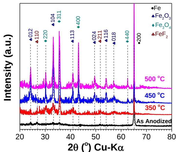
Figure 6.5 XRD patterns of the annealed and as-formed iron oxide microelectrodes formed at 60 V in ethylene glycol electrolyte containing 1.5 \text{ mol dm}^{-3} of water and 0.1 \text{ mol dm}^{-3} of \text{NH}_4\text{F} at 20^\circ\text{C} .
