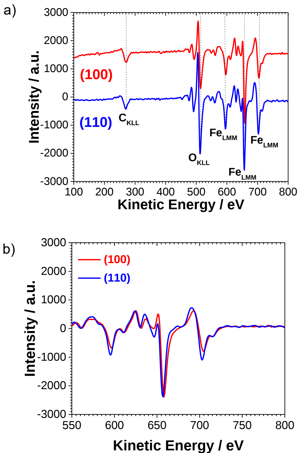
Figure 3.15 a) Wide Auger electron spectra and b) Fe_{LMM} spectra for anodic porous film formed on iron (100) and (110) single crystals anodized at 60 V for 900s in ethylene glycol electrolyte containing 1.5 \text{ mol dm}^{-3} of water and 0.1 \text{ mol dm}^{-3} of ammonium fluoride at 20^\circ\text{C} .
