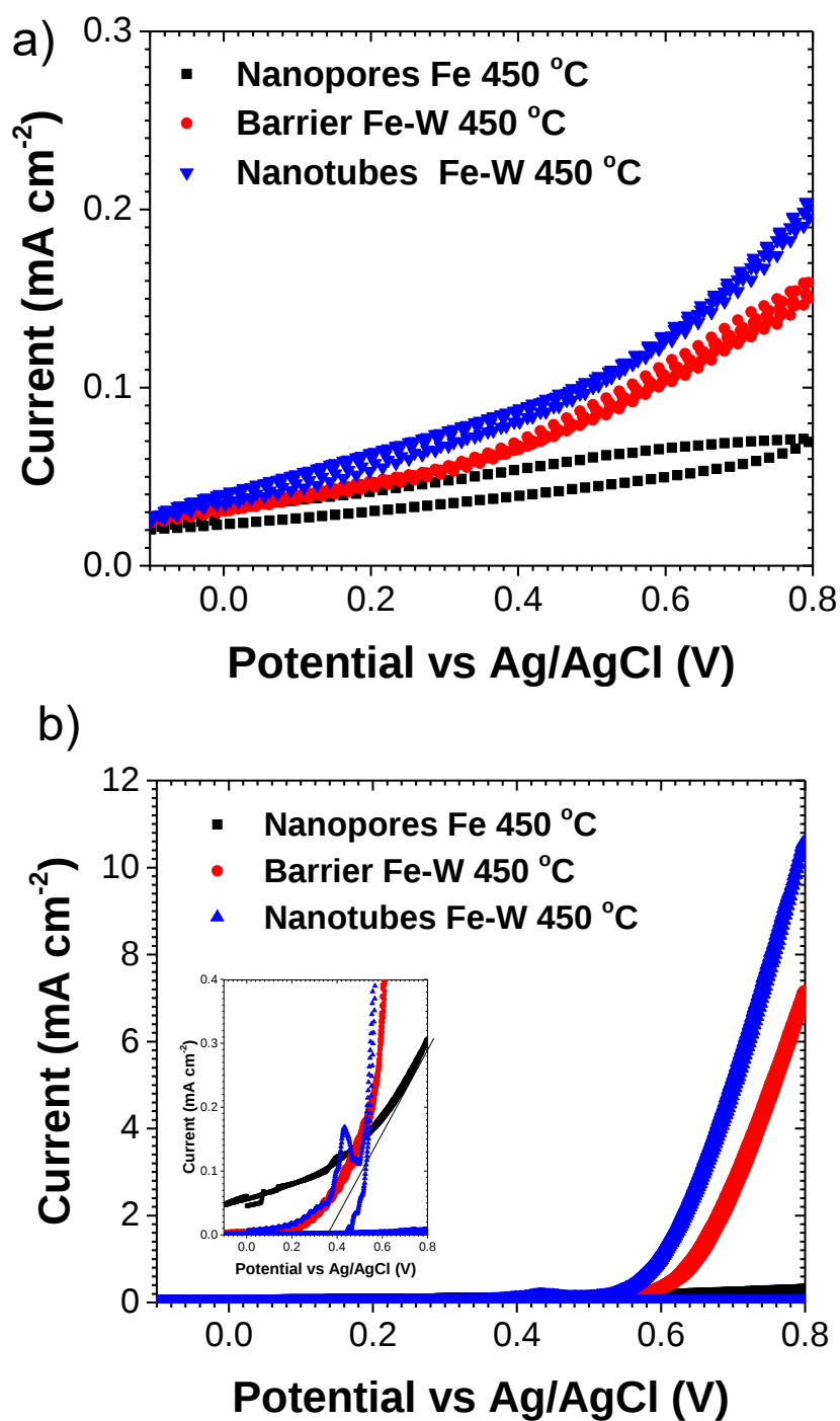
Figure 5.10 (a) Dark and (b) photo-current responses of the nanoporous film grown on Fe in ethylene glycol containing 0.1 mol dm -3 NH 4 F, 1.5 mol dm -3 H 2 O for 150 s, barrier film grown on Fe-W in ethylene glycol containing 0.1 mol dm -3 NH 4 F, 0.1 mol dm -3 H 2 O for 10 s, and nanotubes film grown on Fe-W in ethylene glycol containing 0.1 mol dm -3 NH 4 F, 1.5 mol dm -3 H 2 O for 150 s, and annealed for 30 min under air exposure at 450 °C.
