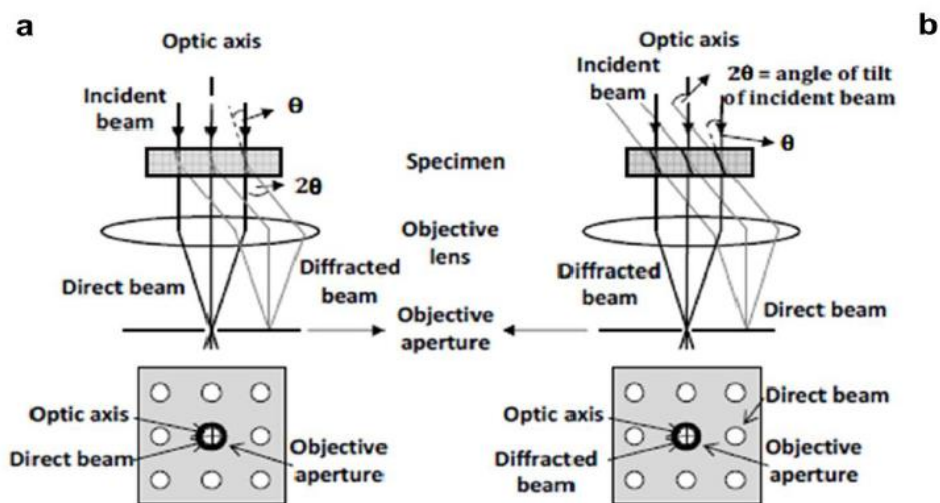
Figure 2.5 Condition for (a) bright- and (b) dark-field imaging [16].
