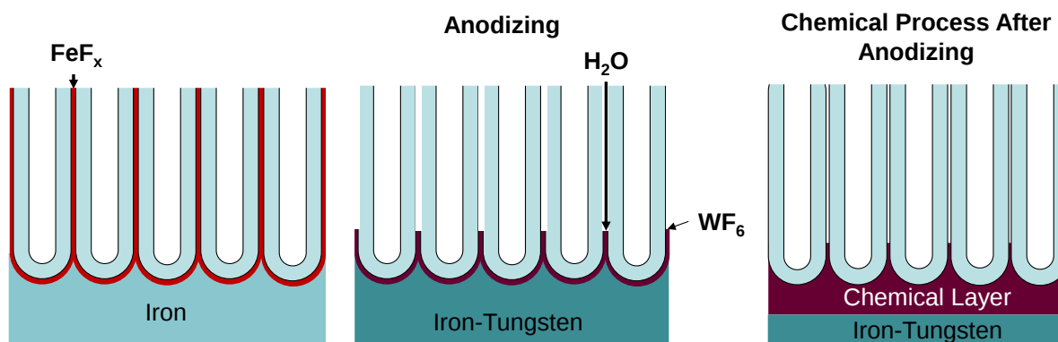
Figure 4.16 Schematic illustrations of anodic proposed growth mechanism for nanopores/nanotubes formed on a) iron, and b) iron tungsten alloy, c) illustrates post reaction with tungsten fluorides leading to formation of thick layer at metal/oxide interface.
