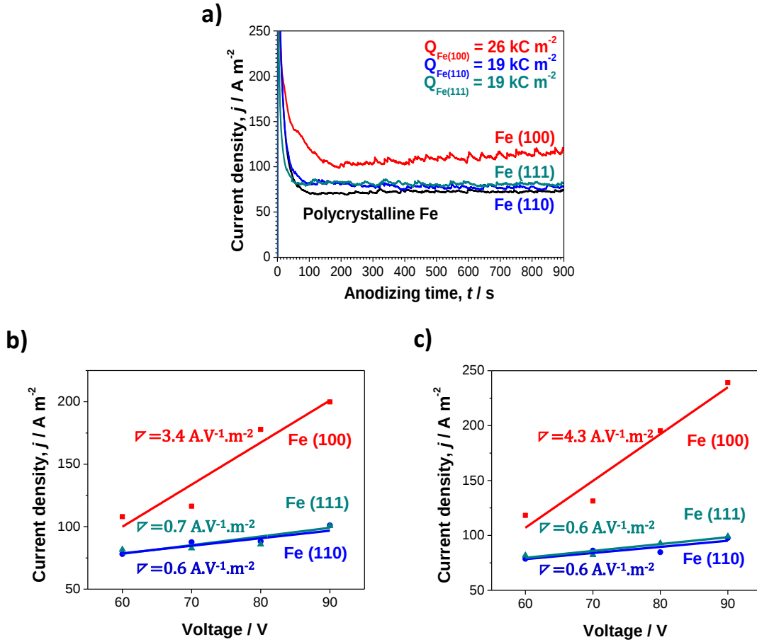
Figure 3.5 (a) Current-time ( j-t ) responses for poly crystalline, (100), (110) and (111) single crystal orientations of the iron substrates in an ethylene glycol electrolyte containing 1.5 mol dm -3 of water and 0.1 mol dm -3 of NH 4 F at 20°C at 60 V anodizing, and current-voltages correlation at (b) 450 s and (c) 900 s on anodizing Fe(100), Fe (110) and Fe(111) shown in panel (b) and (c).
