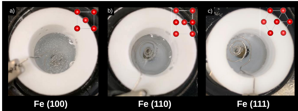
Figure 3.6 Oxygen evolution photos of three different single crystal orientations (a) Fe (100), (b) Fe (110), and (c) Fe (111) in an ethylene glycol electrolyte containing 1.5 \text{ mol dm}^{-3} of water and 0.1 \text{ mol dm}^{-3} of \text{NH}_4\text{F} at 20^\circ\text{C} .
