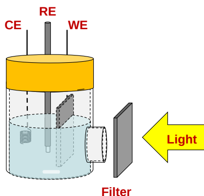
Figure 5.1 Schematic illustration of the photocurrent measurement.
