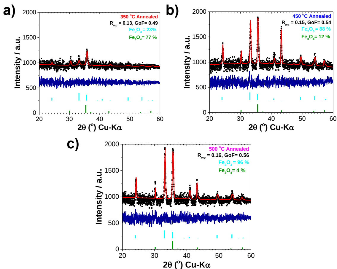
Figure 6.6 XRD refinement of the annealed iron oxide microelectrodes formed at 60 V in ethylene glycol electrolyte containing 1.5 \text{ mol dm}^{-3} of water and 0.1 \text{ mol dm}^{-3} of \text{NH}_4\text{F} at 20^\circ\text{C} after annealing at (a) 350^\circ\text{C} , (b) 450^\circ\text{C} and (c) 500^\circ\text{C} .
