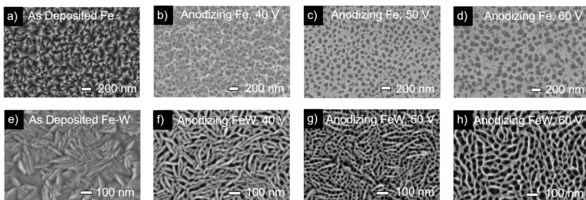
Figure 4.8 Surface morphology images for (a,e) as deposited Fe and Fe-W alloys, (b-d) Fe and (f-h) Fe-W (9 at.%) alloy anodized at 40-60 V in ethylene glycol electrolyte containing 1.5\text{ mol dm}^{-3} of water and 0.1\text{ mol dm}^{-3} of \text{NH}_4\text{F} at room temperature.
