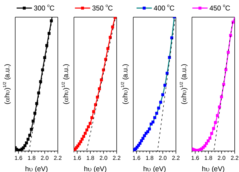
Figure 5.8 (a) UV-vis diffuse reflection spectra and (b) band gap estimate assuming indirect optical transition of the anodic film grown on sputter-deposited Fe-W at 60 V anodizing in ethylene glycol containing 0.1 \text{ mol dm}^{-3} \text{ NH}_4\text{F} , 0.1 \text{ mol dm}^{-3} \text{ H}_2\text{O} for 10 s and annealed for 30 min under air exposure at varying temperature.
