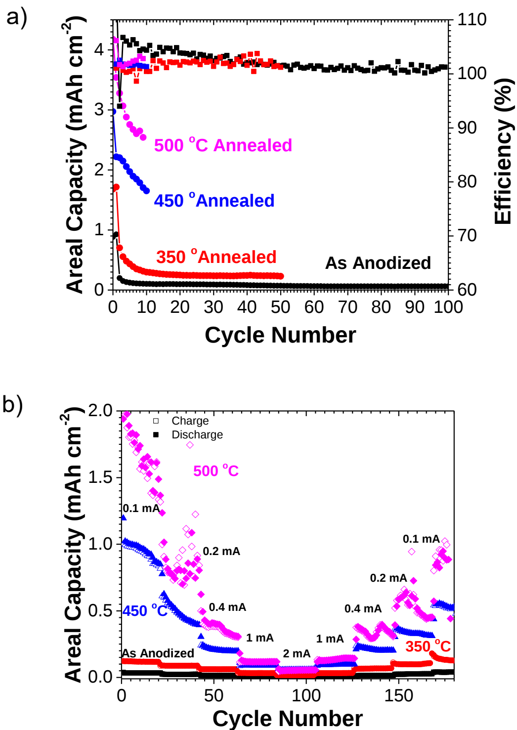
Figure 6.10 (a) Plot of capacity vs. cycle number and columbic efficiency of microelectrodes iron oxide in 1 \text{ mol dm}^{-3} \text{ LiPF}_6 \text{ EC:DMC } 1:1 at constant current density 20 \mu\text{A cm}^{-2} and (b) rate capability for iron oxide in 1 \text{ mol dm}^{-3} \text{ LiPF}_6 \text{ EC:DMC } 1:1 at different current densities from 0.04 to 2 \text{ mA cm}^{-2} .
