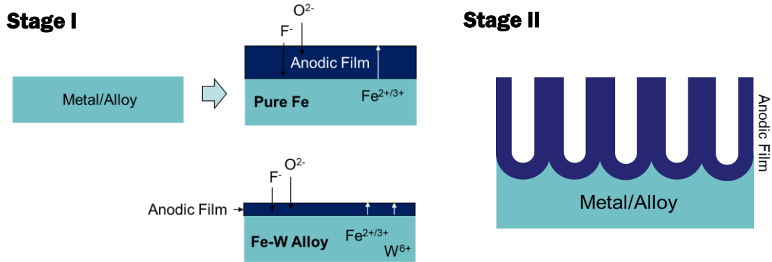
Figure 4.6 Schematic illustration of the growth mechanism of anodic Fe and Fe-W during stage I and Stage II.
