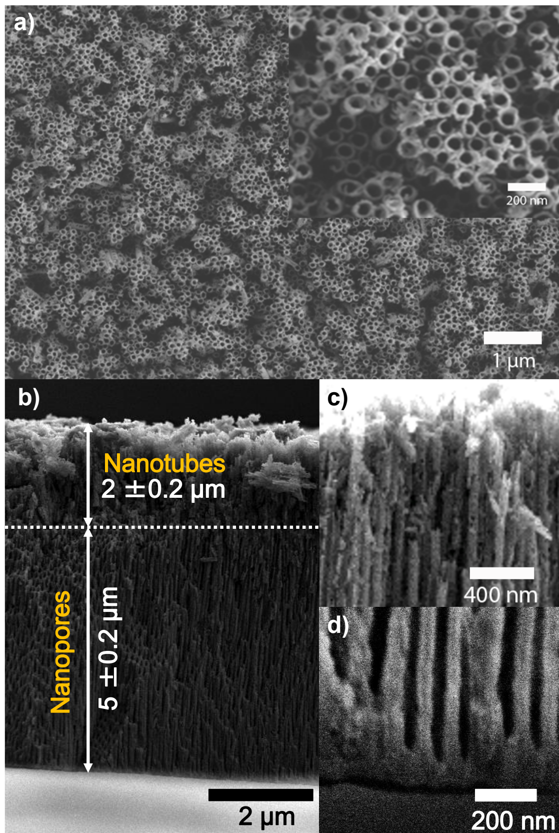
Figure 6.3 (a) Surface morphology and (b) cross-section SEM images obtained by SE mode at 3 kV; of nanopores/nanotubes formed by anodizing of Fe at 60 V in ethylene glycol electrolyte containing 1.5 mol dm -3 of water and 0.1 mol dm -3 of NH 4 F at 20 °C, detail of nanotubular formation on top part and nanoporous formation on bottom part shown on (c) and (d).
