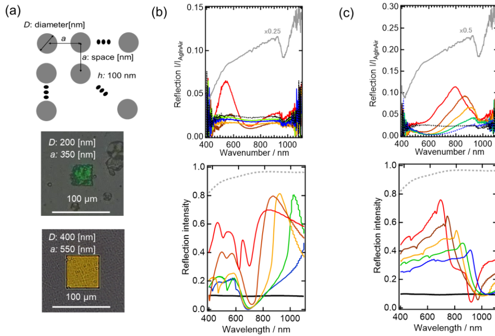
Figure 5-5. (a) Design and optical images of plasmonic disk lattices with different disk diameter ( D ) and lattice spacing ( a ). (b) Experimental reflection spectra of Ag disk grating of (b) D=200 nm with a=300, 350, 400, 450, 500 nm and (c) D=400 nm with a=500, 550, 600, 650, 700 nm are shown as reflection ratio to Ag mirror reference in air. In figure (b), red, brown, orange, green, and blue lines represent the spectra of a=300, 350, 400, 450, and 500 nm, respectively. In figure (c), the red, brown, orange, green, and blue lines represent the spectra of a=500, 550, 600, 650, and 700 nm, respectively. The gray line and black dashed lines correspond to Ag 100 nm films and GC 100 nm layer. All spectra are obtained in 0.5 M \text{NaClO}_4 aq. under 75 MPa. Bottom panels show FDTD calculations of each disk spacing with Ag and GC in the same manner as the experimental spectra.
