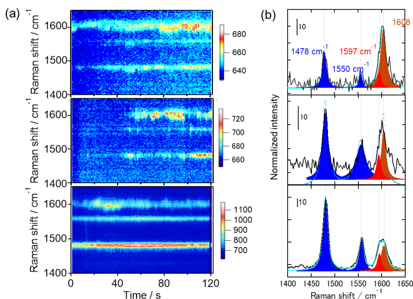
Figure 3-15. 2D-expression of time series SERS spectra of 1\text{ }\mu\text{M} 44bpy + 0.1\text{ M} NaClO 4 aq. at -0.8\text{ V} vs. Ag/ AgCl. 1608\text{ cm}^{-1} (assigned for 44bpy) as red solid line, 1480\text{ cm}^{-1} (assigned for 22bpy) as a blue broken line. t_{ex} : 60 s, I_{ex} : 35, 70, 140\text{ }\mu\text{W }\mu\text{m}^{-2} from top to bottom. (b) Normalized SERS spectra by incident laser intensity collected at laser illumination time of 100 s. Lorentz fitting peaks at 1608 and 1597\text{ cm}^{-1} are represented as brown and red areas(44bpy). The fitting peaks at 1478 and 1550\text{ cm}^{-1} (22bpy) are shown as blue. Light blue dots show total fitting area of these fitting peaks.
