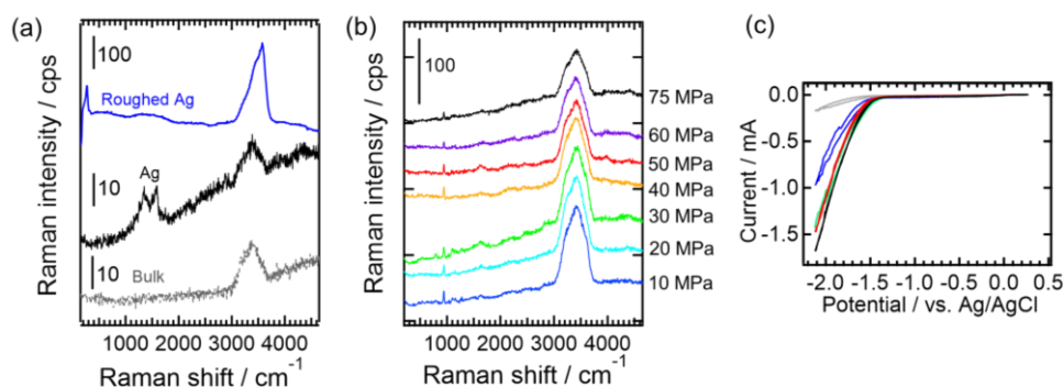
Figure 4-4. (a) Raman spectra of 0.1\text{ M NaClO}_4 aq. were taken in solution, on Ag surface, and on roughened Ag surface, respectively, under 30\text{ MPa } t_{\text{ex}}: 10\text{ s} . (b) SERS spectra with variety of static pressure of \text{H}_2\text{O } 0.5\text{M NaClO}_4 aq. were obtained at -1.42\text{V vs. Ag/AgCl} in t_{\text{ex}}: 10\text{ s} . The static pressure was kept as 10, 20, 30, 40, 50, 60, and 75 MPa from bottom to top. (c) The cyclic voltammogram of 0.5\text{M NaClO}_4 aq. ( \text{H}_2\text{O} ) on roughened Ag are taken with 100\text{ mV/s} under different pressured condition, as 0.1 10, 25, 50, and 75 MPa from top to bottom.
