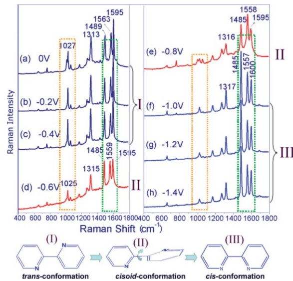
Figure 1-9. Orientation and SERS spectra of 22BPY molecules on a Ag-coated Ag electrode depend on potential (20 \mu L volume of 22BPY solution rapidly added onto the electrode surface and dried fully before adding the ice-cold KCl solution, 0.1 M, 0 ^{\circ} C). 90
