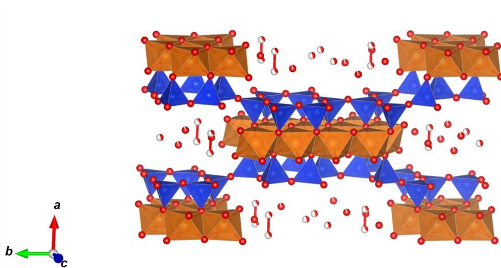
Fig. 1.14. Crystal structure of sepiolite (TOT ribbons)
