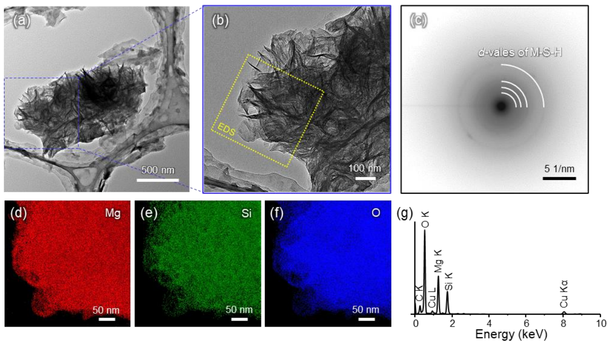
Fig. 5.10. TEM analysis of solid sample from the [\text{Si}]_{\text{in}} 0.15 mM experiment. (a) TEM image of representative particles; (b) high-magnification image of the area selected in (a); (c) electron diffraction pattern; (d–f) Mg, Si, and O distributions in the area selected in (b); (g) EDS spectrum of the area selected in (b).
