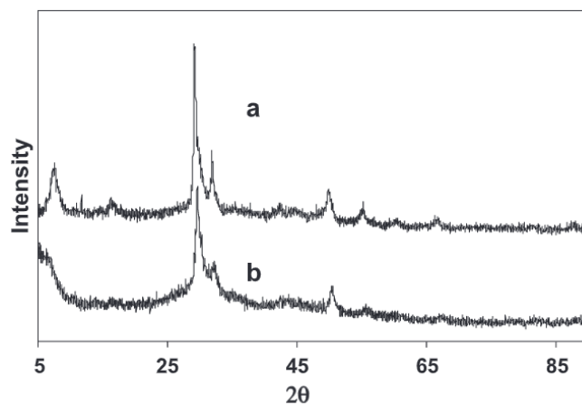
Fig. 1.8. XRD patterns (Cu K \alpha ) of C-S-H obtained (a) in diluted suspension from a mix of CaO and SiO 2 and (b) by hydration of a mix of fine tricalcium silicate (C 3 S) and SiO 2 in paste (Nonat, 2004).
