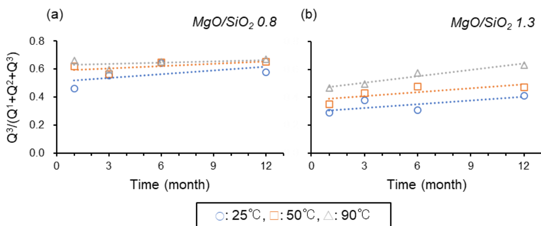
Fig. 3.7. Variation in Q^3/(Q^1+Q^2+Q^3) ratios as a function of time for the M-S-H samples from (a) \text{MgO/SiO}_2 0.8 and (b) \text{MgO/SiO}_2 1.3. The dotted lines represent least squares regression lines.
