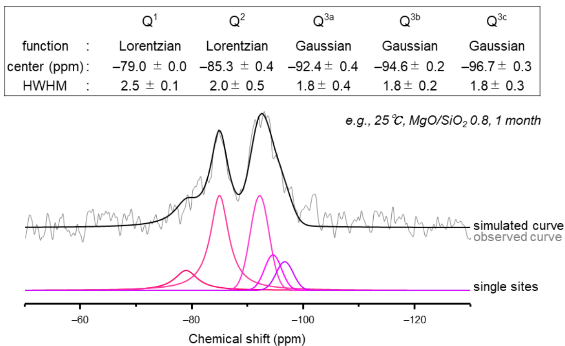
Fig. 3.6. Functions, peak positions, and half width at half maximum (HWHM) in the deconvolution of the ^{29}\text{Si} MAS NMR spectra in this study.
