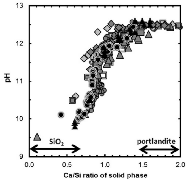
Fig. 1.7. Relation between solid Ca/Si ratio and pH in the C-S-H syntheses (Lothenbach and Nonat, 2015).
