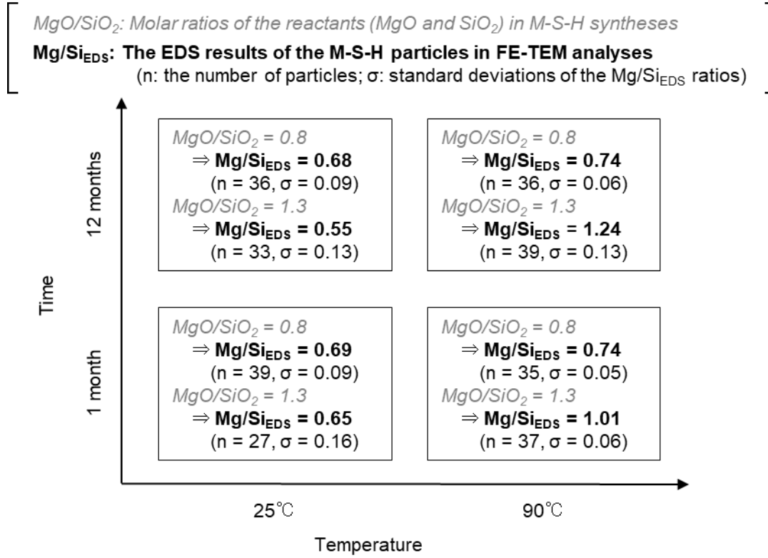
Fig. 3.13. Average Mg/Si molar ratios of M-S-H particles formed at 25°C and 90°C for 1 month and 12 months.
