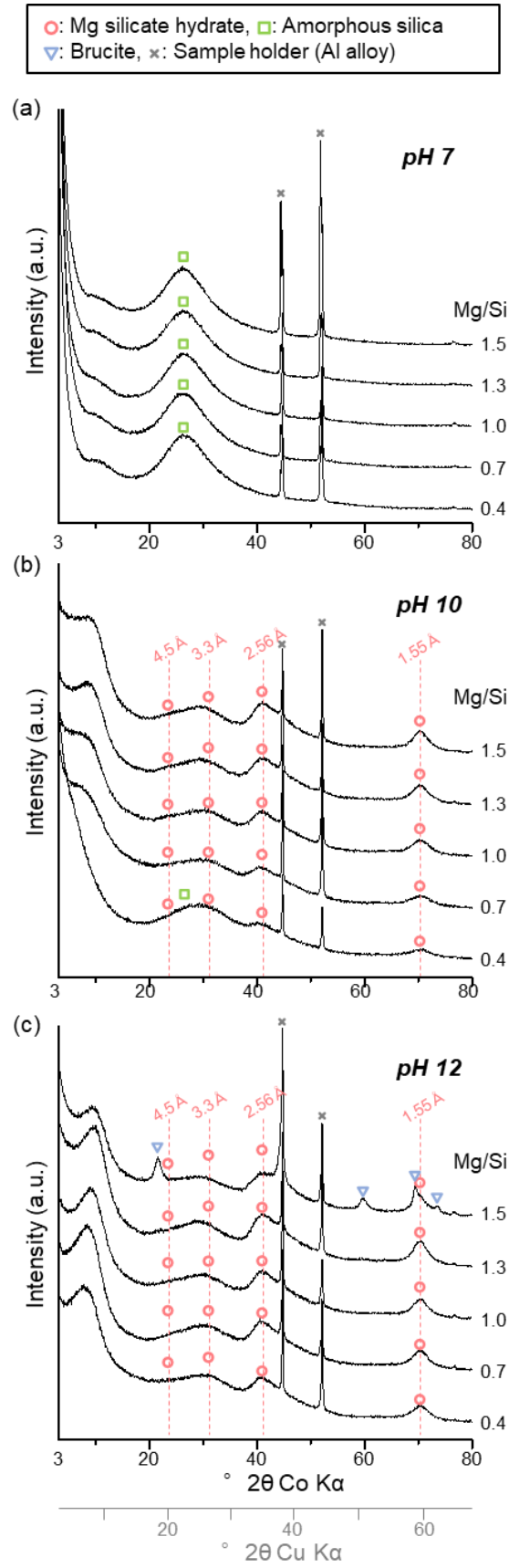
Fig. 4.1. XRD patterns of precipitates in Mg–Si–H 2 O systems at (a) pH 7, (b) pH 10, and (c) pH 12.
