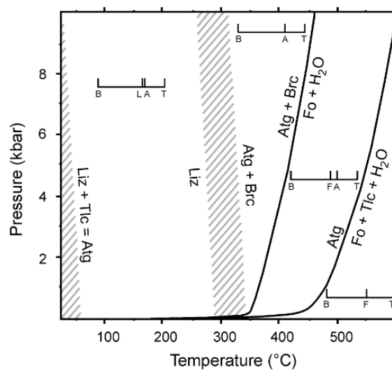
Fig. 1.1. Stable phase diagram in the system Mg–Si–H 2 O proposed by Evans (2004). The shades show uncertain areas. Atg: antigorite; Brc: brucite; Fo: forsterite; Liz: lizardite; Tlc: talc.
