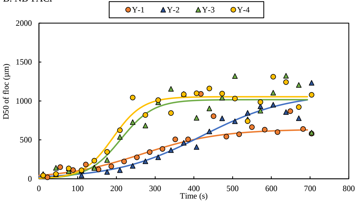
Fig. 3-3. Change of D50 of floc particles in coagulation experiments using HB-PACl (Panel A) and NB-PACl (Panel B). Particle size measurements were conducted every 10 s, and the average value of triplicate measurements is shown (plots). The lines are the fits to the semi-empirical model equation proposed by Chassagne (2021). The time until the D50 of floc particles grew to 500 \mu\text{m} was determined from the model-fit lines. Y series waters (Y-1–4) were used in these experiments. The PACl dose was 2.5 mg-Al/L. The coagulation pH was 7.0.
