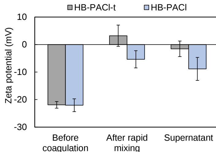
Fig. 2-12. Change of zeta potential during CSF experiment. Water C-1 was used. Initial SPAC concentration was 2 mg/L. HB-PACI-t and HB-PACI were used at a dosage of 2.5 mg-Al/L. Coagulation pH was 7.0.
