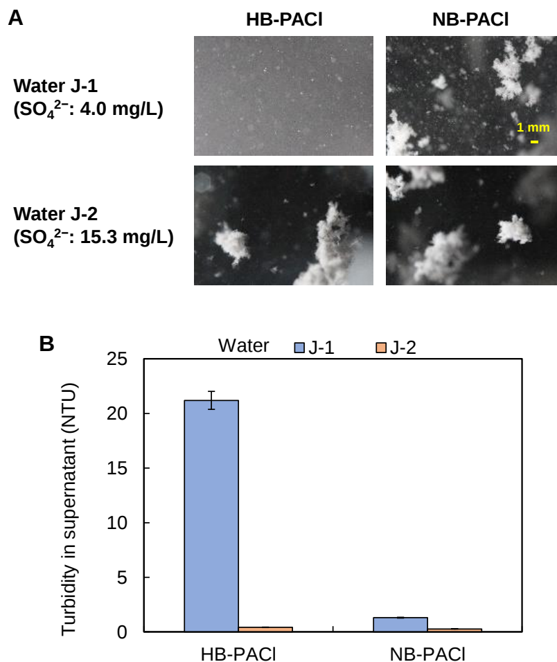
Fig. 2-23. Photographs taken at the end of slow mixing 3 (Panel A) and residual turbidities of supernatants (Panel B). Waters J-1 and J-2 with different sulfate ion concentrations of 4.0 and 15.3 mg/L, respectively, were used. Initial SPAC concentration was 2 mg/L. HB-PACl and NB-PACl were used at a dosage of 4.0 mg-Al/L. Coagulation pH was 7.0.
