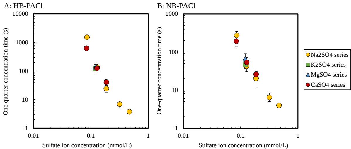
Fig. 4-3. Plots of one-quarter concentration times against sulfate ion concentrations with different counter cations. Panel A shows the data for HB-PACl in Na 2 SO 4 -1–4,6 and CaSO 4 -1,3,4 waters. Panel B shows the data for NB-PACl in Na 2 SO 4 -2–4 and CaSO 4 -1,3,4 waters. The PACl dose was 2.5 mg-Al/L. The coagulation pH was 7.0. Error bars indicate 95% confidence intervals.
