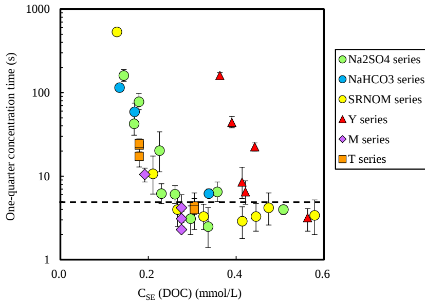
Fig. 4-11. One-quarter concentration times versus C_{SE} values, where DOC was used instead of UV260 for the NOM concentration. Panel A shows the data for HB-PACl in Na 2 SO 4 -1,2,4,6,8–13, NaHCO 3 -3,5,6, SRNOM-3–10, Y-1–6, M-1,2, and T-1,2 waters, and Panel B shows the data for NB-PACl in Na 2 SO 4 -1,2,4,6,8–13, NaHCO 3 -1,5,7, SRNOM-2–9, Y-1–6, M-1,2, and T-1,2 waters. The PACl dose was 2.5 mg-Al/L, but doses of 1.5 and 3.5 mg-Al/L were also used in the experiments with M-1,2 and T-1,2 waters. The coagulation pH was 7.0. Error bars indicate 95% confidence intervals.
