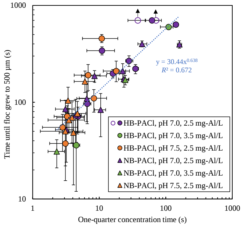
Fig. 3-12. Relationship between the time until floc grew to 500 μm and one-quarter concentration times in coagulation experiments. The results for HB-PACl and NB-PACl at pHs of both 7.0 and 7.5 are shown. Y-1–6, M-1,2, and T-1,2 waters were used in these experiments. Results for PACl doses of 2.5 and 3.5 mg-Al/L are shown. Open circles indicate that floc size did not grow to 500 μm during flocculation. Error bars indicate 95% confidence intervals.
