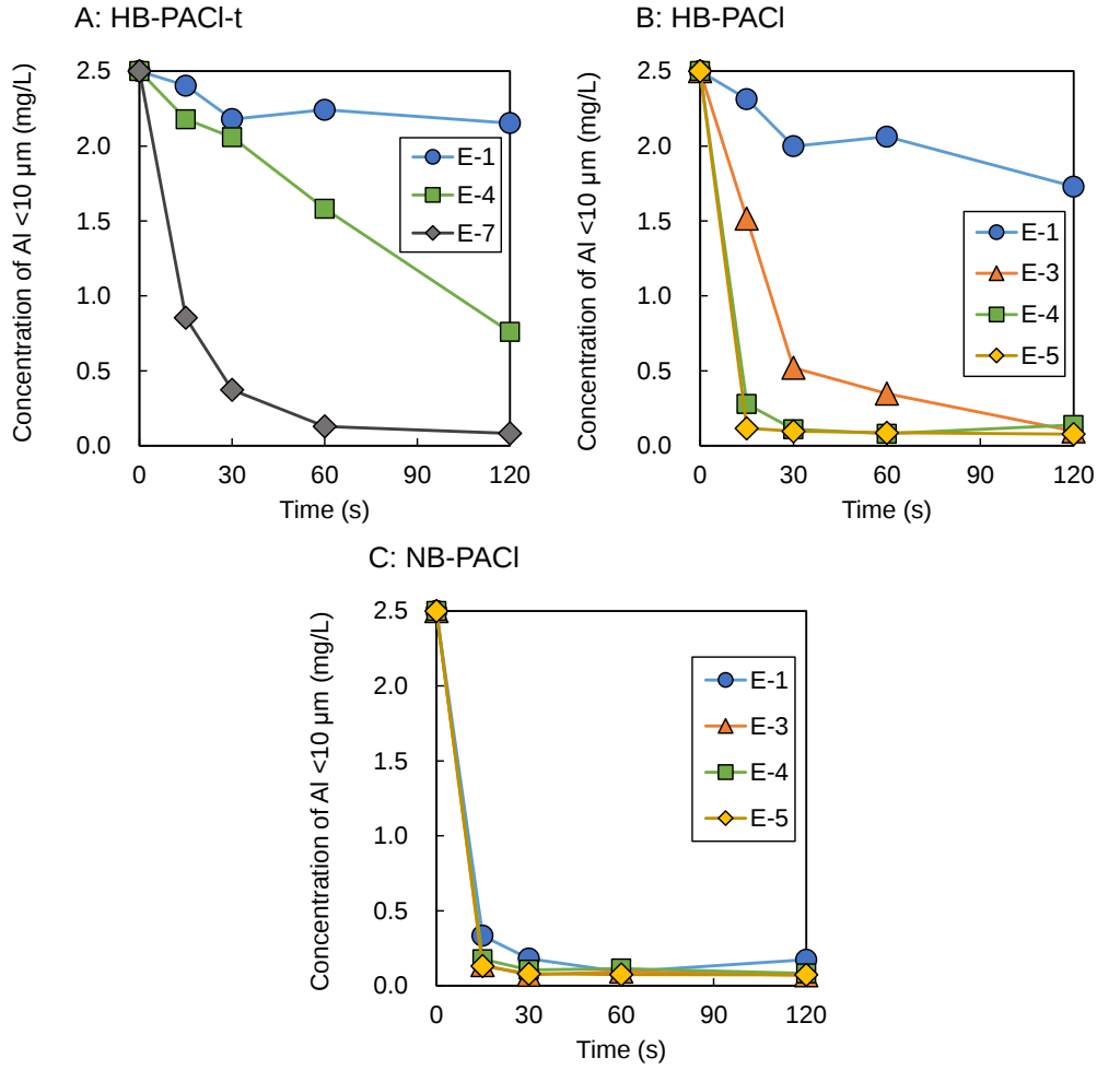
Fig. 2-24. Change of concentration of aluminum that passed through a membrane with a 10- \mu\text{m} pore size. Waters E-1, E-3, E-4, E-5, and E-7 with sulfate ion concentrations of 0.0, 6.4, 15.8, 15.7, and 48.8 mg/L, respectively, were used. HB-PACI-t (Panel A), HB-PACI (Panel B), and NB-PACI (Panel C) were dosed at 2.5 mg-Al/L. pH during mixing was 7.
