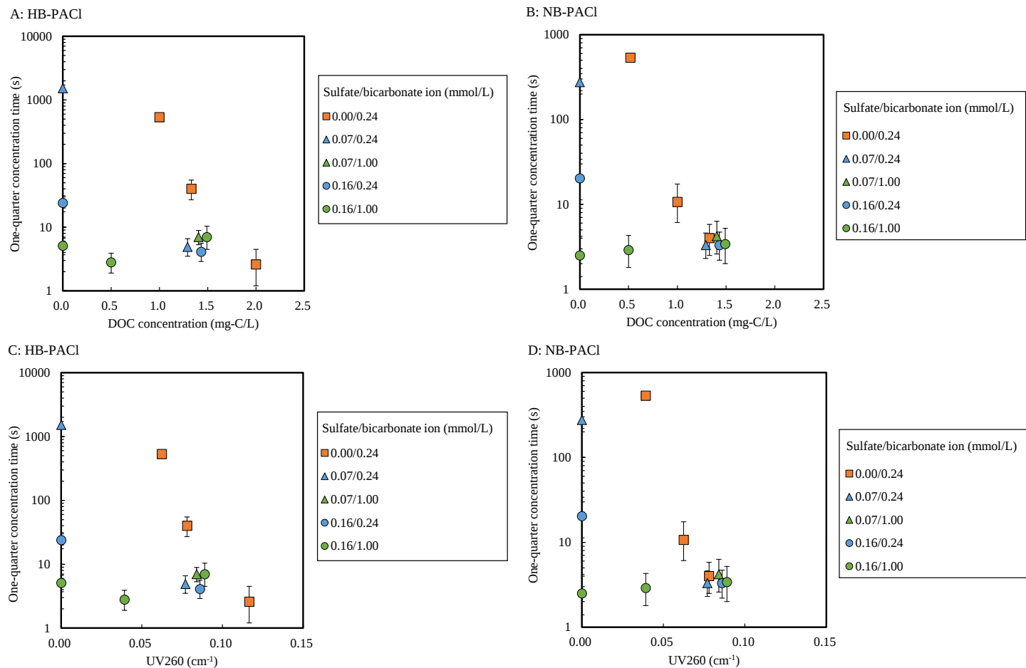
Fig. 4-9. One-quarter concentration times for various concentrations of NOM (DOC in Panels A and B, UV260 in Panels C and D), sulfate ions, and bicarbonate ions. Panels A and C; HB-PACl was used in SRNOM-3–5,7–10 and Na 2 SO 4 -2,3,6,8 waters. Panel B and D: NB-PACl was used in SRNOM-2–5,7–9, and Na 2 SO 4 -2,3,6,8 waters. The coagulation pH was 7.0. The PACl dose was 2.5 mg-Al/L. Numerical values in the legends indicate the concentrations of sulfate ion and bicarbonate ion. Error bars indicate 95% confidence intervals.
