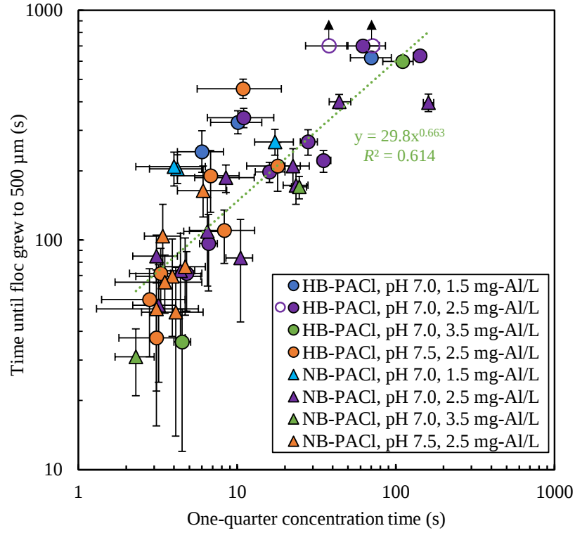
Fig. 3-11. Relationship between the time until floc grew to 500 µm and one-quarter concentration times in coagulation experiments. The results for HB-PACl and NB-PACl at pHs of both 7.0 and 7.5 are shown. Y-1–6, M-1,2, and T-1,2 waters were used in these experiments. Results for PACl doses of 1.5, 2.5, and 3.5 mg-Al/L are shown. Open circles indicate that floc size did not grow to 500 µm during flocculation. Error bars indicate 95% confidence intervals.
