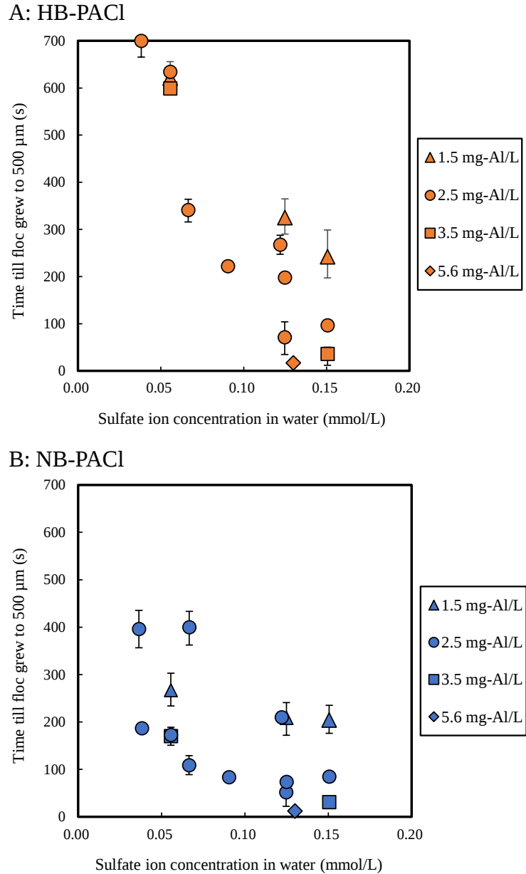
Fig. 3-8. Plots of the time till floc grew to 500 \mu\text{m} against sulfate ion concentration in water. Panels A and B show the data for HB-PACl and NB-PACl respectively. Y-1-6, M-1,2, T-1,2, and S-1 water were used. The coagulation pH was controlled at 7.0. Error bars indicate 95% confidence intervals.
