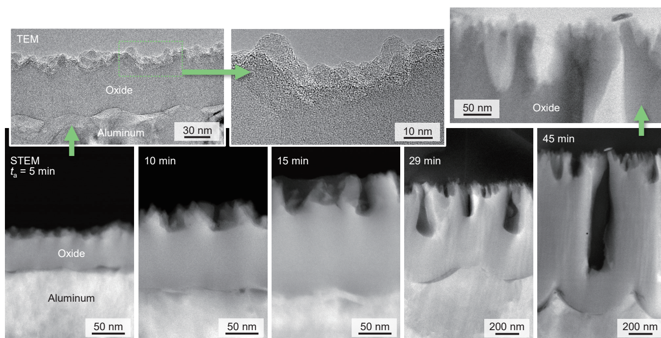
Figure 2-3. STEM images of the cross-section of the specimen anodized at 5.0 \text{ Am}^{-2} for 5-45 min. High-magnification TEM images of the anodized specimens for 5 min and 45 min are also described in the upper part.
