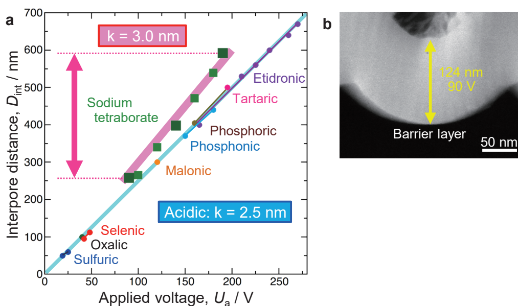
Figure 6-4. (a) Linear relationships between the applied voltage, U_a , and the interpore distance of the self-ordered porous alumina, D_{int} , formed by anodizing in conventional acidic electrolyte solutions. (b) An HAADF-STEM image of the ultrathin section of the bottom barrier layer formed by anodizing at 90 V.
