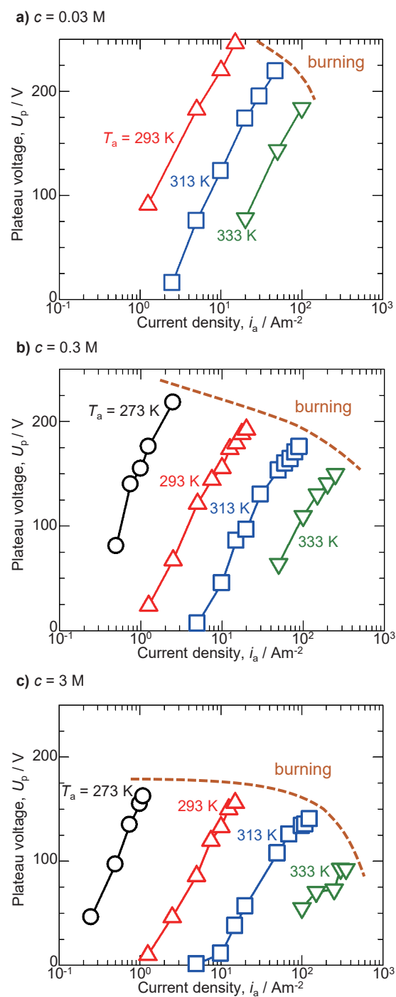
Figure 3-2. Changes in the plateau voltage, U_p , with the current density, i_a , during galvanostatic anodizing in a) 0.03 M, b) 0.3 M, and c) 3 M etidronic acid solutions at 273-333 K.
