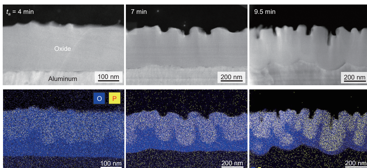
Figure 2-8. STEM images of the cross-section of the specimen anodized at 20.0 Am -2 for 4-9.5 min and the corresponding elemental mapping images of oxygen and phosphorus.
