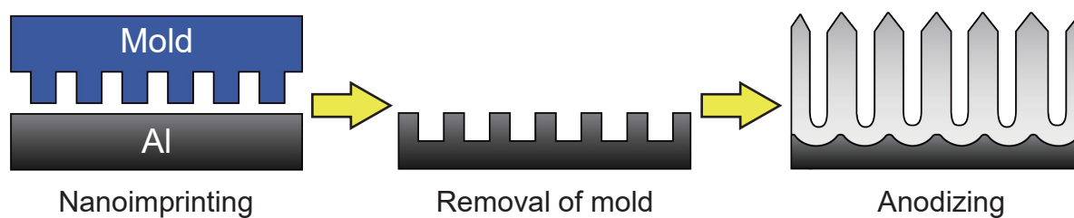
Figure 1-3. Schematic diagrams of a) two-step anodizing and b) Nanoimprinting methods.
