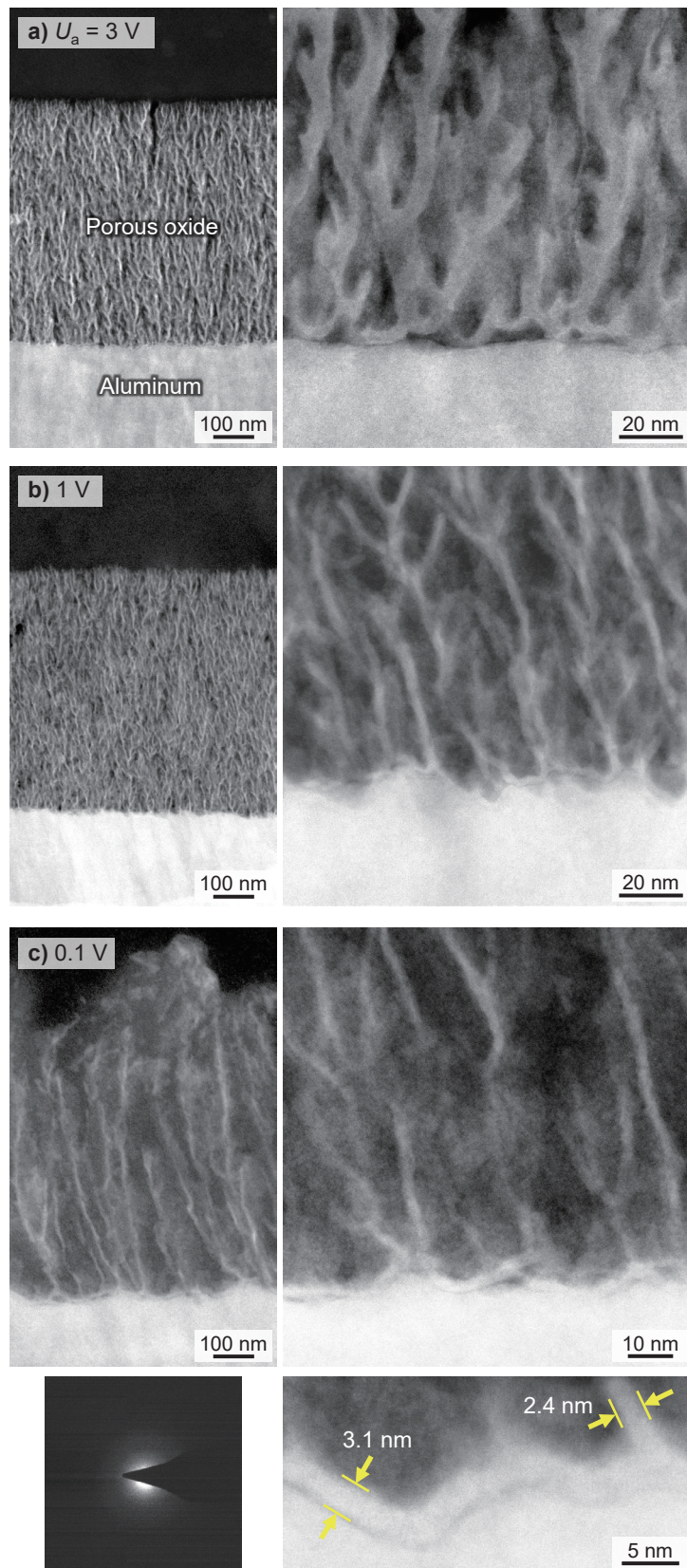
Figure 5-9. Low- and high-magnification HAADF-STEM images of the porous alumina formed by anodizing in a 0.3 M sodium metaborate solution at 278 K and a) 3, b) 1, and c) 0.1 V. A corresponding diffraction pattern of the anodic oxide formed at 0.1 V is shown in c).
