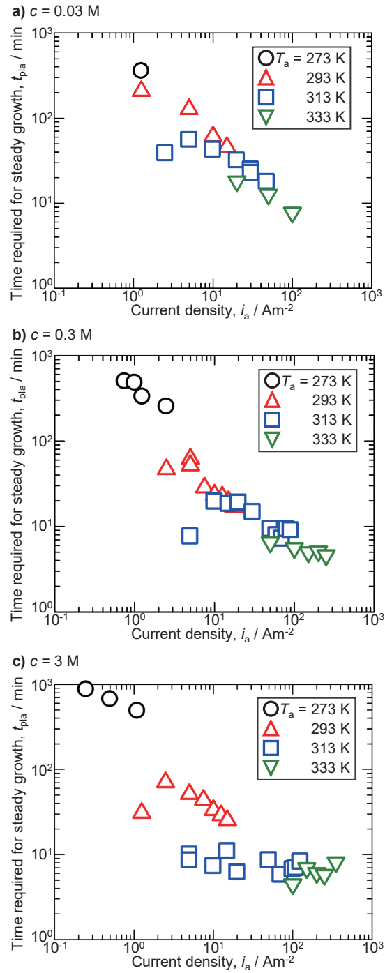
Figure3-3. Changes in the time to reach the plateau voltage, t_{\text{pla}} , with the current density, i_a , during galvanostatic anodizing in a) 0.03 M, b) 0.3 M, and c) 3 M etidronic acid solutions at 273-333 K.
