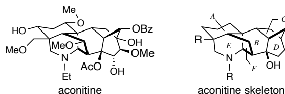
Figure 3.1 Aconitine-type C 19 -Diterpenoid Alkaloids
