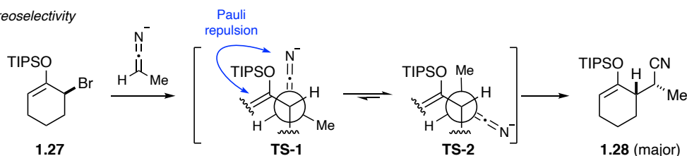
Scheme 1.10 Intermolecular Alkylation
