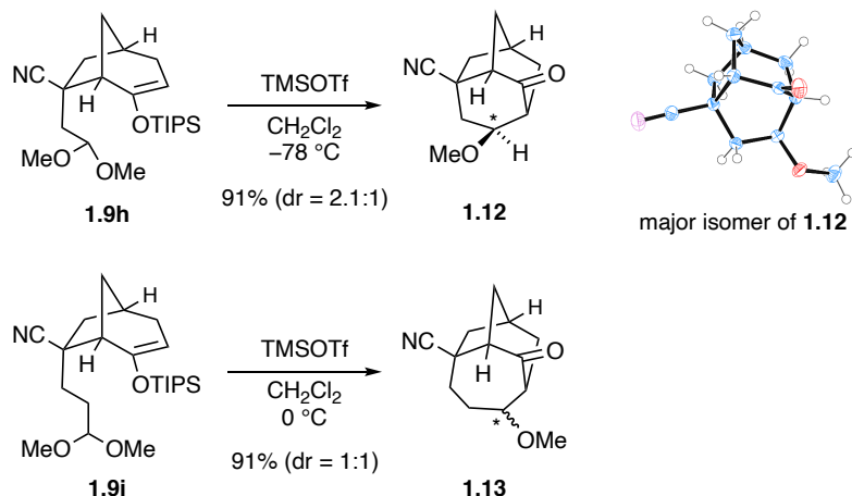
Scheme 1.5 Construction of Caged Skeletons
