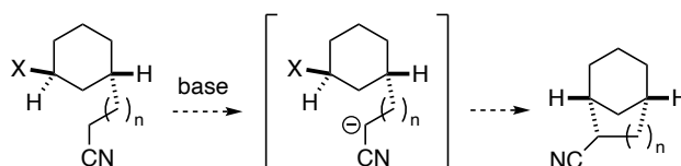
Scheme 10 S_{Ni} Displacement on the Carbocycle
