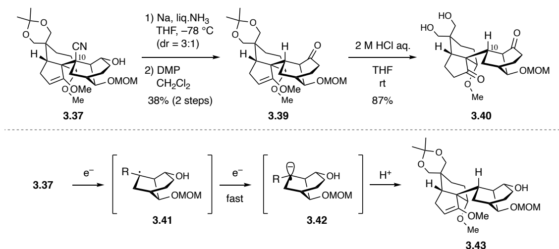
Scheme 3.13 Reductive Decyanation of Tetracyclic Compound
