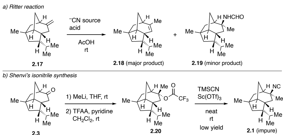
Scheme 2.7 Attempts for Isocyanation at C2-position
