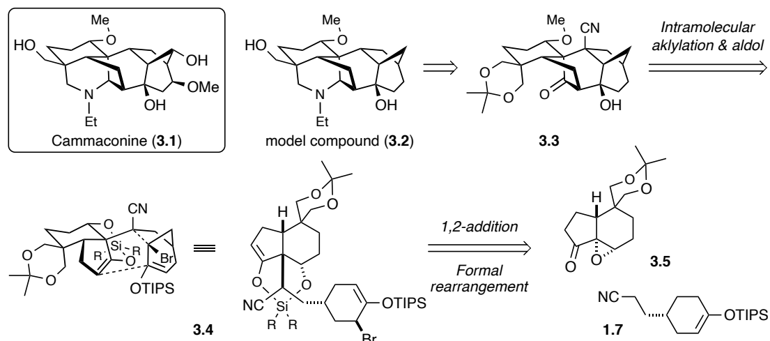
Scheme 3.5 Retrosynthetic analysis
