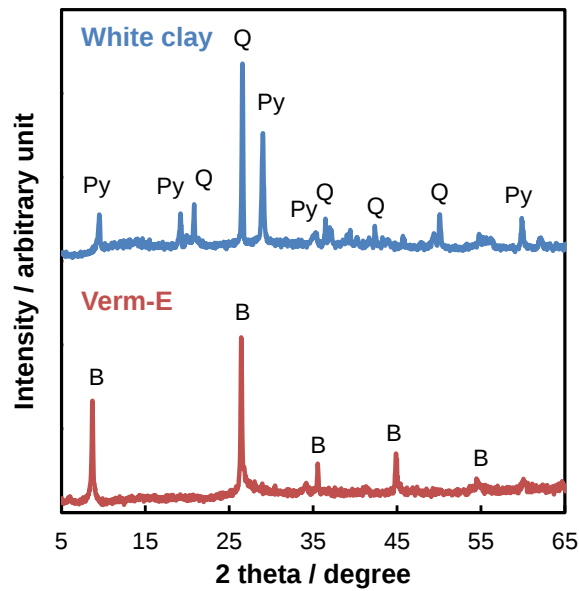
Fig. 5-2. X-ray diffractograms of white clay and Verm-E. Py: Pyrophyllite, Q: Quartz, B: Biotite.
