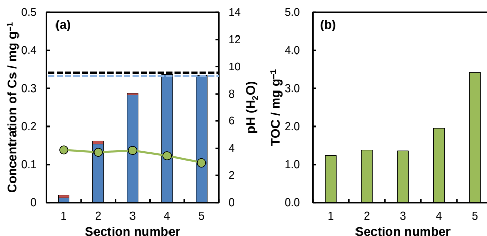
Fig. 6-4. Distribution of (a) Cs and pH (green line), and (b) TOC in model contaminated soil after the EK process for 72 h. The contaminated soil was leached with 0.5 mol/L oxalic acid for 2 weeks before the EK process. The black and blue dashed lines indicate the total initial concentration of Cs and the initial concentration of Cs in ion exchangeable form. The blue and red bars indicate the concentration of Cs in ion exchangeable form and residual form.
