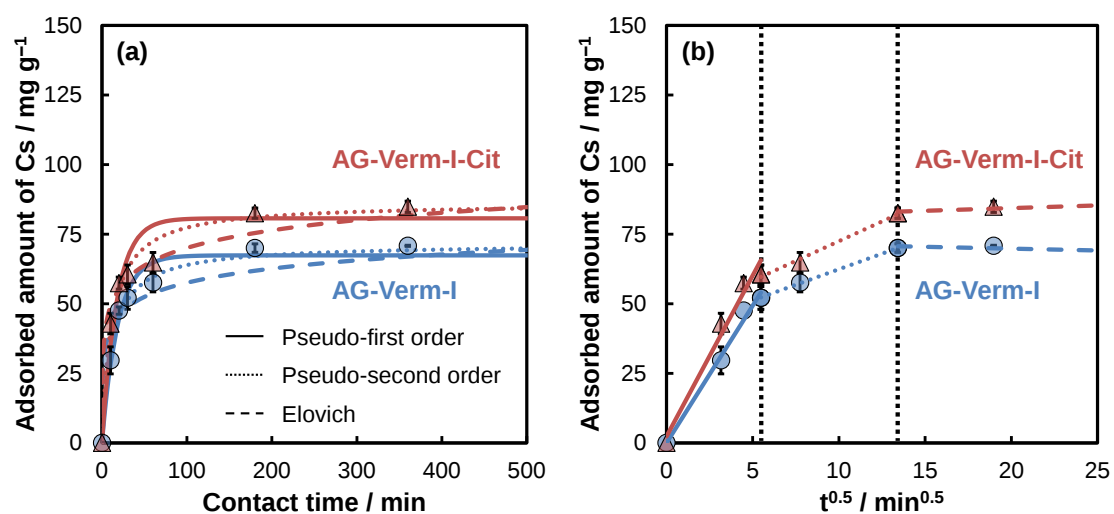
Fig. 4-13. (a) Adsorbed amount of Cs by alginate gel vermiculite (AG-Verm) beads and alginate gel sodium citrate-pretreated vermiculite (AG-Verm-Cit) beads in each contact time, and (b) the linearized plot for IPD kinetics model. The concentration of Cs was 500 mg/L (pH 6.0); the temperature was 25 °C; the adsorbent dose was 25 beads in 25 mL. Error bars indicate the standard deviation ( n = 3 ).
