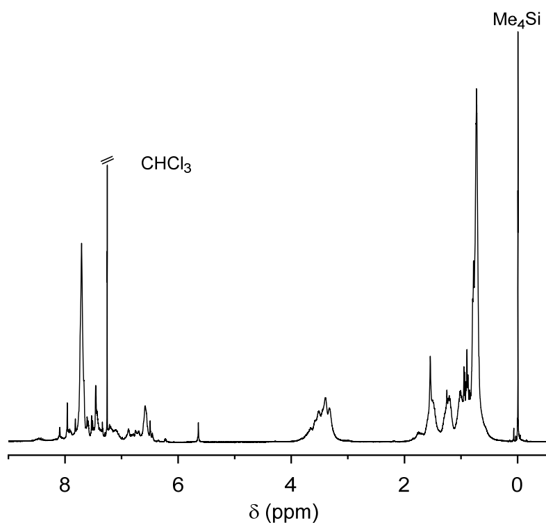
Figure 2-15. ^1\text{H} NMR spectrum of poly(3-alt-6). [400 MHz, \text{CDCl}_3 , r.t.].
