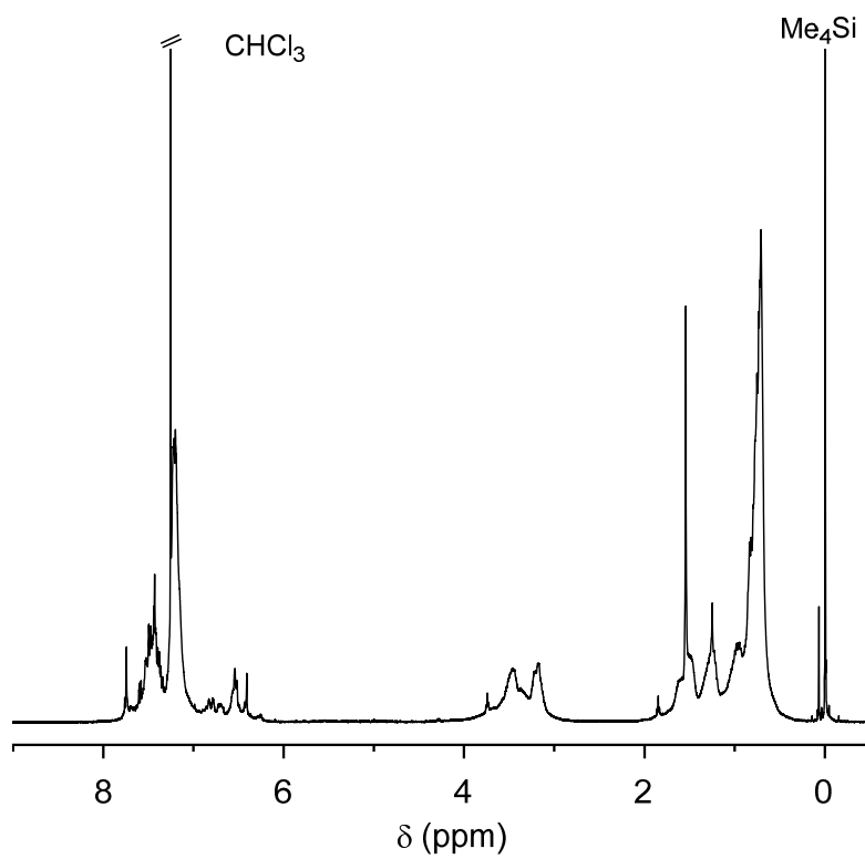
Figure 2-13. ^1\text{H} NMR spectrum of poly(1- alt -6). [400 MHz, \text{CDCl}_3 , r.t.].
