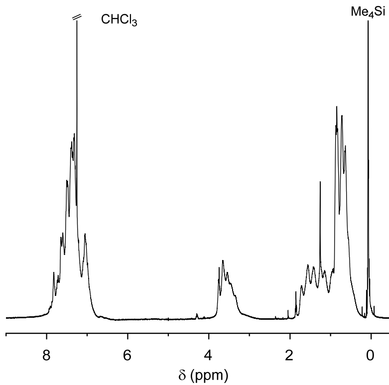
Figure 2-8. ^1\text{H} NMR spectrum of poly(4- ran -5). [400 MHz, \text{CDCl}_3 , r.t.].
