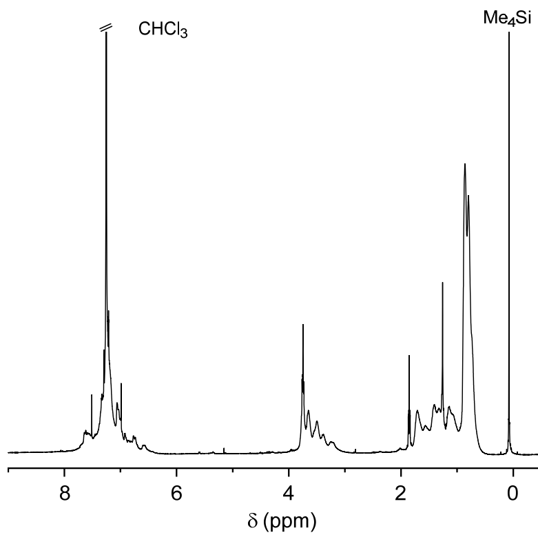
Figure 2-5. ^1\text{H} NMR spectrum of poly(1- ran -5). [400 MHz, \text{CDCl}_3 , r.t.].
