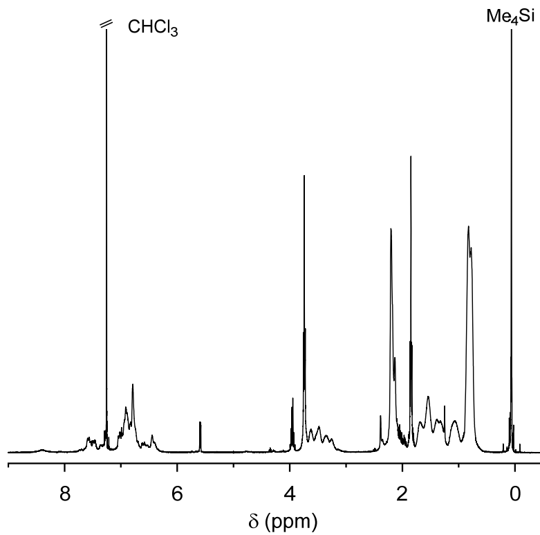
Figure 2-6. ^1\text{H} NMR spectrum of poly(2- ran -5). [400 MHz, \text{CDCl}_3 , r.t.].
