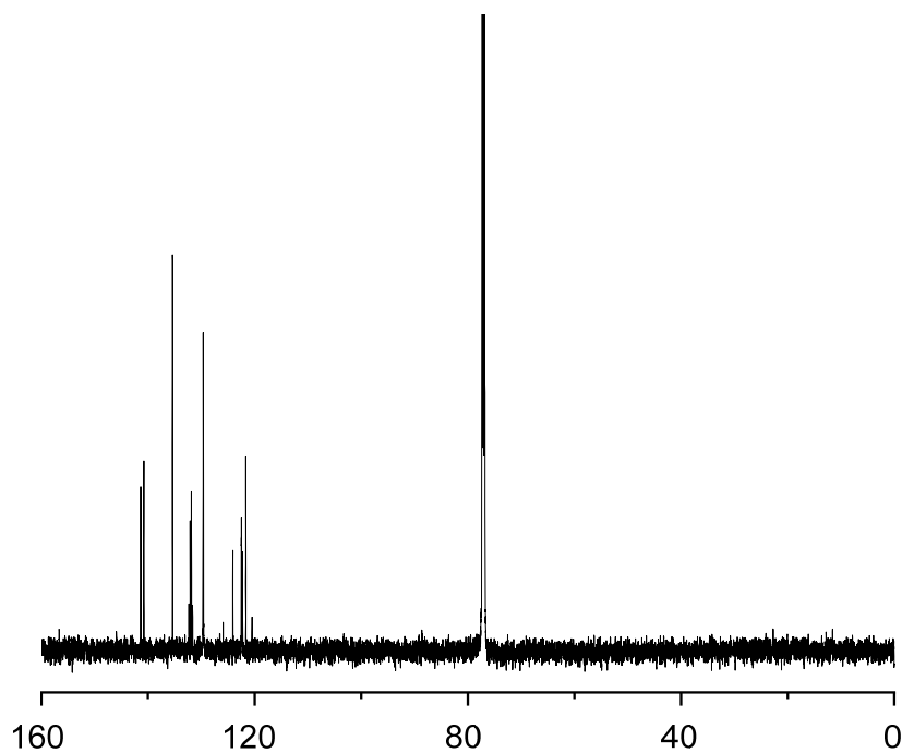
Figure 2-38. ^{13}\text{C} NMR spectrum of 1,4-dibromo-2,5-bis(3,5-bis(trifluoromethyl)phenyl)benzene. [600 MHz, \text{CDCl}_3 , r.t.].
