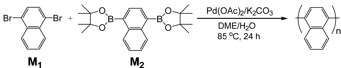
Scheme 3-4. Synthesis of poly(naphthalene-1,4-diyl) by Suzuki-Miyaura cross coupling polymerization using \text{Pd(OAc)}_2 as catalyst in DME.
