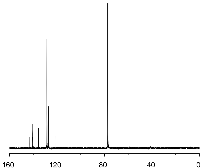
Figure 2-41. ^{13}\text{C} NMR spectrum of 1,4-dibromo-2,5-bis(3,5-diphenylphenyl)benzene. [600 MHz, \text{CDCl}_3 , r.t.].
