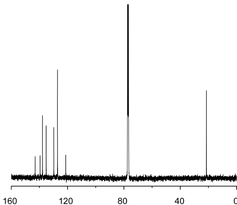
Figure 2-35. ^{13}\text{C} NMR spectrum of 1,4-dibromo-2,5-bis(3,5-dimethylphenyl)benzene. [600 MHz, \text{CDCl}_3 , r.t.].
