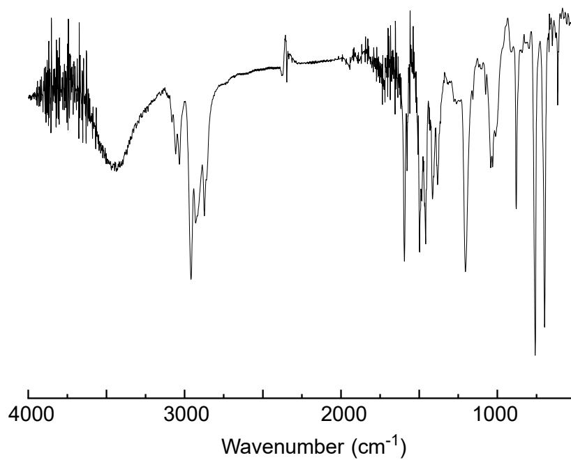
Figure 2-12. IR spectrum of poly(4-alt-6).
