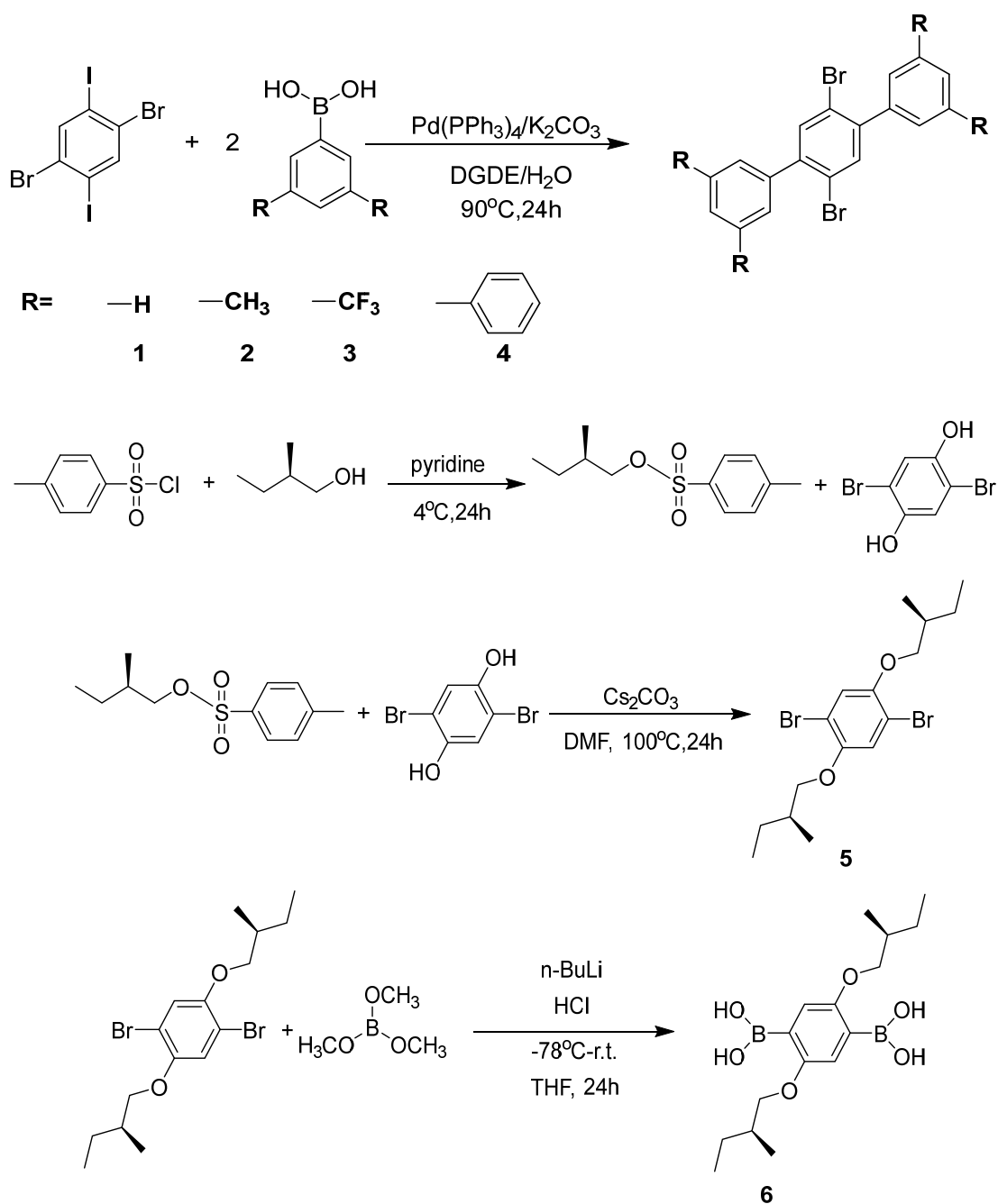
Scheme 2-1. Monomer synthesis.
