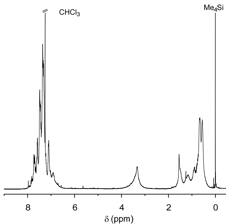
Figure 2-16. ^1\text{H} NMR spectrum of poly(4-alt-6). [400 MHz, \text{CDCl}_3 , r.t.].
