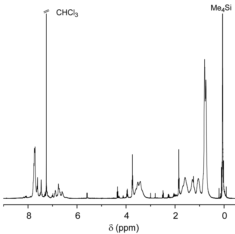
Figure 2-7. ^1\text{H} NMR spectrum of poly(3- ran -5). [400 MHz, \text{CDCl}_3 , r.t.].
