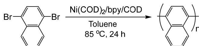
Scheme 3-3. Synthesis of poly(naphthalene-1,4-diyl) by Yamamoto coupling polymerization using \text{Ni(COD)}_2 as catalyst in toluene.
