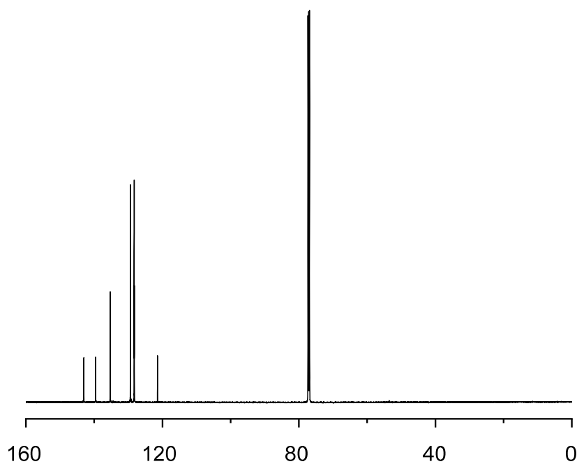
Figure 2-32. ^{13}\text{C} NMR spectrum of 1,4-dibromo-2,5-diphenylbenzene. [600 MHz, \text{CDCl}_3 , r.t.].
