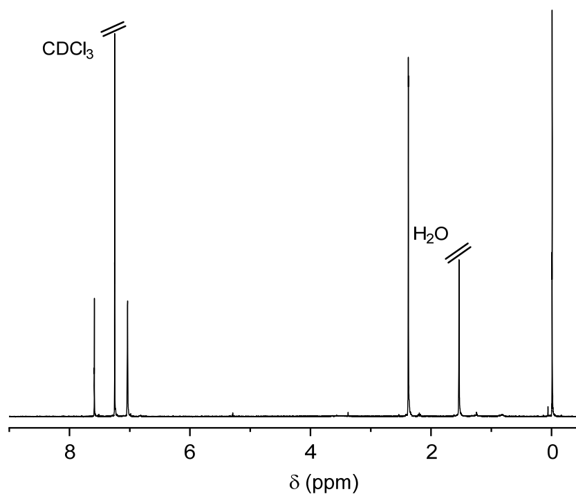
Figure 2-34. ^1\text{H} NMR spectrum of 1,4-dibromo-2,5-bis(3,5-dimethylphenyl)benzene. [400 MHz, \text{CDCl}_3 , r.t.].
