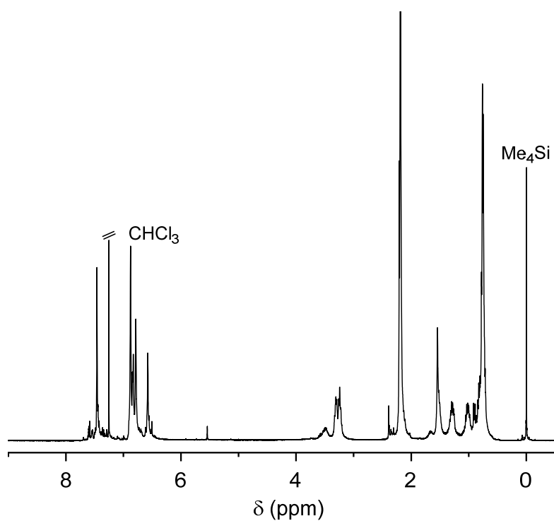
Figure 2-14. ^1\text{H} NMR spectrum of poly(2- alt -6). [400 MHz, \text{CDCl}_3 , r.t.].
