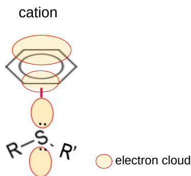
Fig. 7-7 Schematic diagram of lone pair- pi interaction between sulfide and aromatic carbon.
