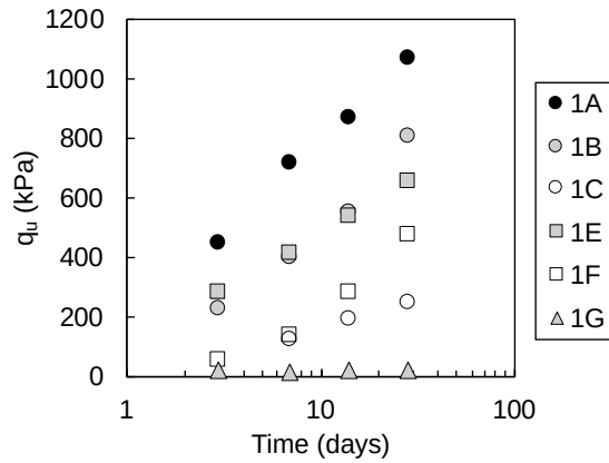
Fig. 3-6 Unconfined compressive strength ( q_u ) values of mixtures 1A, 1B, 1C, 1E, 1F, and 1G with curing time (data for mixtures 1A, 1B, and 1C are from Toda et al. [1]).
