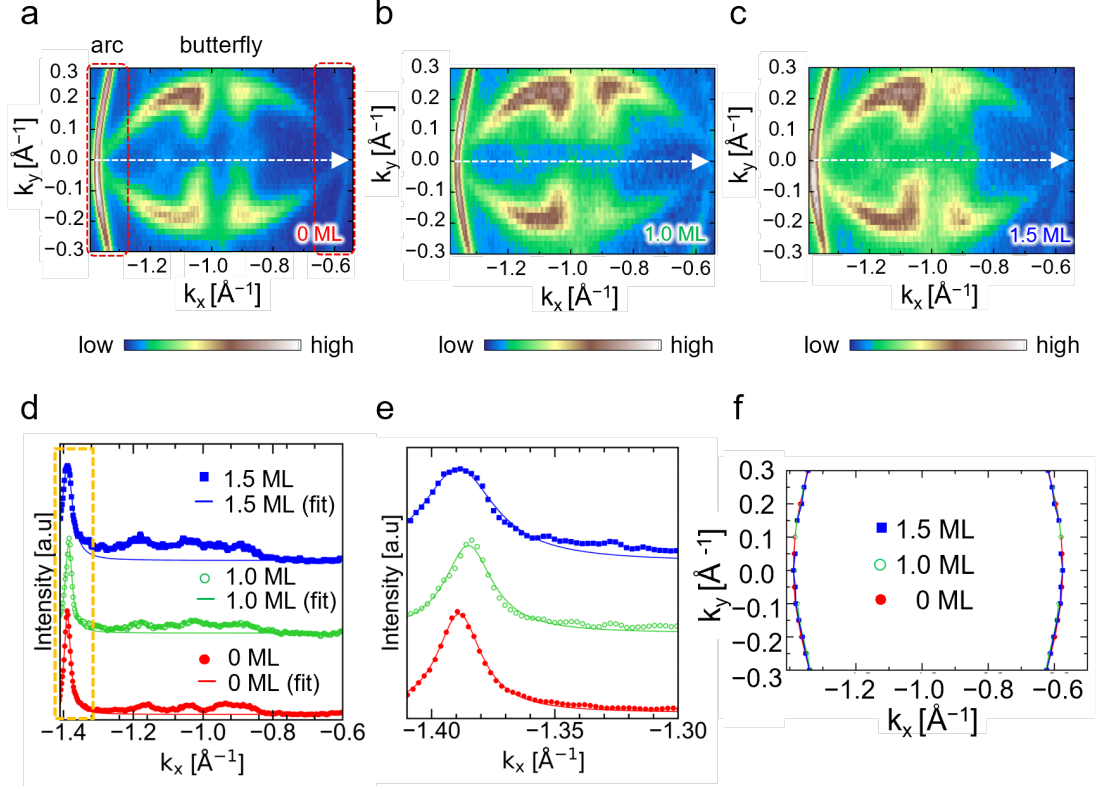
Figure 4.10 ARPES measurements of (\sqrt{7} \times \sqrt{3}) -In before and after adsorption of ZnPc molecules. Photoelectron mapping of the (\sqrt{7} \times \sqrt{3}) -In Fermi surface in momentum space before. (a) and after (b) adsorption of 1.0 \pm 0.3 ML and after adsorption of 1.5 \pm 0.5 ML ZnPc. The region encircled by the dashed red lines indicates an arc-like Fermi surface. (d) MDCs obtained along the white arrow ( k_y = 0 \text{ \AA}^{-1} ) in Fig.4.10(a-c) and peak positions of the arc-like Fermi surface of (\sqrt{7} \times \sqrt{3}) -In (f) acquired for different ZnPc coverages. Solid red circles: 0 ML, open green circles: 1.0 \pm 0.3 ML, solid blue squares: 1.5 \pm 0.5 ML. (e) is the MDC inside the yellow dashed frame in Fig.4.10(d).
