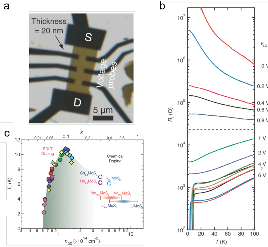
Figure 1.4 (a) Optical micrograph of MoS 2 FET device used for superconductivity measurements. (b) Temperature dependence of resistance of MoS 2 electrical double layer FET modulated by the gate voltage. (c) Dependence of superconducting transition temperature T_c of both electrostatically and chemically doped MoS 2 on carrier density n_{2D} . Fig.1.4 are taken from [36].
