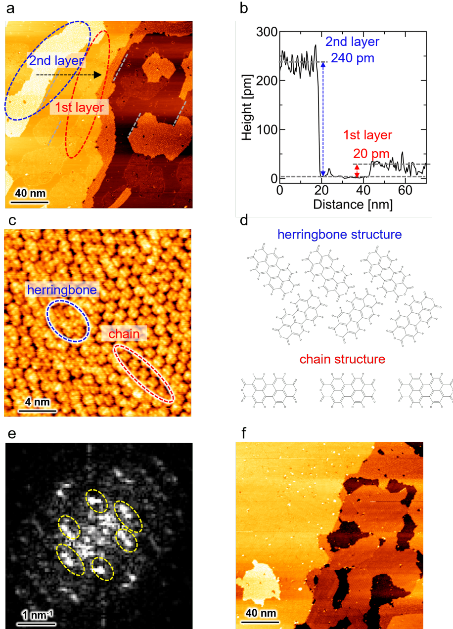
Figure 5.6 PTCDA molecular film structure on (\sqrt{7} \times \sqrt{3}) -In. (a) STM image of PTCDA thin film (0.9 ML) grown on (\sqrt{7} \times \sqrt{3}) -In (200 × 200 nm 2 , V_s = -2.0 V, I_t = 10 pA, T = 4.7 K). The gray dotted line indicates the crystallographic orientation of the substrate. The red and blue dotted circles indicate the first and second layers of PTCDA film. (b) shows the height profile along the black arrow in (a). (c) STM image of PTCDA film structure on (\sqrt{7} \times \sqrt{3}) -In (20 × 20 nm 2 , V_s = -2.0 V, I_t = 10 pA, T = 78 K). The red and blue dotted frame indicate the chain and herringbone structure. (d) PTCDA chain and herringbone structural models. (e) is FFT image of (c) (5 × 5 nm -2 ). The spots within the yellow dotted frame reflect the subtle periodic structure of the film structure. (f) STM image of PTCDA thin film (1.6 ML) grown on (\sqrt{7} \times \sqrt{3}) -In (200 × 200 nm 2 , V_s = -2.0 V, I_t = 10 pA, T = 4.7 K).
