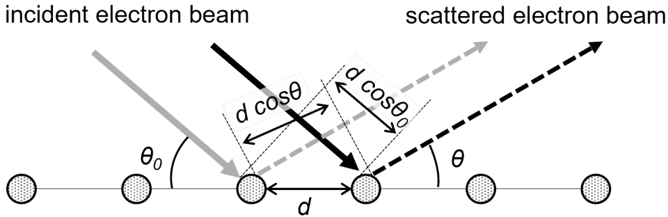
Figure 3.1 Electron diffraction by atoms in one-dimensional array. The incident electron beam come from the incident angle \theta_0 and are reflected to the reflect angle \theta .
