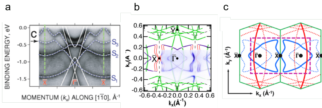
Figure 4.2 Electronic state of ( \sqrt{7} \times \sqrt{3} )-In investigated by ARPES measurements. (a) The band structure of ( \sqrt{7} \times \sqrt{3} )-In [6]. (b) The Fermi Surface of ( \sqrt{7} \times \sqrt{3} )-In [7]. The blue line indicates the experimental data. The other color lines indicate the theoretical calculation results. The Brillouin zone is indicated by black broken lines. (c) The schematic illustration of the Fermi Surface of ( \sqrt{7} \times \sqrt{3} )-In [8].
