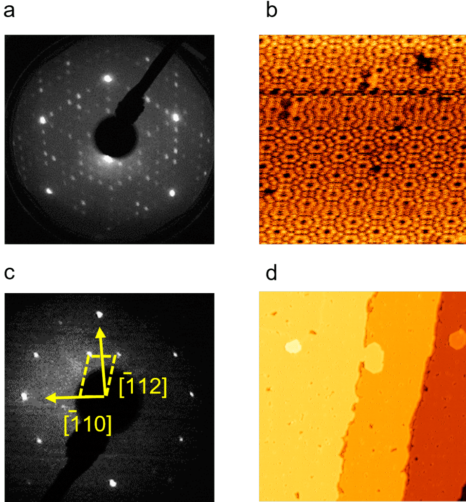
Figure 4.7 Sample preparations for transport measurements. (a) LEED pattern (50 eV) at RT and (b) STM image (image size: 20 \times 20 \text{ nm}^2 , sample voltage: V_s = -1.5 \text{ V} , tunnel current: I_t = 300 \text{ pA} .) at RT of Si(111)- 7 \times 7 . (c) LEED pattern (90 eV) at RT and (d) STM image (image size: 200 \times 200 \text{ nm}^2 , sample voltage: V_s = -1.5 \text{ V} , tunnel current: I_t = 300 \text{ pA} .) at RT of (\sqrt{7} \times \sqrt{3}) -In.
