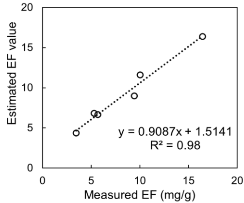
Fig. 3-6 The correlation of PM EF of batch 1, the experiment, and the estimated value based on the pure biochar EF
