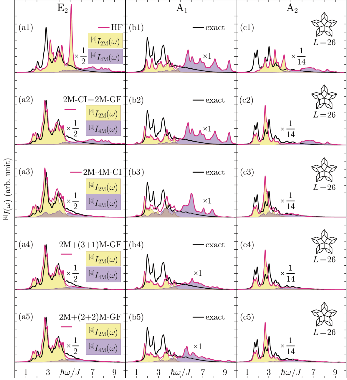
Figure 4.5: The same as Fig. 4.4 for the L = 26 two-dimensional Penrose lattice of \mathbf{C}_{5v} point symmetry.
