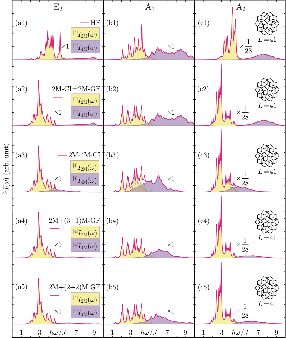
Figure 4.6: The same as Fig. 4.4 for the L = 41 two-dimensional Penrose lattice of \mathbf{C}_{5v} point symmetry without any exact solution available.
