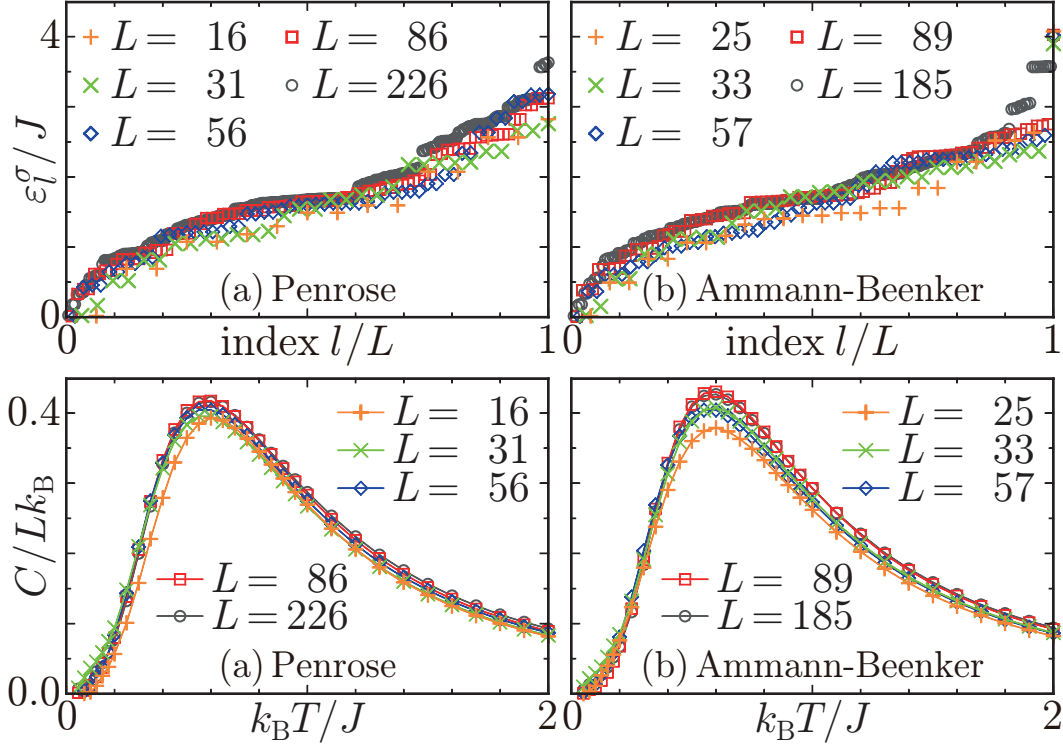
Figure 3.1: The eigenvalues \varepsilon_l^{\sigma} (\sigma = \pm, 1 \leq l \leq L) of the bosonic Hamiltonian (3.20) and quantum Monte Carlo calculations of the specific heat C as a function of temperature T of the antiferromagnetic Heisenberg Hamiltonian (3.1) for various two-dimensional Penrose (a) and Ammann-Beenker (b) clusters of point symmetry \mathbf{C}_{5v} and \mathbf{C}_{8v} , respectively.
