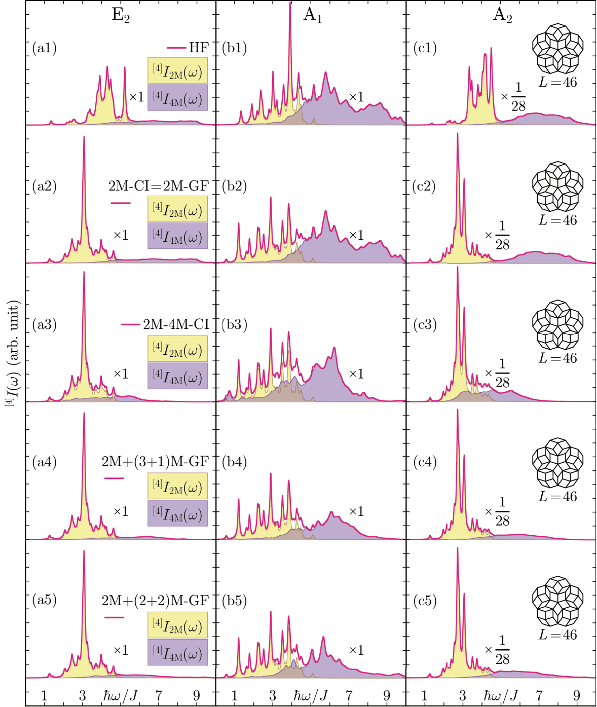
Figure 4.7: The same as Fig. 4.4 for the L = 46 two-dimensional Penrose lattice of \mathbf{C}_{5v} point symmetry without any exact solution available.
