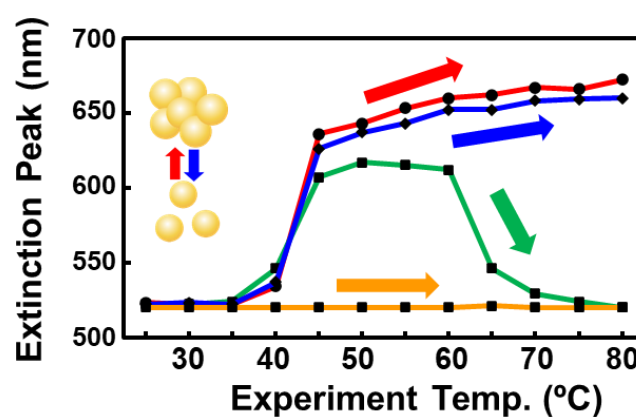
Figure 3-5. Temperature-dependent changes in the extinction peak wavelength of 10 nm AuNPs @ C2-EG6-C11-SH: without free ligands (red), with OH-EG6-C12 addition (blue), with OH-EG6-C11-SH addition (green), removal of free OH-EG6-C12-SH (orange).
