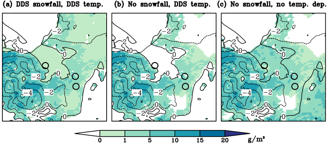
Fig. 2.6. (a) Snow concentration estimated based on the DDS data with the full conditions on temperature and wind shown by shading, superimposed contours describing 2-m temperature ( ^{\circ}\text{C} ), at 0000 UTC on 29 Feb 2016. (b) Snow concentration estimated without the snowfall effect in Eq. (2.1). (c) Snow concentration estimated without the snowfall effect in Eq. (2.1) and further without the temperature dependencies.
