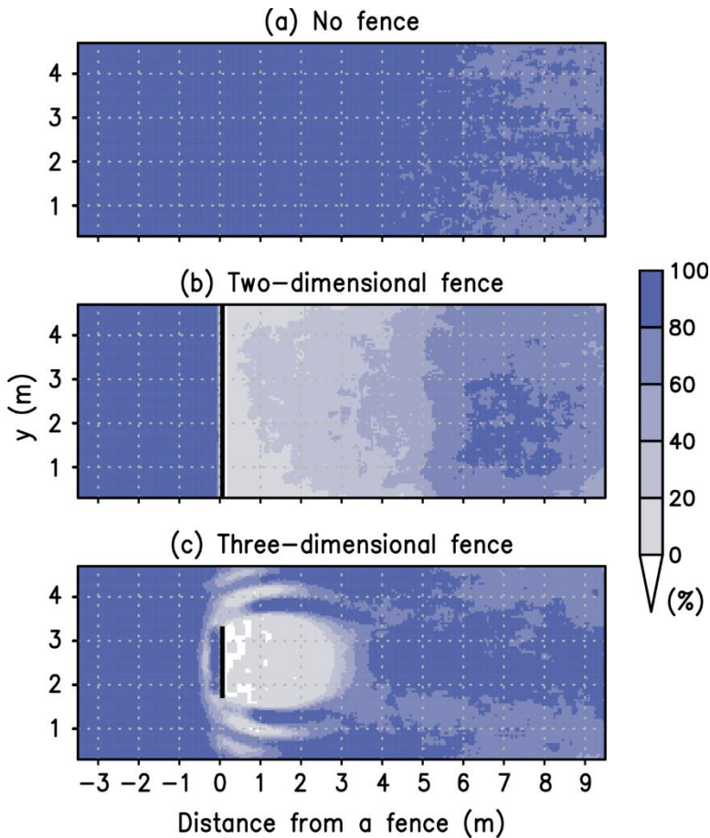
Fig. 3.13. Snowdrift potential (a) for no fence, (b) around the two-dimensional fence, and (c) around the three-dimensional fence. The position of the fence is shown by a solid line.
