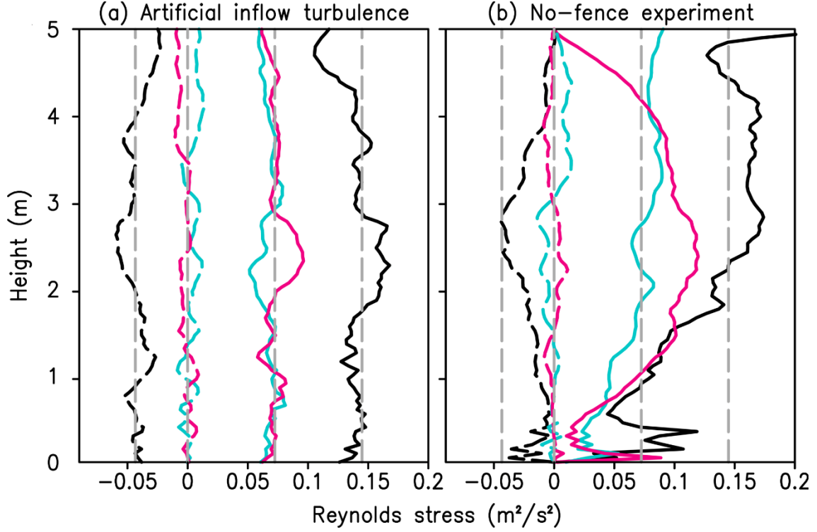
Fig. 3.5. Vertical profile of six components of Reynolds stress (a) in the artificial inflow turbulence at the center of the y -axis and (b) in the no-fence experiment at (x, y) = (3.5 \text{ m}, 2.5 \text{ m}) . Solid lines are \langle u'u' \rangle (black), \langle v'v' \rangle (blue), and \langle w'w' \rangle (pink). Broken lines are \langle u'w' \rangle (black), \langle u'v' \rangle (blue), and \langle v'w' \rangle (pink). The grey dotted line indicates the target values of \langle u'w' \rangle , \langle u'v' \rangle and \langle v'w' \rangle , \langle v'v' \rangle and \langle w'w' \rangle , and \langle u'u' \rangle from left to right.
