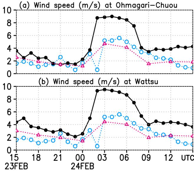
Fig. 2.5. Time-series of surface wind speed (a) at Ohmagari-Chuou, 141.47°E, 42.98°N and (b) at Wattsu, 141.50° E, 42.96°N, from 1500 UTC 23 Feb 2016 to 1500 UTC 24 Feb. It is remarked that the model outputs are at 10 m above the ground level (AGL) while the anemometer is installed at 15 m AGL at Ohmagari-Chuou and at 5 m AGL at Wattsu. A black line with filled circles indicates the results of DDS at the nearest gridpoint, a pink line with triangles indicates MSM analysis, a blue line with open circles indicates AMeDAS observation.
