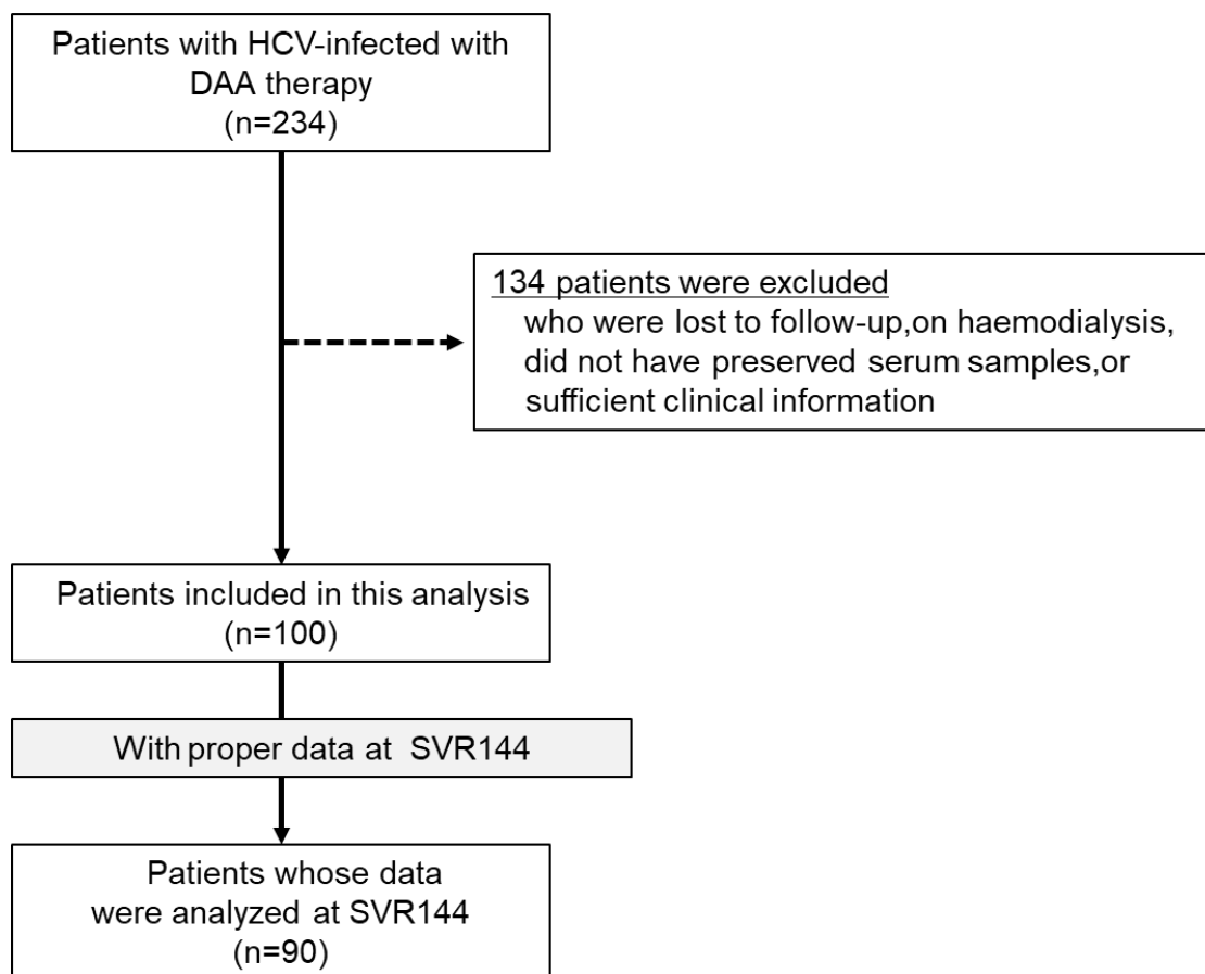
Figure 1. Study flow
