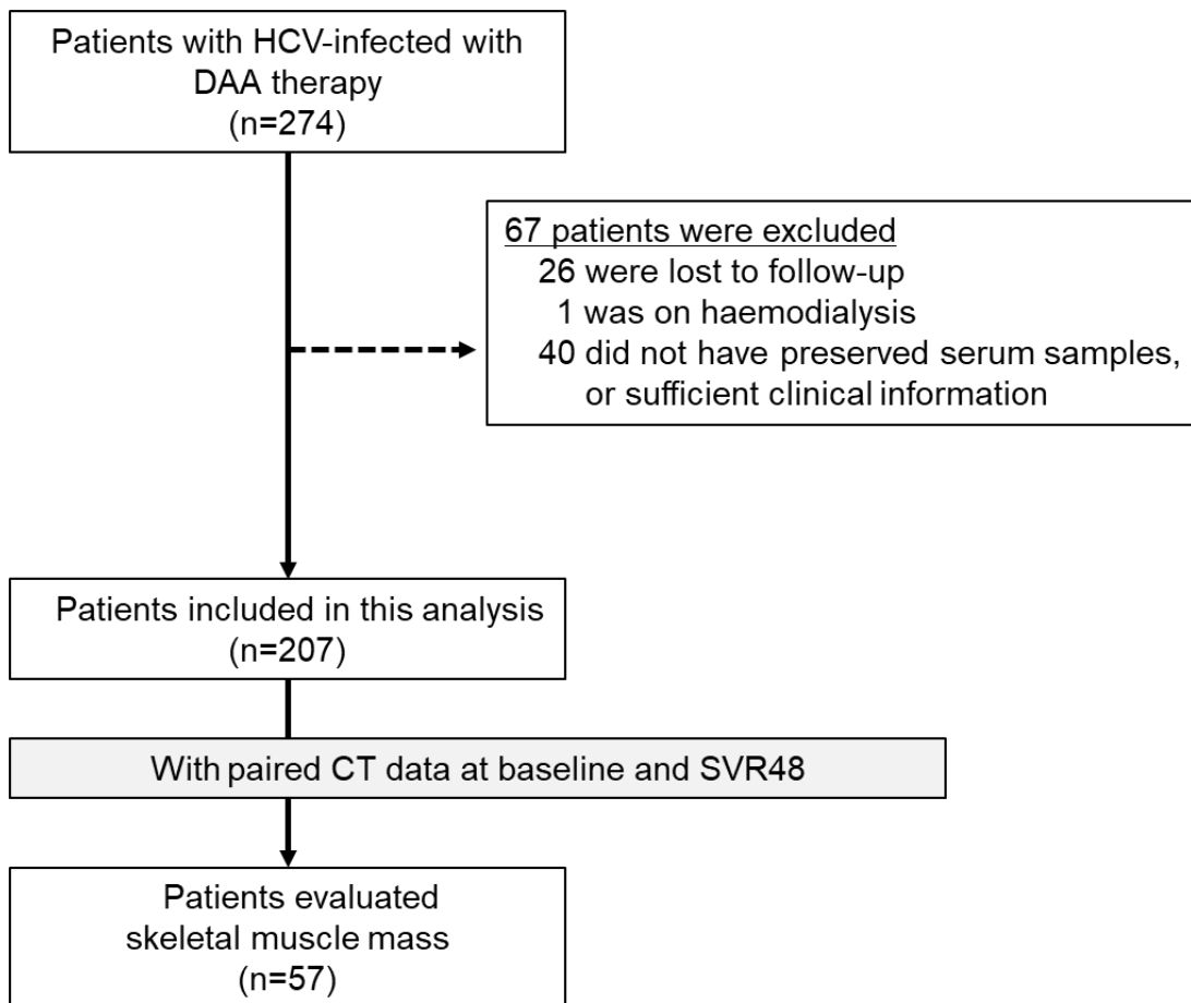
Figure 2. Study flow
