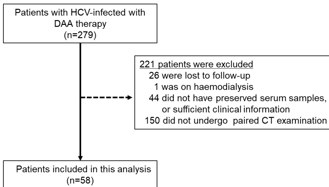
Figure 1. Study flow
