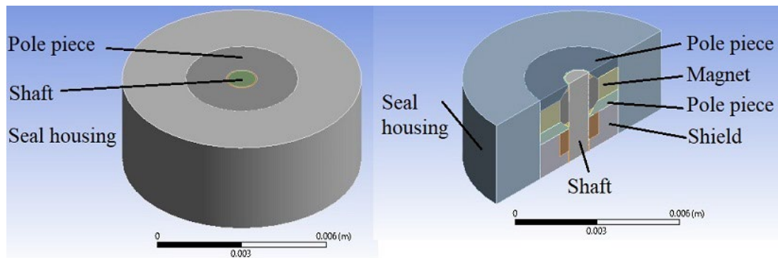
Figure 5 Basic model of an MF seal.
