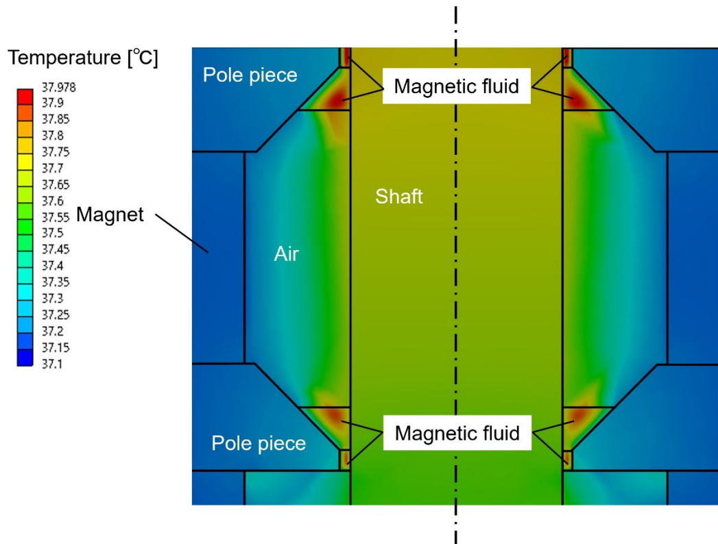
Figure 10 Temperature distribution in MF of a basic MF seal model.
