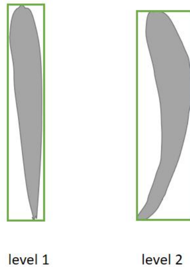
Fig. 3.7 Two specifications divided with convex polygon.
