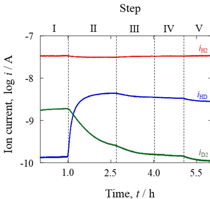
Figure 2.2 Transient behavior of the ion currents ( i_{\text{H}_2} red, i_{\text{HD}} blue, i_{\text{D}_2} green) of the hydrogen gas in each experimental step in Table 2.1. (For interpretation of the references to color/colour in this figure legend, the reader is referred to the Web version of this article.)
